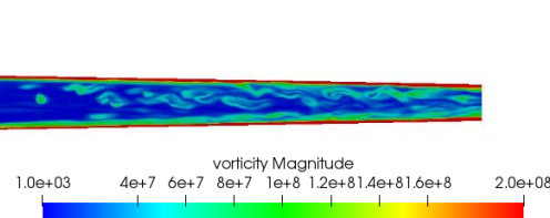
Figure 4-15 Cross-sectional view of the instantaneous vorticity field along the nozzle length and at the nozzle exit.
