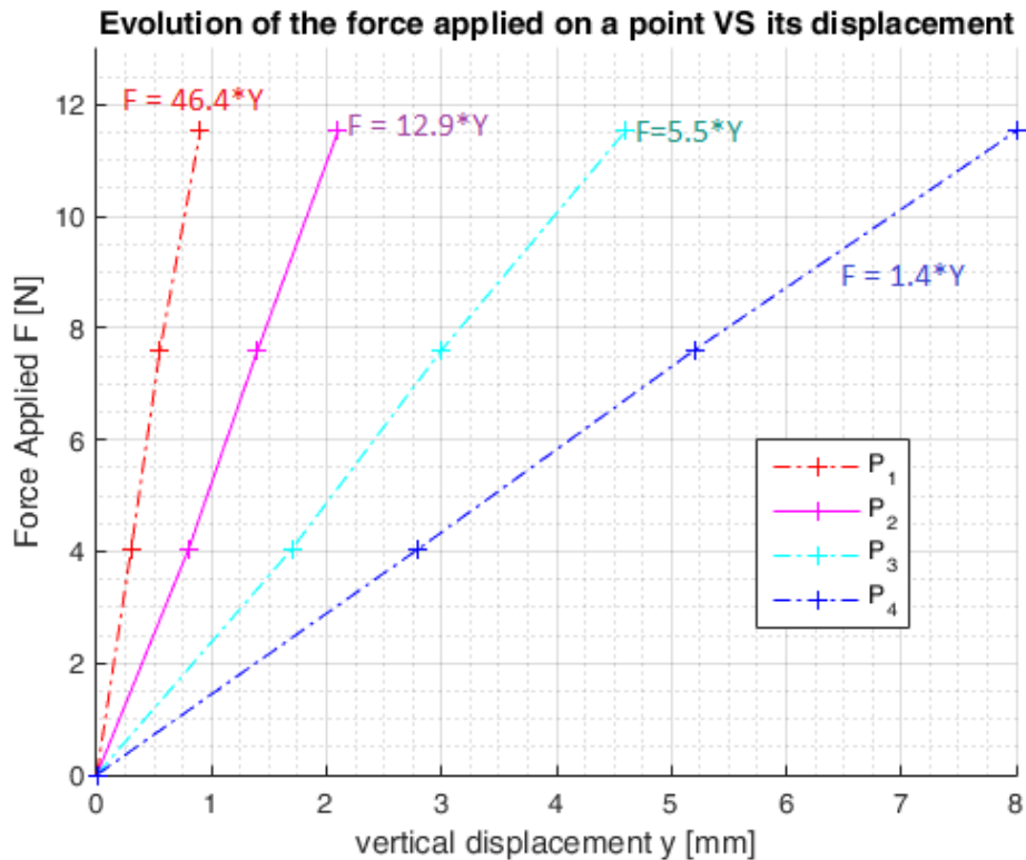
FIGURE 2.23 – Evolution of the force versus the displacement on a point, 3D-printed carbon foil
