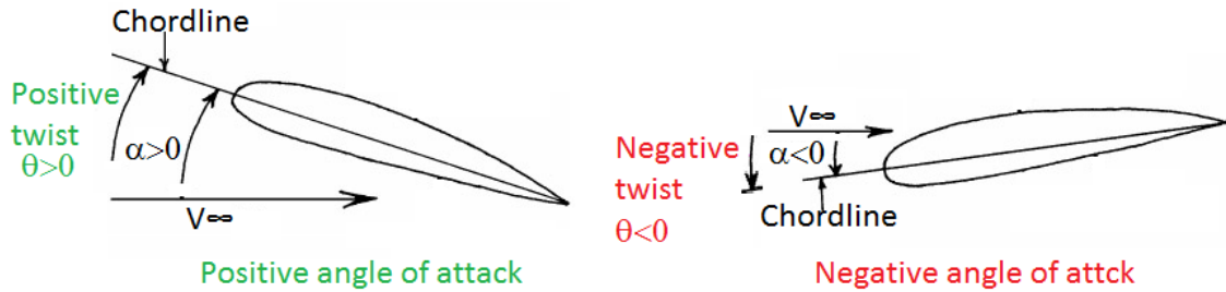
FIGURE 4.30 – sign convention for the angle of attack on a profile
