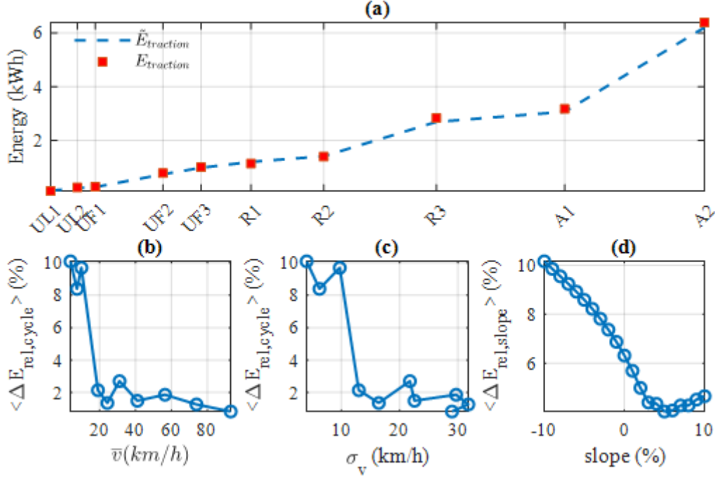
Figure 48. Energy estimator assessment for the 10 INRETS driving cycles : (a) E_{\text{traction}} (squares) and \tilde{E}_{\text{traction}} (dotted lines) versus cycle, (b) \langle \Delta E_{rel,cycle} \rangle versus \bar{v} , (c) \langle \Delta E_{rel,cycle} \rangle versus \sigma_v , (d) \langle \Delta E_{rel,slope} \rangle versus slope.
