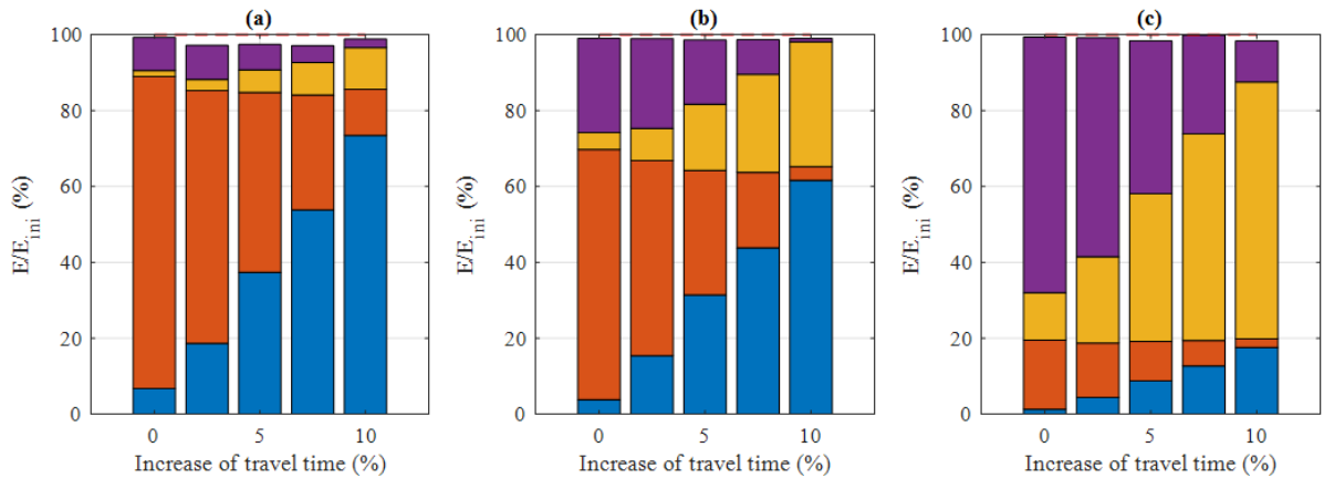
Figure 65. Repartition of estimated and realized energy for T_{ext,0} = 38\text{ }^{\circ}\text{C} , RH_{ext,0} = 55\% , P_{sun,0} = 1000\text{ W} and the following driving cycles: (a) INRETS A2, (b) INRETS R2, (c) INRETS UL1
