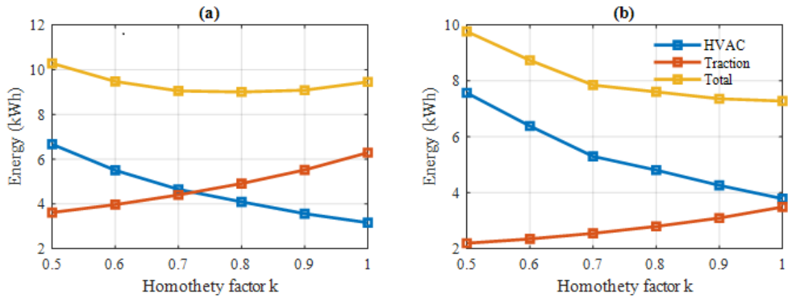
Figure 38. Traction, air conditioning and total energy consumed for a driver dressed in an informal way, for T_{ext} = 36^\circ C , RH_{ext} = 50\% \dot{q}_{sun} = 1000 W/m^2 , and: (a) INRETS R2, (b) INRETS UF3 driving cycle
