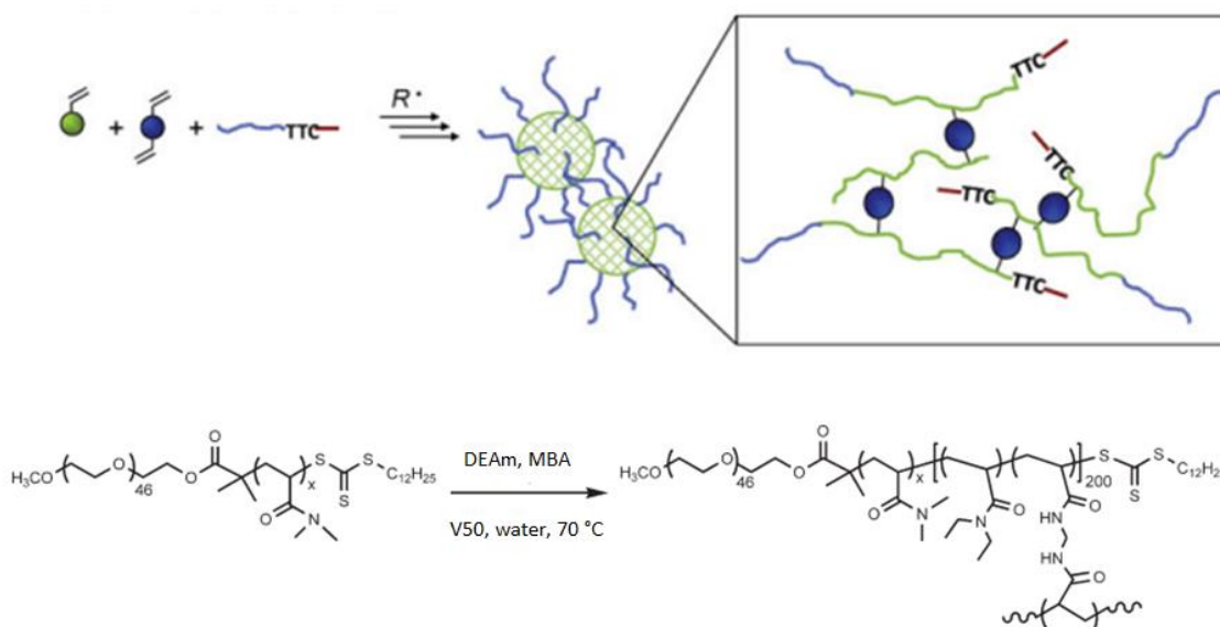
Figure I.40. Synthesis of LCST-type thermosensitive nanogels by RAFT-PITSA of DEAm in water and at 70°C in presence of PEO- b -PDMAm macro-CTA containing trithiocarbonate group (TTC).Reproduced from ref. 159
