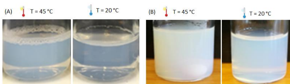
Figure III.9. Pictures of (A) Thermal-PPEGA 30 - b -Thermal-P(NIPAm 188 - co -MBA 7 ) nanogel aqueous solution and (B) UV-PPEGA 30 - b -UV-P(NIPAm 175 - co -MBA 6 ) nanogel aqueous solution at a concentration of 5 g.L -1 at 20°C and 45 °C.
