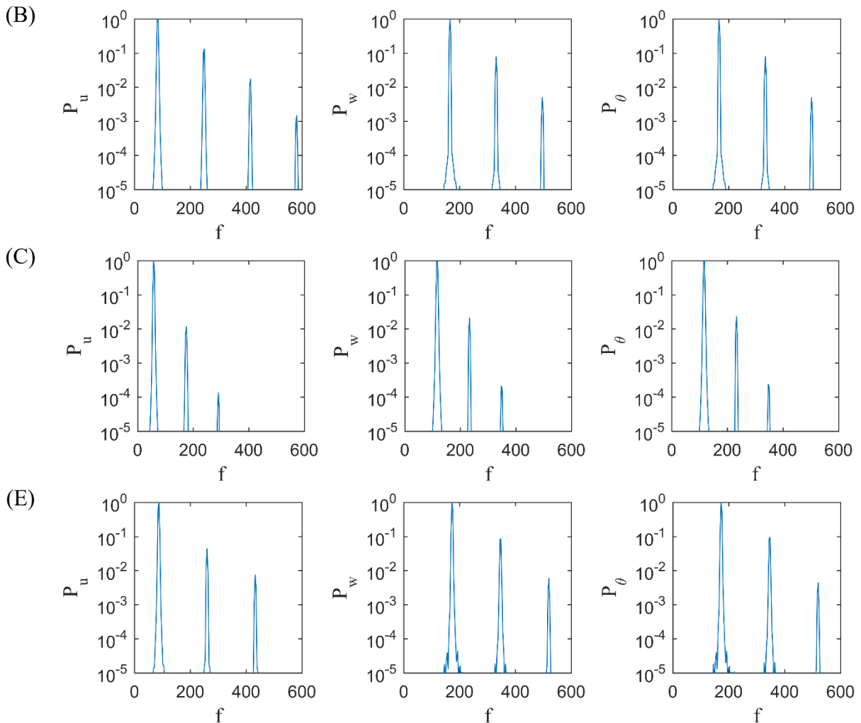
Figure 4.20. Ra = 1.2 \times 10^7 . Density power spectra of u , w and \theta at the point B_1 for the different configurations.
