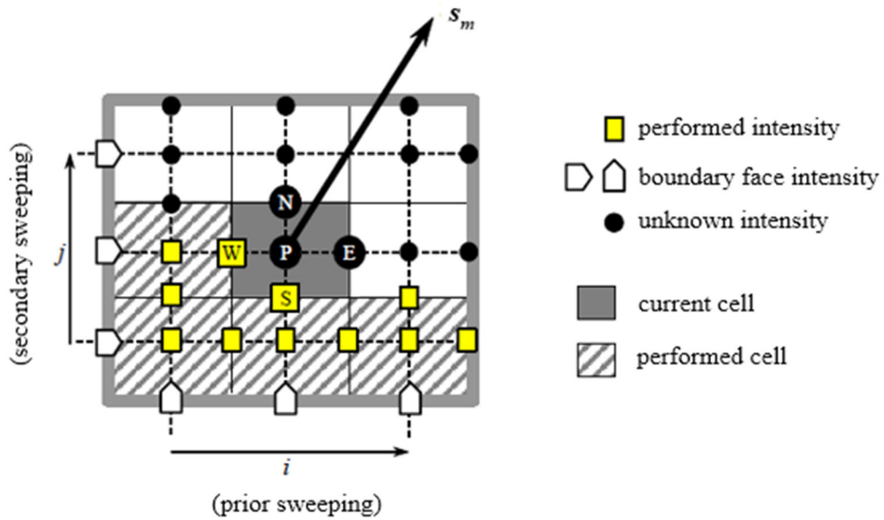
Figure 2.4. Resolution of the RTE by sweeping the computation domain. (From Denis Lemonnier course on radiation phenomena-ISAIE-ENSMA).
