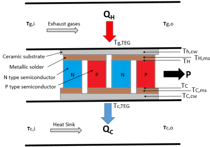
Figure 4. Thermal modeling of TEG.
