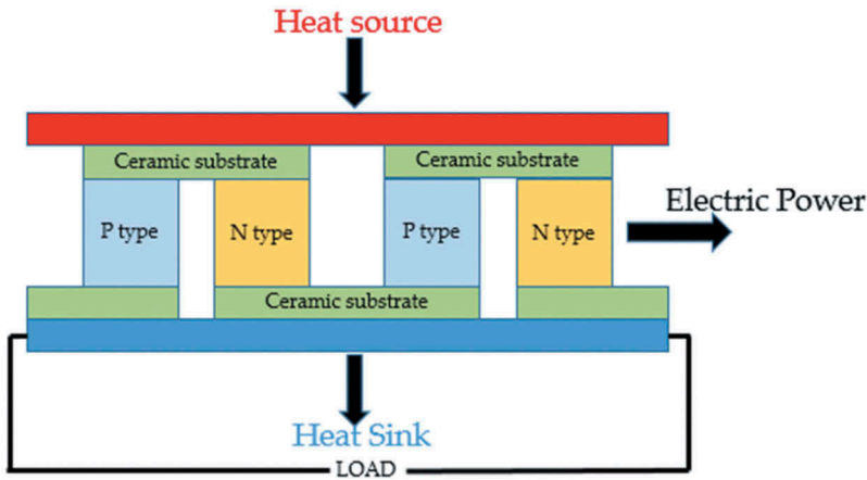
Figure 2. Thermoelectric generator.
