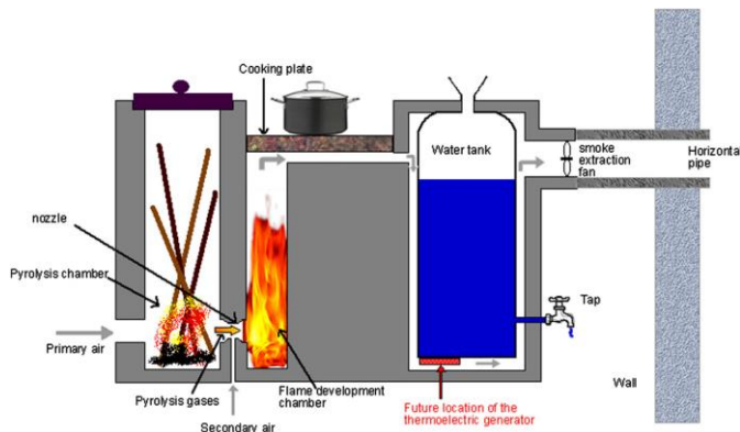
Figure 10. Multifunction wood stove [37].
