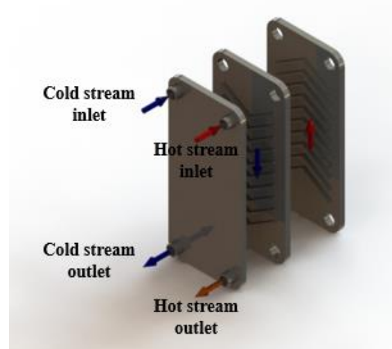
Fig. 10. Plate heat exchanger.
