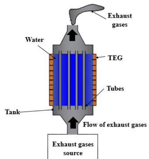
Figure 1. Domestic thermoelectric cogeneration heat recovery system.
