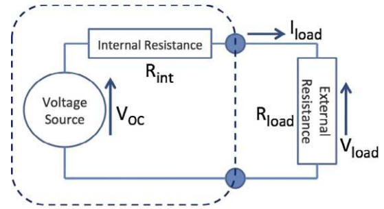
Thermoelectric Generator
