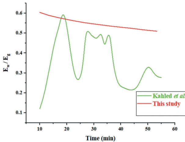
Figure 10. Energy fraction for both studies over time.
