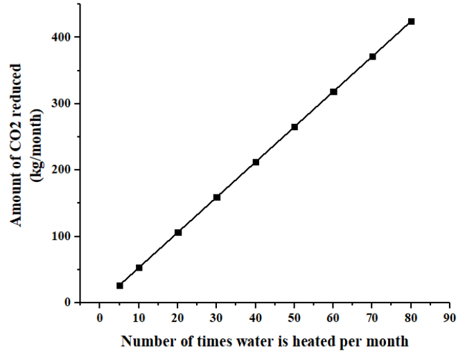
Figure 16. Amount of CO 2 gas reduced by the heat recovery system.
