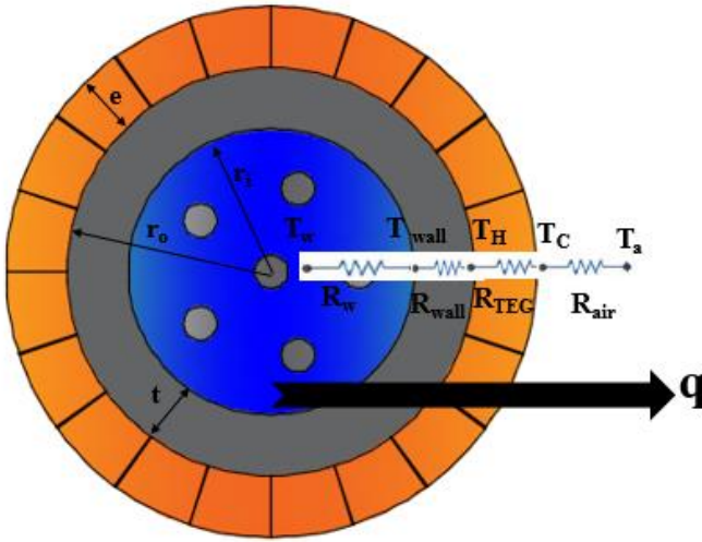
Figure 3. Thermal resistance modelling schematic of the system
