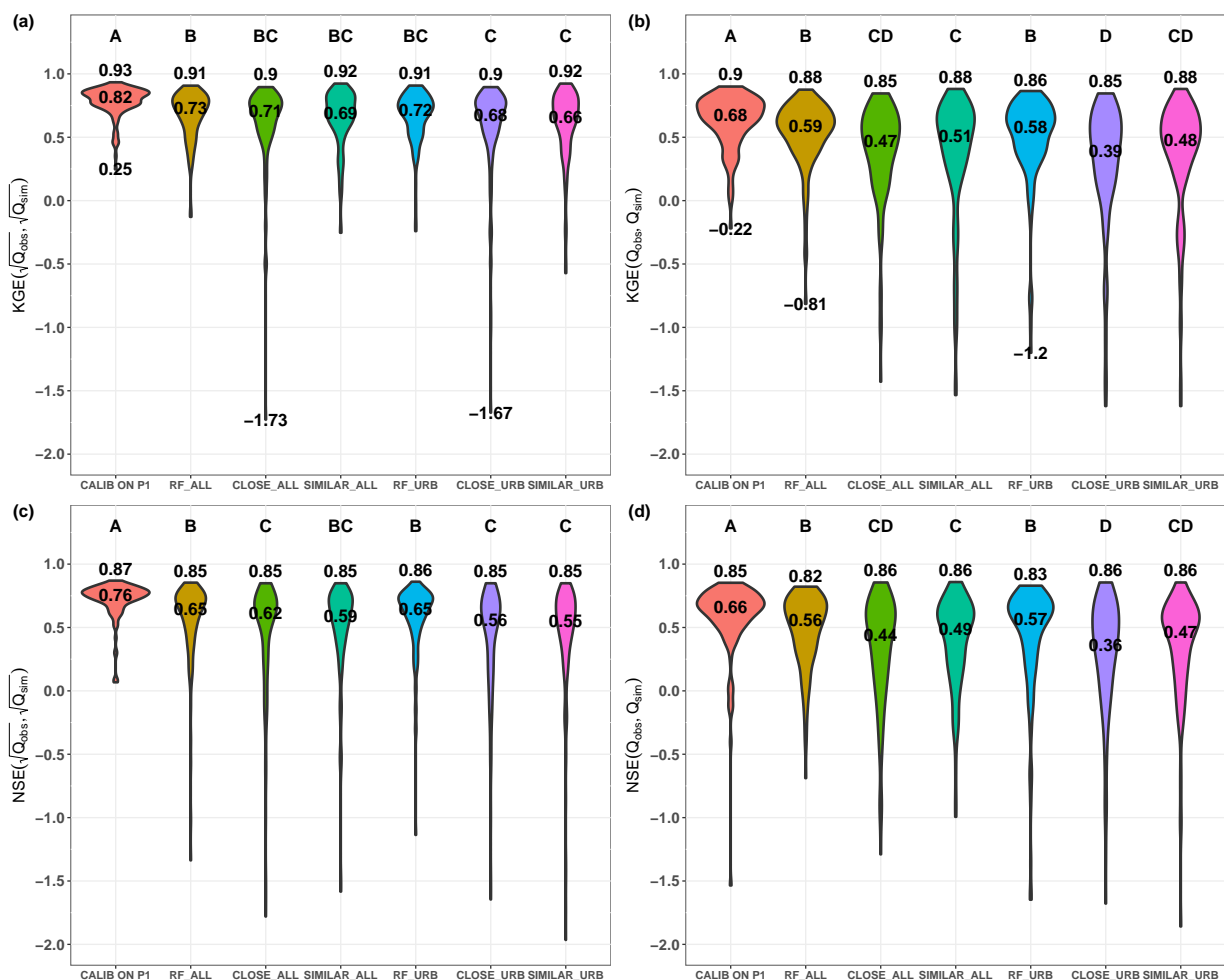
Figure 5.5. Validation scores on P2 in terms of (a) KGESR (b) Kling-Gupta efficiency (KGE) (c) NSESR and (d) Nash-Sutcliffe efficiency (NSE) using calibrated parameters on P1 (CALIB ON P1), estimated parameters using random forest (RF_ALL and RF_URB), transferred parameters from the closest catchments (CLOSE_ALL and CLOSE_URB) and from the most similar catchments (SIMILAR_ALL and SIMILAR_URB). The values indicate the minimum, the median, and the maximum scores. Some minimum values were not shown as they were less than -2.0 for the considered metric of evaluation. The letters indicate the statistical equality at 10% risk between the performances, estimated using the Mann-Whitney-Wilcoxon test.
