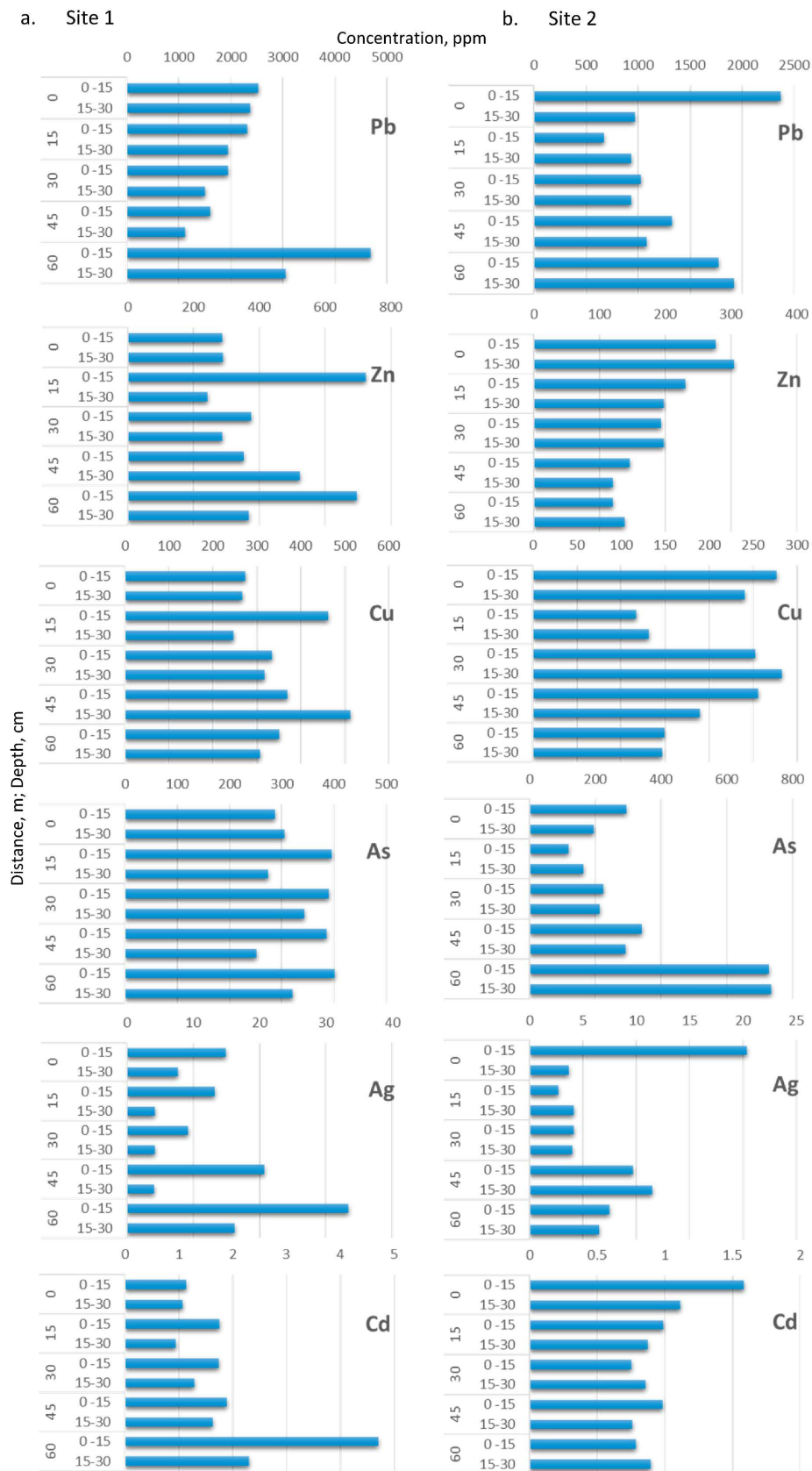
Figure 2. Soil Pb, Zn, As, Cu, Ag, and Cd concentration (mg kg -1 ) for five distances (0–60 m) and two depths (0–15 and 15–30 cm) in site#1 and site #2 from Hualgayoc district, Cajamarca region, Peru.
