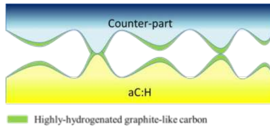
Fig. 1 Schematic image of superlubricity in a vacuum.
