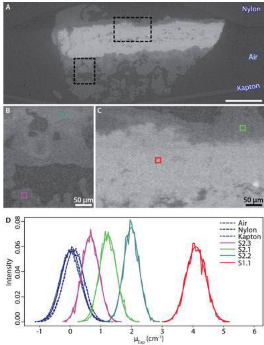
Figure 4.5: Measurement of attenuation coefficients \mu_{Exp} from selected zones in sample AO 14506-1b. A, Tomographic slice showing zones where attenuation coefficients were measured. Scale bar: 500 \mu\text{m} . B and C, Close-up of the left and right dotted boxes in A. Scale bar in B and C: 50 \mu\text{m} . D, Distribution of calibrated \mu_{Exp} of each selected zone fitted by Gaussian distributions. I_{GV} values were sampled at the locations indicated by a square of 5 \times 5 voxels through 101 successive slices in the reconstructed data volume (2,525 voxels in total).
