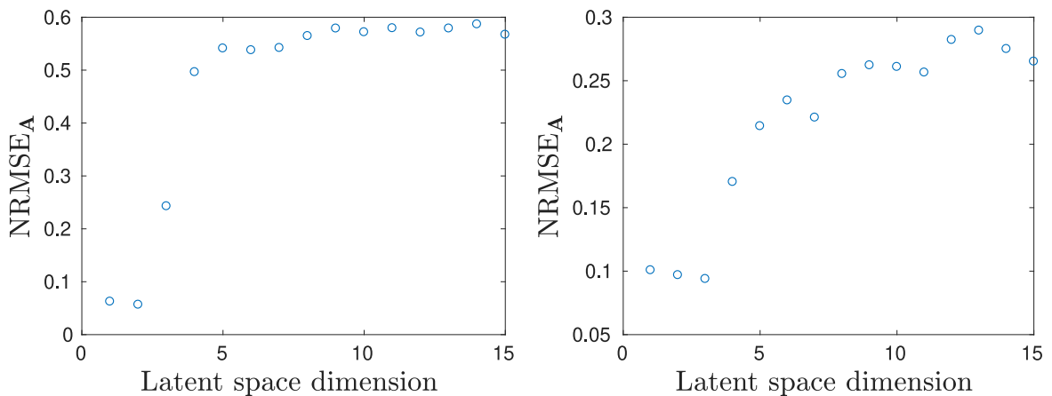
Figure 35 – Abundance NRMSE as a function of the latent space dimension H for datacubes DC1 (left) and DC2 (right).
