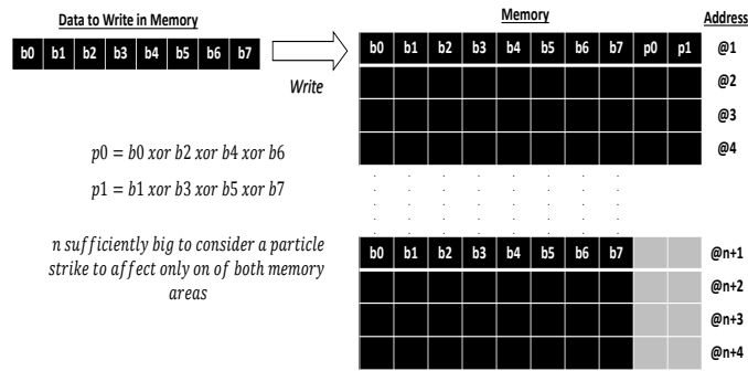
FIGURE 3.1: DPSR Write for 8 bits word
