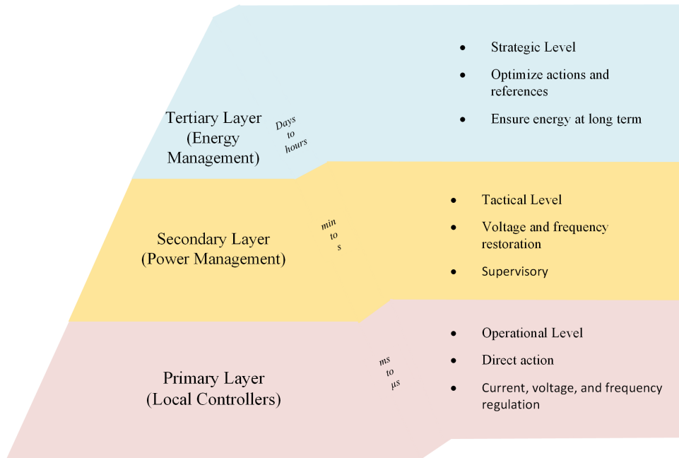
FIGURE 12: MG hierarchical management and control.
