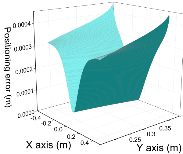
Figure 2.21: Positioning error in the regular dexterous workspace when using leg-direction-based visual servoing ( 30^\circ \sim 150^\circ , \pm 1 pixel)
