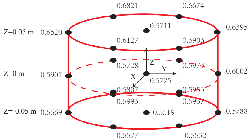
Figure 4.30: Co-simulation positioning errors of the test points using line-based visual servoing (observing 2 legs {1,3}). Measures are in mm
