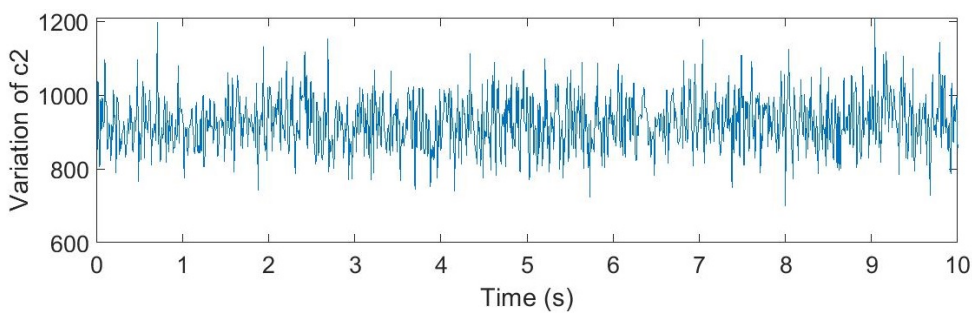
Figure 5.33: Variation of the image moment c_2 for the regular triangle
