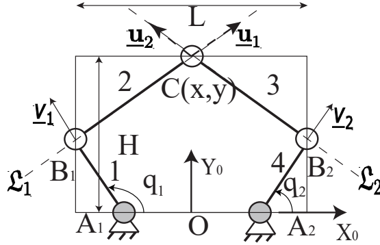
Figure 2.1: Five-bar mechanism
