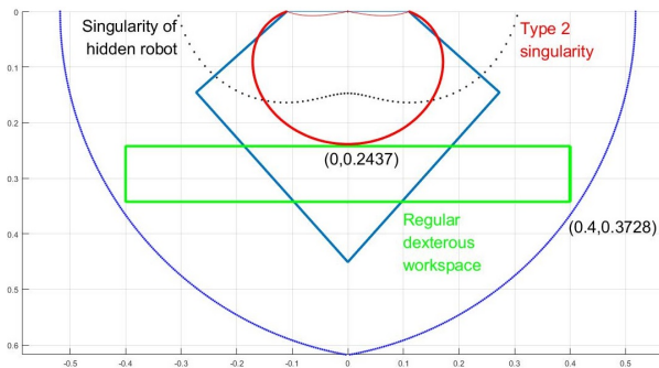
Figure 2.13: Regular dexterous workspace of the optimized Five-bar mechanism using leg-direction-based visual servoing ( 30^\circ \sim 150^\circ , \pm 1 pixel)
