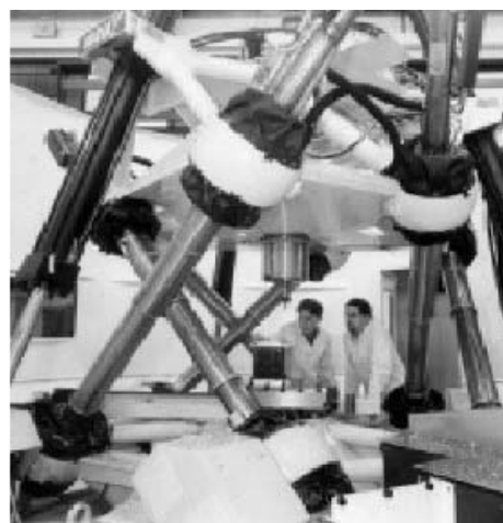
Figure 1.8: The Variax of Giddings and Lewis, the first industrial parallel milling machine presented in 1994 at IMTS [Merlet 2006]
