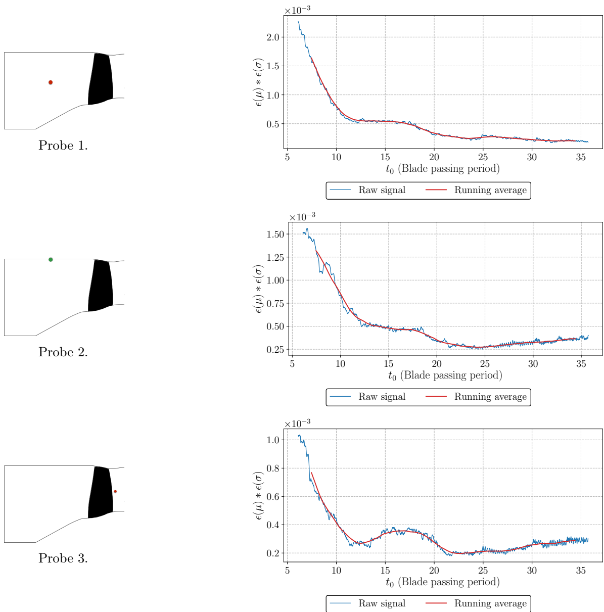
Figure C.2: Evolution of the product of the mean and standard deviation of the probe pressure signals following Mockett's methodology.
