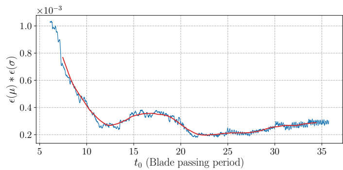
Figure C.2: Evolution of the product of the mean and standard deviation of the probe pressure signals following Mockett's methodology.
