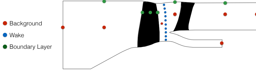
Figure 2.26: Probe locations.
