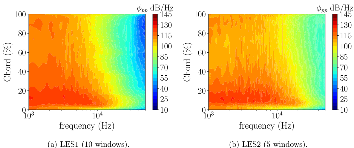
Figure 4.24: PSD of the pressure fluctuations on the rotor surface at 75% fan span.
