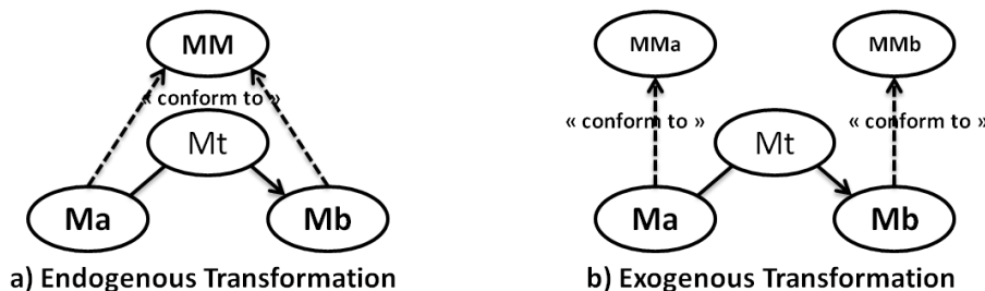
Figure 3.4: The Types of Model Transformation
