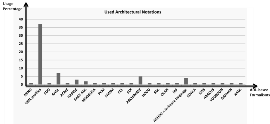
Figure 4.1: Some ADL notations
