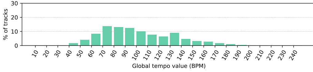
Figure 3.1: ACM tempo distribution.
