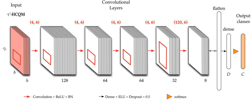
Figure 4.6: DR model Architecture with \tau' - HCQM as input (of size (\phi, b, h) ), the size of convolutional filters is indicated in red (filter_height, filter_width), the number of kernel is indicated in black under each convolutional layer, D denotes the number of units in the dense layer while C is the number of units in the output layer (i.e. the classes logits).
