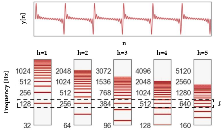
Figure 4.2: Computation of the CQT s of a harmonic signal according to the harmonic series h . The fundamental frequency is bordered by the black dotted rectangle. Figure taken from Bittner's PhD Thesis.
