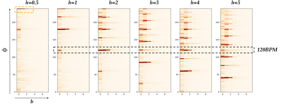
Figure 4.5: HCQM example for a given temporal frame \tau' of a techno track excerpt. \phi denotes the modulation frequency (associated with a candidate tempo), b the acoustic frequency band and h the harmonic coefficient. The tempo is visually identifiable at 120BPM by superimposing its rhythmic harmonic components through h . For h = 0.5 , the tempo is detected at its sub-harmonic (orange dotted lines) that corresponds to the value 240BPM.
