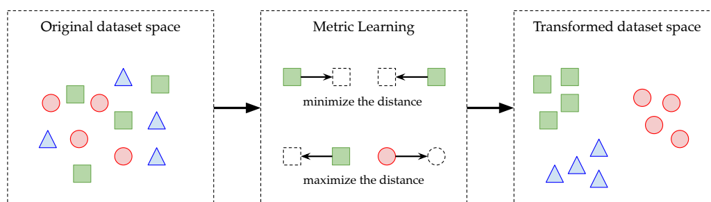
Figure 6.1: Metric learning principle.
