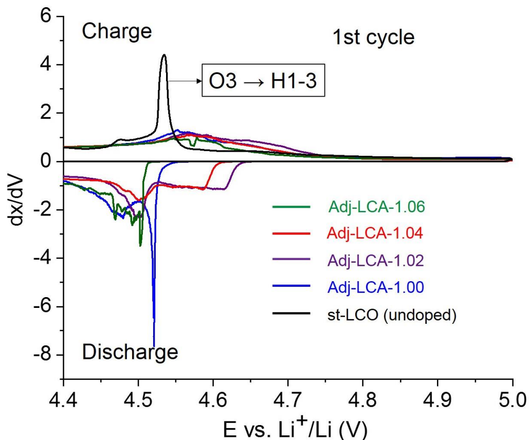
Figure C39. 1 st cycle [4.4 – 5.0 V] dx/dV curves for Group A Adj-LCA-X samples as compared to undoped st-LCO.
