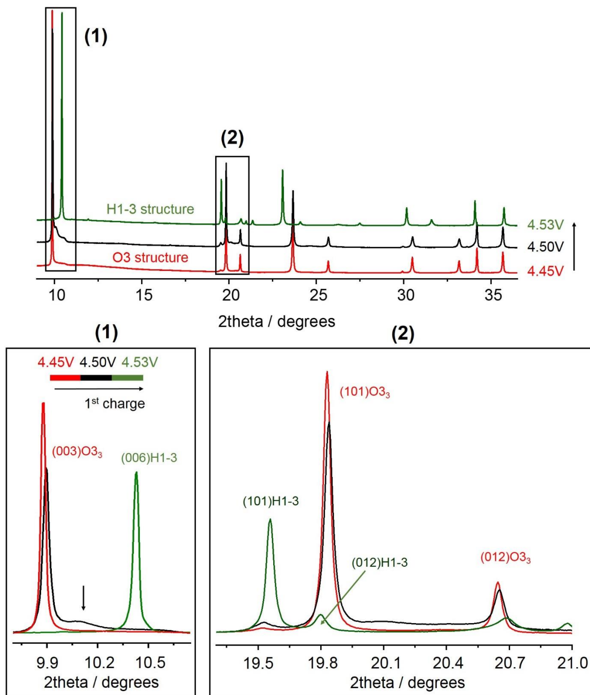
Figure B19. Ex situ SXRD pattern recorded for various \text{Li}_x\text{CoO}_2 powders prepared from electrochemical Li de-intercalation of st-LCO charged up to either E = 4.45\text{ V} , E = 4.50\text{ V} or E = 4.53\text{ V} . Zooms focusing on the (00 \beta ), (101) and (012) diffraction lines are also given.
