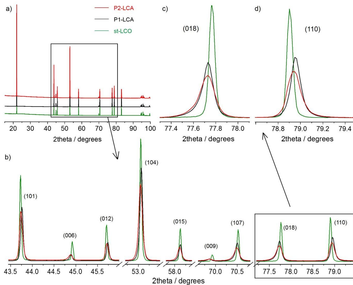
Figure C8. a) Synchrotron X-ray diffraction (SXRD) patterns obtained for P1- and P2-LCA, as compared to undoped LiCoO 2 (st-LCO). All patterns were collected for \lambda = 0.826 \text{ \AA} , but are converted here to \lambda(\text{CoK}\alpha_1) = 1.790 \text{ \AA} for better comparison with all XRD patterns showed in Figure C7. Zooms on several lines is shown in b) and a larger zoom in (0 1 8) and (1 1 0) peaks is provided in c) and d) .
