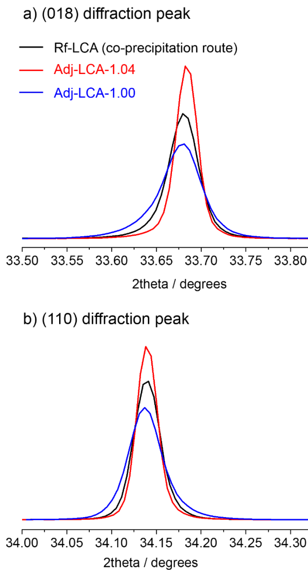
Figure C26. Comparison of a) (018) and b) (110) diffraction peak shapes for two samples prepared from solid state reaction (Adj-LCA-1.00 and Adj-LCA-1.04) vs. a sample prepared from a co-precipitation route.
