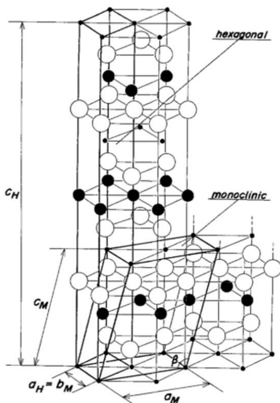
Figure B16. Schematic representation of the structural relationship between the hexagonal and monoclinic settings in describing \text{LiMO}_2 (from Ohzuku and Ueda 27 ). All formulas used to convert the cell parameters from one setting to another in Table B.T5 are given on the right of the figure.
