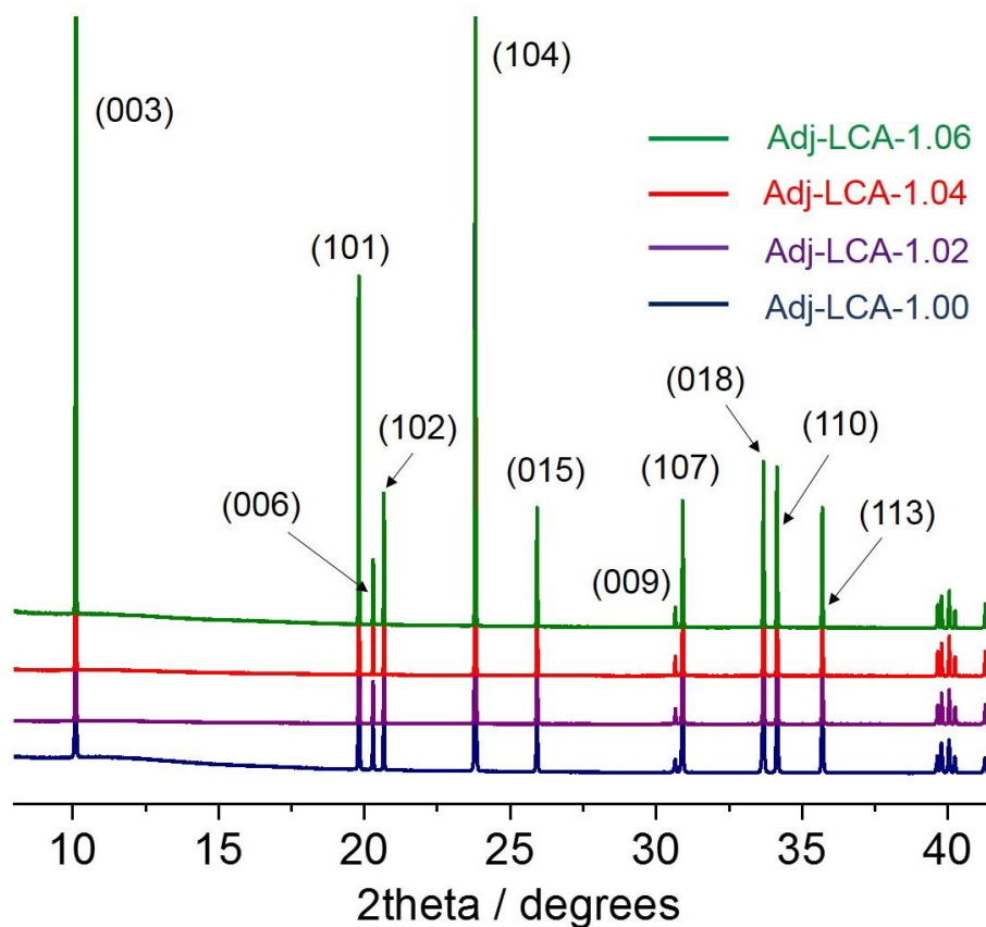
Figure C24. Synchrotron X-ray diffraction (SXRD) patterns obtained for all Li-adjusted LCA from Group A. All patterns were collected for \lambda = 0.826 \text{ \AA} . Miller indexes for the main peaks are also given.
