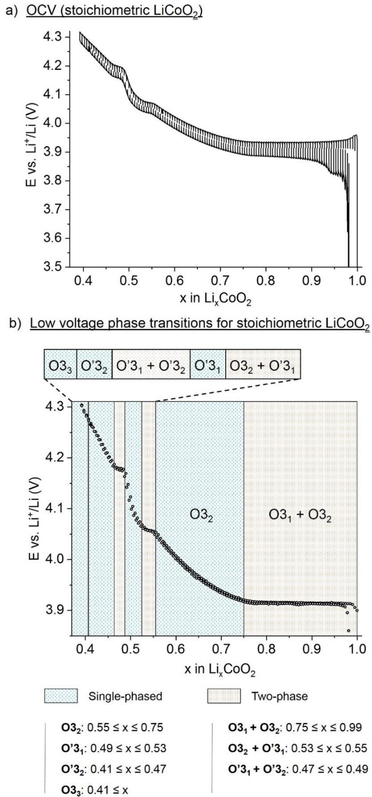
Figure B17. a) Transient voltage profile of st-LCO vs. Li content obtained from GITT and b) reported equilibrium open-circuit voltage measurements. The various structures adopted by st-LCO during Li de-intercalation, previously identified from in situ SXRD, are also highlighted in b).
