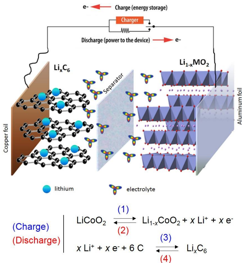
Figure A1. Schematic working principle of a Li-ion cell (image reproduced from the University of Waterloo website).
