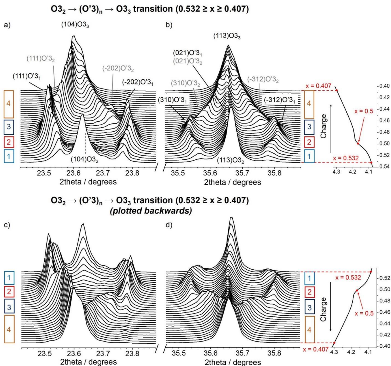
Figure B14. Changes detected on the a) (104)\text{O}3_2 and b) (113)\text{O}3_2 diffraction lines during the charge of st-LCO at C/20 in the 0.532 \geq x \geq 0.407 range, in which the \text{O}3 - \text{O}'3 transition is expected. The corresponding voltage profile of the cell is provided on the right of the figure. Rectangles with numbers delimit four domains, each domain being defined by both the nature and the number of phases identified in the SXRD patterns (see Figure B15). Alternative plots of the same data are provided in c) and d) .
