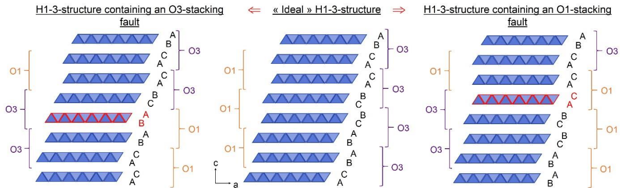
Figure B7. Schematic representation of the CoO 2 stacking in the ideal H1-3 structure, as opposed to an H1-3 structure containing either an O1-type stacking fault or an O3-type stacking fault. The letters refer to oxygen positions arbitrarily used to describe these structures ( A(0, 0, z_A) , B(\frac{1}{3}, \frac{2}{3}, z_B) and A(\frac{2}{3}, \frac{1}{3}, z_C) ).
