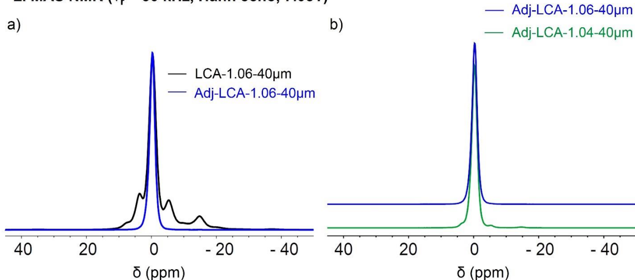
Figure C31. ^7\text{Li} MAS NMR spectra recorded at 116.66 MHz using a 30 kHz spinning frequency of a) LCA-1.06-40 \mu m and Adj-LCA-1.06-40 \mu m; b) Li-adjusted samples from Group B: Adj-LCA-1.04-40 \mu m and Adj-LCA-1.06-40 \mu m.
