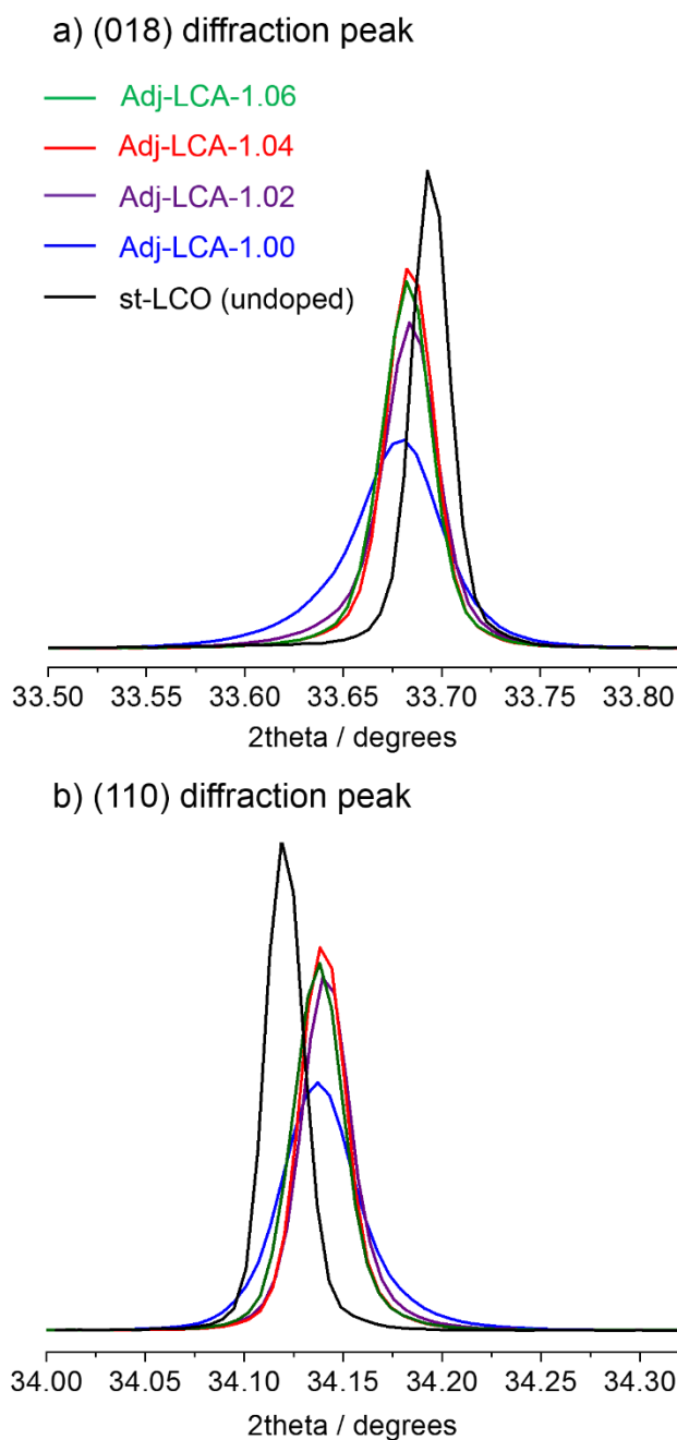
Figure C25. Zoom on the a) (0 1 8) and b) (1 1 0) diffraction peaks from the Synchrotron X-ray diffraction (SXRD) patterns shown in Figure C23.
