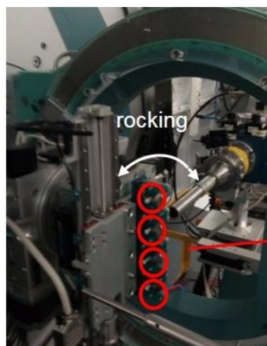
Measurement setup at the MSPD-BL04, ALBA synchrotron
