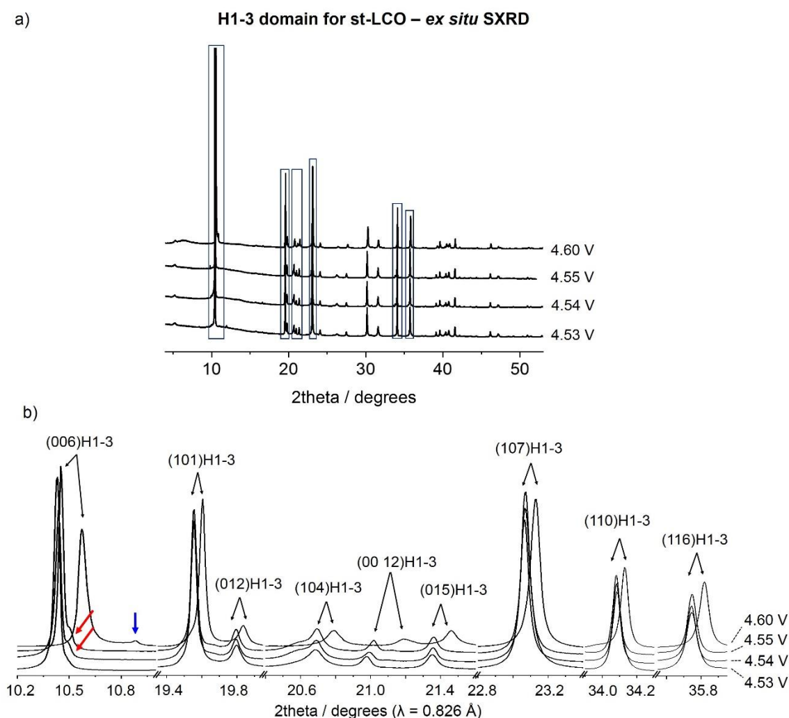
Figure B23. a) Ex situ SXRD patterns recorded for various H1-3-Li x CoO 2 powders prepared from electrochemical Li de-intercalation of st-LCO charged up to either E = 4.53 V, E = 4.54 V, E = 4.55 V or E = 4.60 V. Zooms on the most intense diffraction lines are given in b).
