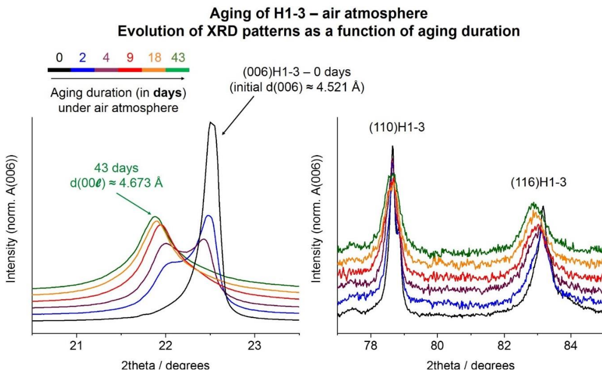
Figure B28. Ex situ XRD patterns recorded at various aging time for the same H1-3- \text{Li}_x\text{CoO}_2 powder left under air for 43 days ( \lambda_{\text{CoK}\alpha 1} = 1.789 \text{ \AA} , \lambda_{\text{CoK}\alpha 2} = 1.793 \text{ \AA} ). The powder was initially prepared from electrochemical Li de-intercalation of st-LCO charged up to E = 4.53 \text{ V} .
