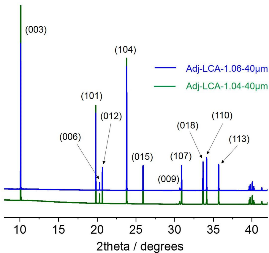
Figure C33. Synchrotron X-ray diffraction (SXRD) patterns obtained for Li-adjusted LCA from Group B. All patterns were collected for \lambda = 0.826 \text{ \AA} . Miller indexes for the main peaks are also given.
