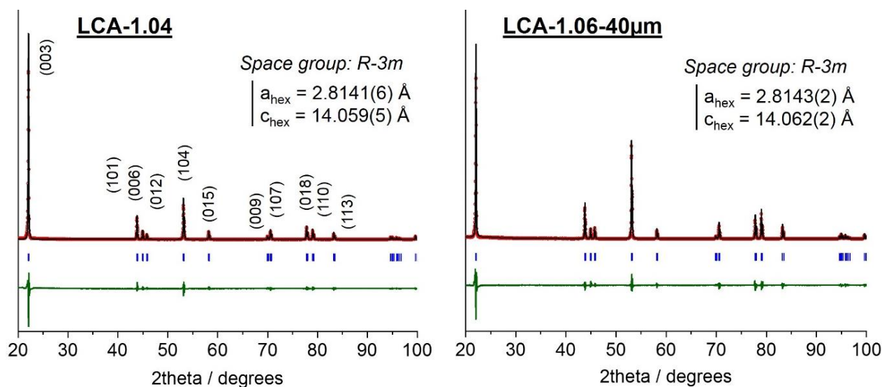
Figure C40. XRD patterns collected for the intermediate LCA-1.04 (Group A) and LCA-1.06-40 \mu m (Group B). Cell parameters were obtained from Le Bail refinements (also shown here). The Miller indexes for the mains peaks are also provided.
