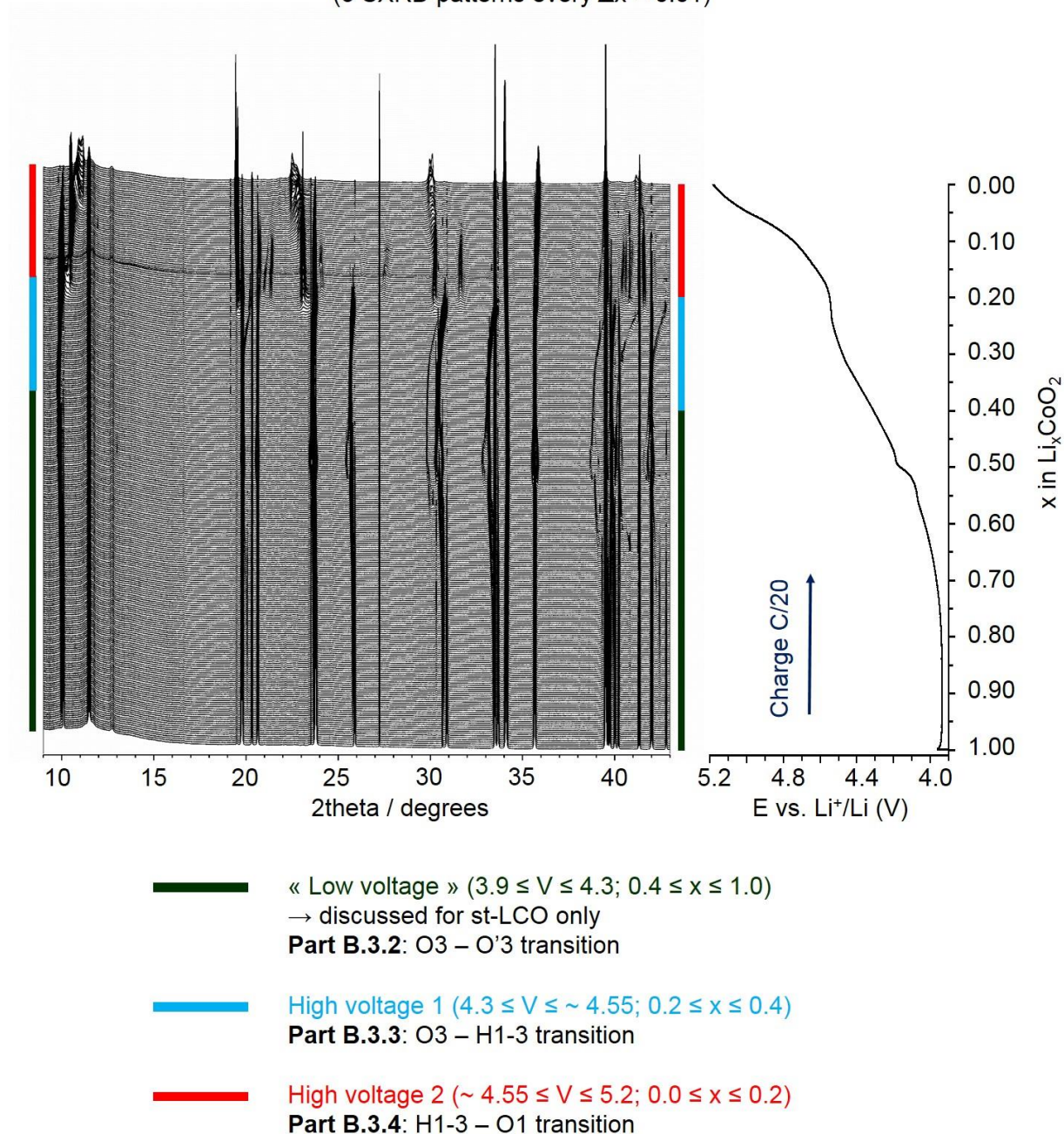
Figure B10. Cumulated \sim 275 XRD patterns recorded in situ operando during the full charge of st-LCO and collected with \lambda = 0.825 \text{ \AA} . The associated electrochemical curve is given on the right. The green, blue and red rectangles denote the three successive electrochemical windows that will be commented upon in part B.3.
