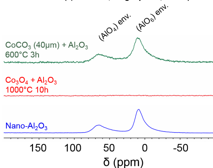
Figure C29. ^{27}\text{Al} MAS NMR spectra recorded at 130.33 MHz using a 30kHz spinning frequency for (\text{CoCO}_3 + \text{Al}_2\text{O}_3) heat treated at 600 °C for 3 hours (in green) and (\text{Co}_3\text{O}_4 + \text{Al}_2\text{O}_3) heat treated at T = 1000 °C for 10 hours (in red), as compared to the spectra of pure alumina (in blue). Note that Group A samples were formed from the red precursors, while Group B samples were obtained from the green precursor.
