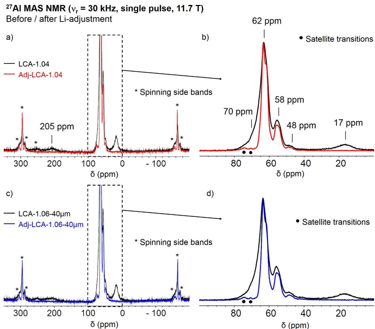
Figure C41.a) ^{27}\text{Al} MAS NMR spectra recorded at 130.33 MHz using a 30 kHz spinning frequency for non Li-adjusted LCA-1.04 (Group A), as compared to its Li-adjusted analogue Adj-LCA-1.04. A zoom on the central transitions is given in b). c) ^{27}\text{Al} MAS NMR spectra recorded at 130.33 MHz using a 30 kHz spinning frequency for non Li-adjusted LCA-1.06-40 \mu\text{m} (Group B), as compared to its Li-adjusted analogue Adj-LCA-1.06-40 \mu\text{m} . A zoom on the central transitions is given in d).
