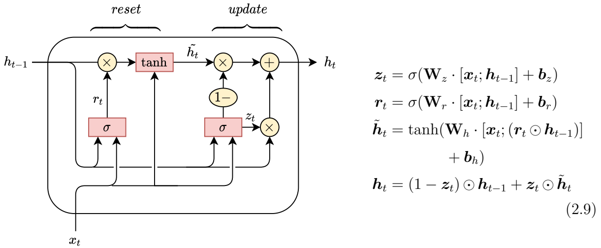
FIGURE 2.6 – Architecture GRU
