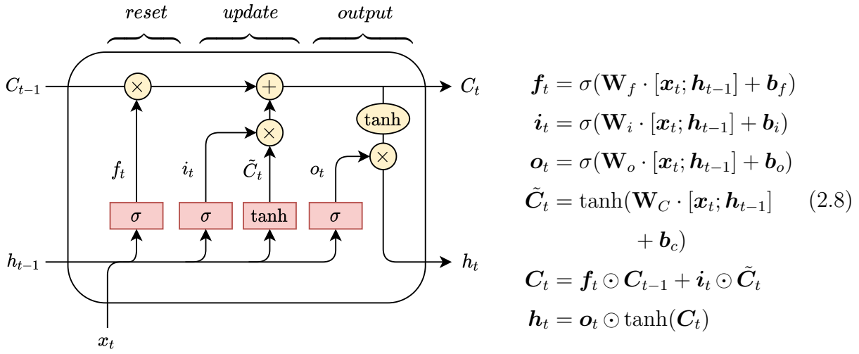
FIGURE 2.5 – Architecture LSTM
