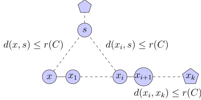
Figure 4.7: Distance relations between vertices x , s and x_k used for Proposition 36
