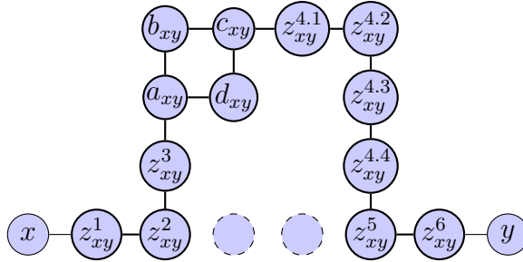
Figure 3.7: Gadget T_{xy}^1 used in F for (x, y) \in E^{H_q} .
