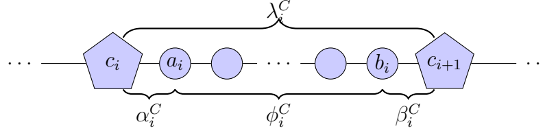
Figure 5.1: Values \lambda_i^C , \alpha_i^C , \phi_i^C and \beta_i^C illustrated on a segment \mu_i^C
