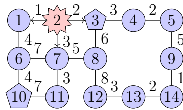
Figure 2.3: The operational graph associated with scenario 2 with shelters located on \{3, 10\}
