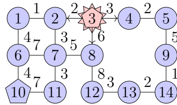
Figure 2.4: The operational graph associated with scenario 3 with shelters located on \{3, 10\}
