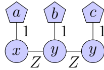
Figure 4.6: A case where \frac{\mathbf{E}(C)}{r(C)} = Z + 1 .
