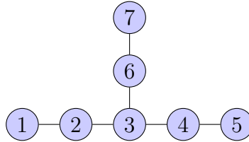
Figure 2.7: An example where, for p = 5 , there is an optimal solution for \text{RpCP} and \text{PpCP} of size 4.
