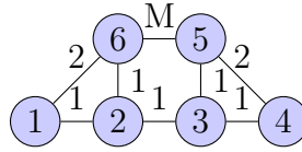
Figure 2.6: An example of different optimal solutions for \text{Min } p\text{-Center} and \text{RpCP} with p = 2 .
