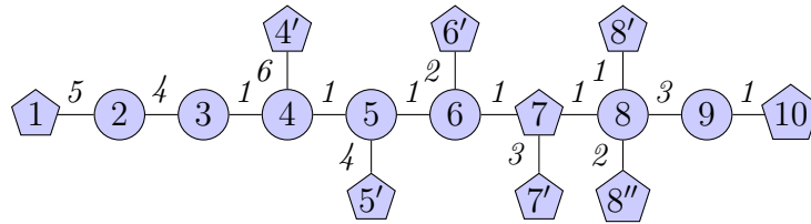
Figure 5.5: Example of the notation of a caterpillar.
