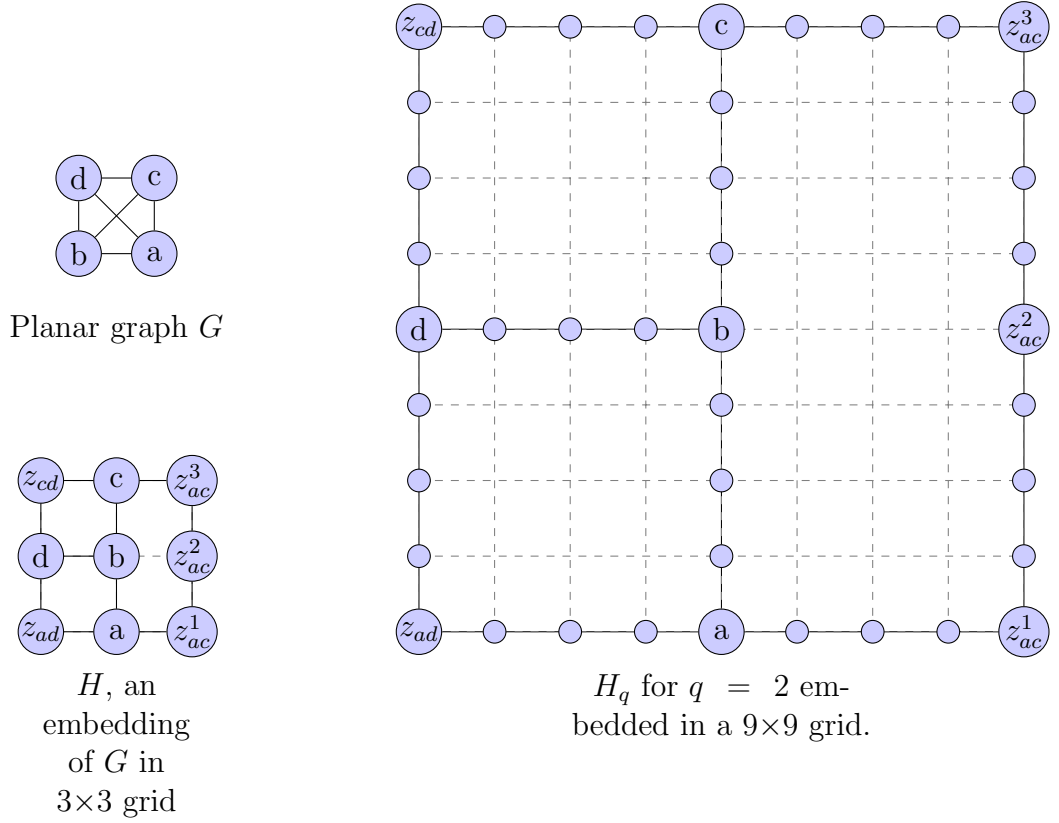
Figure 3.4: Example of Transformation 1
