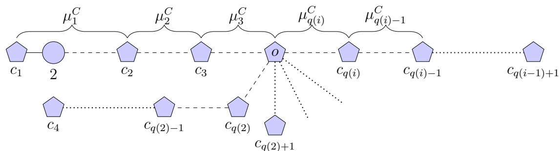
Figure 5.4: Example of notations on an extended star.
