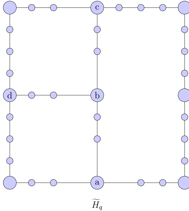
Figure 3.5: The graph \tilde{H}_q obtained from G through H_q . k_{ab} = k_{bc} = k_{bd} = 1 , k_{ad} = k_{cb} = 3 and k_{ac} = 7
