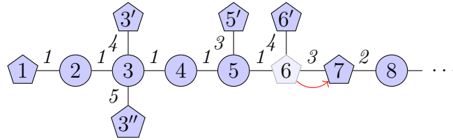
Figure 5.6: Applying Algorithm 5 on a caterpillar for k -RCP with k = 5 , the red arc shows the relocation of the shelter from vertex 6 to vertex 7 at the beginning of iteration 7.
