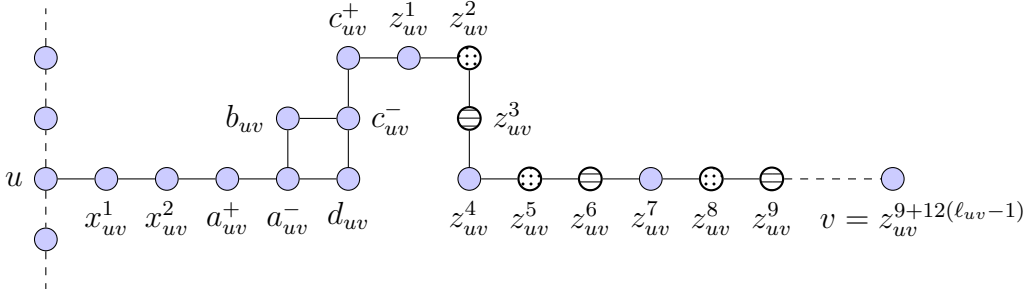
Figure 3.2: The subgraph \tilde{T}_{uv} for the edge (u, v) oriented from u to v and \ell_{uv} > 1 . Continuous lines are used for T_{uv} 's edges while dashed lines correspond to edges outside T_{uv} .
