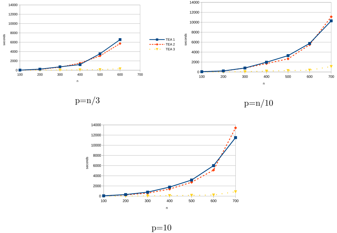
Figure 6.1: Processing time of each variant of the Exact Algorithm on some OR-Library instances
