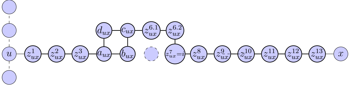
Figure 3.6: Gadget T_{ux}^2 used in F for (u, i), (i, x) \in E^{H_q} ; z_{ux}^7 = i .
