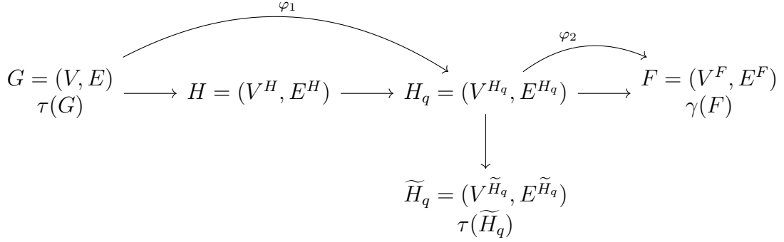
Figure 3.3: The different graphs involved in the reduction.
