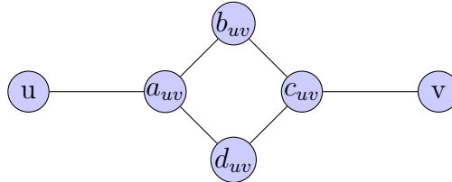
Figure 3.1: The gadget L_4 for an edge (u, v)
