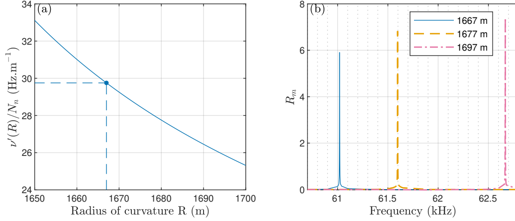
Figure 6.7: (a): \nu'_n(R_{\text{EM}})/N_n for an arm cavity, in AdV's configuration ( x = \{1, 2, 3, 4\} , L_{1,2,3,4} = 2999.8 m, and \text{FSR} \approx 50 kHz). (b) parametric gain R_m of the mechanical mode of the third couple of fig. 3.6 for various radii of curvature. A radius-of-curvature shift ultimately leads to a frequency shift of the HOM, which, in turn, modifies the beat note, and then the optical resonant frequency. The optical mode is an order 2, then the frequency shift matches the one expected by (a).
