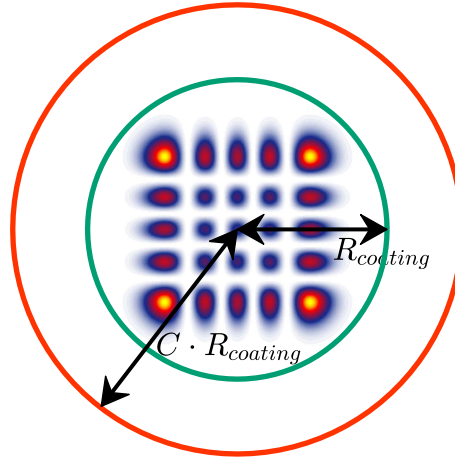
Figure 5.10: Method to estimate the diffraction losses of the HGM. This one is the \text{HG}_{44} . The green circle highlights the coating radius R_{\text{coating}} of the mirrors of Adv's arm cavities. The red circle highlights a larger radius built to mimic an infinite mirror and is C times larger than R_{\text{coating}} .
