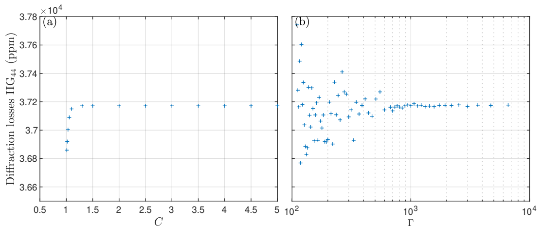
Figure 5.11: Convergence tests for the \text{HG}_{44} diffraction loss. (a) Diffraction loss while making C vary, with a fixed \Gamma_0 = 3500 . A convergence is reached for C = 1.5 . (b) Diffraction loss while making \Gamma vary, with a fixed C_0 = 1.5 . A convergence is reached from \Gamma = 650 .
