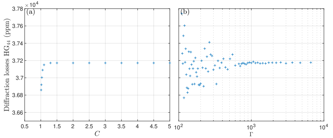
Figure 5.11: Convergence tests for the HG_{44} diffraction loss. (a) Diffraction loss while making C vary, with a fixed \Gamma_0 = 3500 . A convergence is reached for C = 1.5 . (b) Diffraction loss while making \Gamma vary, with a fixed C_0 = 1.5 . A convergence is reached from \Gamma = 650 .
