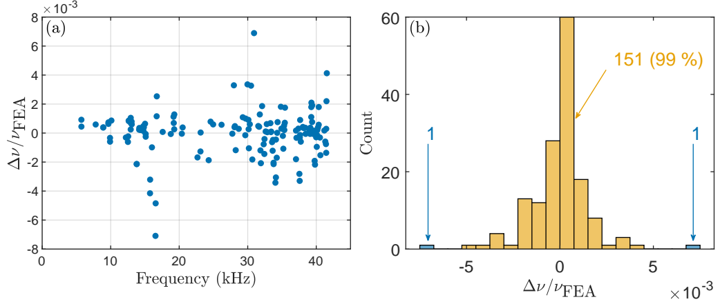
Figure 4.2: (a) Relative differences of measured frequencies with respect to frequencies obtained with the FEA vs the FEA frequencies. The standard deviation \sigma(\nu_{\text{meas}}) is 0.15 %. (b) Distribution of the relative differences; the bin width is \sigma(\nu_{\text{meas}})/2 . There are 153 data, of which 151 (99 %) are comprised within \pm 3.5 \sigma(\nu_{\text{meas}}) \approx \pm 0.50 \% .
