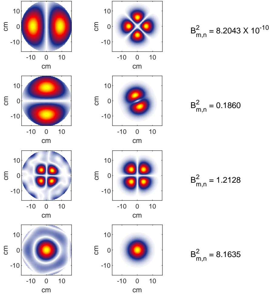
Figure 3.6: On the left, the surface displacements of various mechanical modes. In the middle, some optical modes. On the right, the associated squared spatial overlap parameters B^2_{m,n} . Downwards, the optical modes are respectively the FSMM(5) (order 2), the FSMM(3) (order 1), the FSMM(4) (order 2), and the FSMM(1) (order 0). The FSMM will be introduced in section 5.3.3.
