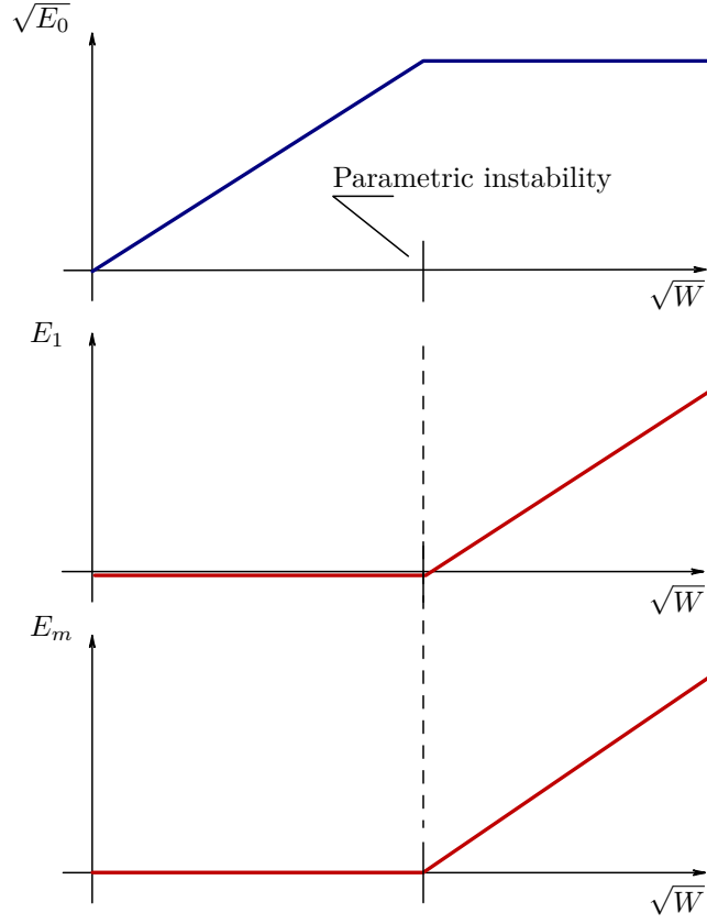
Figure 3.2: Energy in the fundamental mode E_0 , energy in the Stokes E_1 , and energy in the mechanical mode E_m with respect to the laser power W , below and above the OPI threshold. Image adapted from [59].
