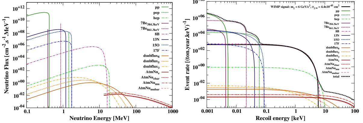
Figure 1.4: Left: Relevant neutrino fluxes to the background of direct dark matter detection experiments: Solar, atmospheric, and diffuse supernovae [123, 124, 125]. Right: Neutrino background event rates for a germanium based detector. The black dashed line corresponds to the sum of the neutrino induced nuclear recoil event rates. Also shown is the similarity between the event rate from a 6 \text{ GeV}/c^2 WIMP with a SI cross section on the nucleon of 4.4 \times 10^{-45} \text{ cm}^2 (black solid line) and the {}^8\text{B} neutrino event rate. Figures taken from [89]
