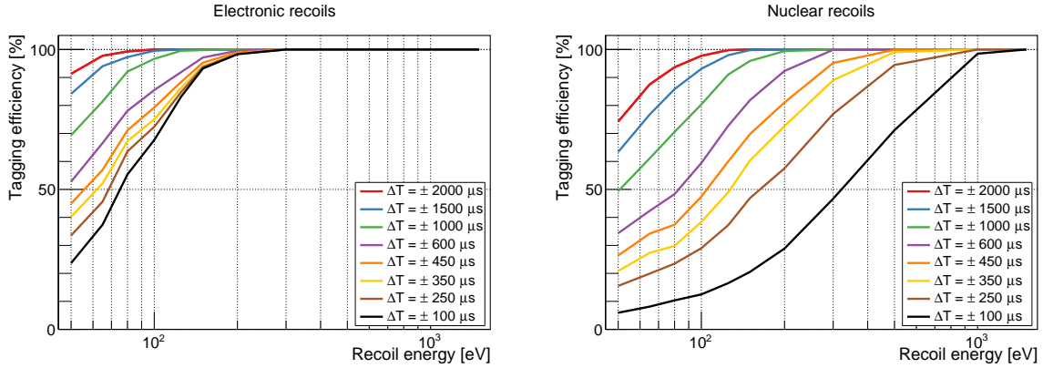
Figure 4.9: Tagging efficiency as a function of recoil energy for electronic ( left ) and nuclear ( right ) recoils, with varying lengths of time windows ranging from 2 ms (red) to 100 \mu\text{s} (black).
