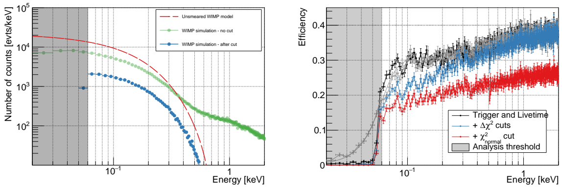
Figure 2.7: Left: Simulation of a 2 \text{ GeV}/c^2 WIMP energy distribution where we show the theoretical unsmearred distribution (red long-dashed line), the resulting simulated energy distribution before (green) and after (blue) applying all the selection cuts detailed in the main text. Right: Signal efficiency as a function of heat energy for 10^6 simulated events injected in the data stream with energies uniformly generated between 0 and 2.5 keV, shown from 0 to 2 keV corresponding to the region of interest. Grey points: trigger plus live-time efficiency as a function of the input energy, together with a fit with an error function (grey line). Black points and line: trigger plus live-time efficiency as a function of the energy resulting from the \chi^2 fit of a pulse to the data in the frequency domain. Blue points and line: the same, but after applying all \Delta\chi^2 cuts. Red points and line: the final efficiency obtained after applying the additional cut on \chi^2_{\text{Normal}} . In both panels, the grey area corresponds to energies below the analysis cut. Figures taken from [97].
