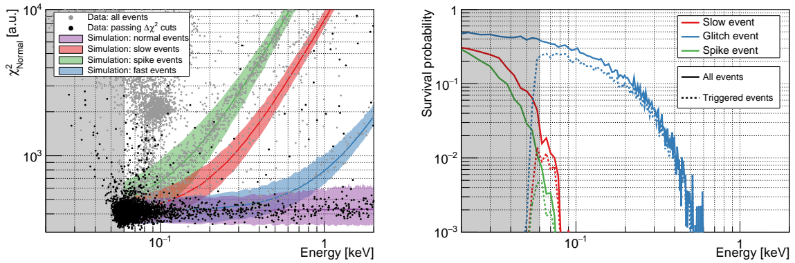
Figure 2.6: Left: Distribution of \chi_{\text{Normal}}^2 as a function of energy for the events in the blinded data set. The events passing all \Delta\chi^2 cuts are shown as black dots while those rejected are shown as grey dots. The expected region where different pulse populations are expected are shown in purple (events with normal pulse shape), blue (fast pulses), red (slow pulses) and green (single-sample spikes). Right: Survival probability of the three type of background events: blue (glitch/fast pulses), red (slow pulses) and green (single-sample spikes), with (solid line) and without (dashed line) considering the trigger selection. Figures taken from [97].
