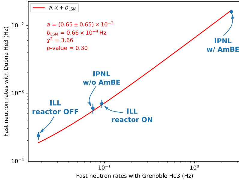
Figure 3.12: Correlation between the fast neutron measurements from the ILL (x-axis) and JINR (y-axis) 3 He PC, realised at the ILL-H7 site and at IP2I.
