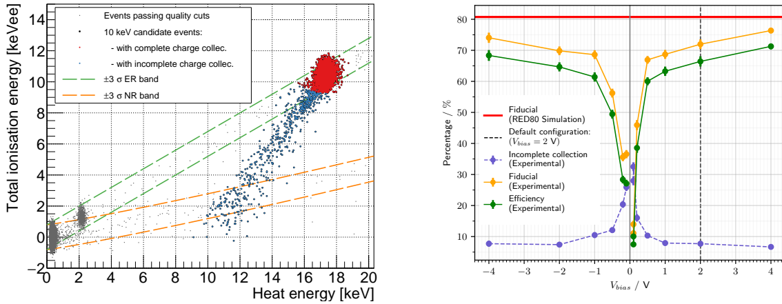
Figure 5.8: Left: Event distribution in the total ionisation energy, defined as (Ei_A + Ei_B + Ei_C + Ei_D)/2 , versus heat energy from a “background” data taking period with a 2 V voltage bias (tg181005). The events shown in grey are passing all the data quality selection cuts, while the black ones are 10.37 keV candidate events with the red (blue) ones exhibiting a complete (incomplete) charge collection. For illustration we also show the \pm 2\sigma ER and NR bands in green and orange dashed lines respectively. Right: Measurement of the fraction of: incomplete charge collection (purple), fiducial volume (orange), and combined fiducial and collection efficiency (green), as a function of the voltage bias. The vertical dashed line at 2 V corresponds to the bias voltage used in our neutron calibration and background characterization discussed in Sec. 5.3.4. Figure taken from [228].
