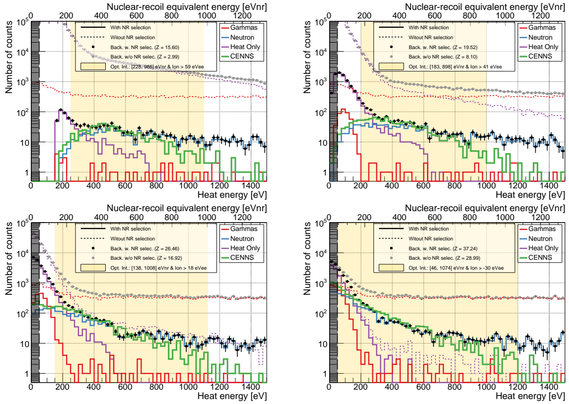
Figure 4.13: Simulated heat energy distributions with the same background and detector model parameters as given in Tab. 4.4 with varying HO background reduction factors of 10 (top left), 100 (top right), 1000 (bottom left), and 10000 (bottom right).
