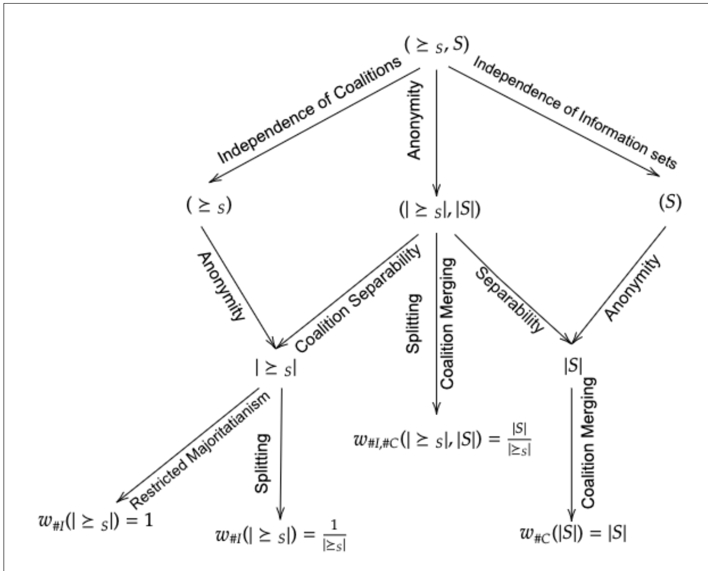
Figure 4.1: Being sub-family relation between different families.
