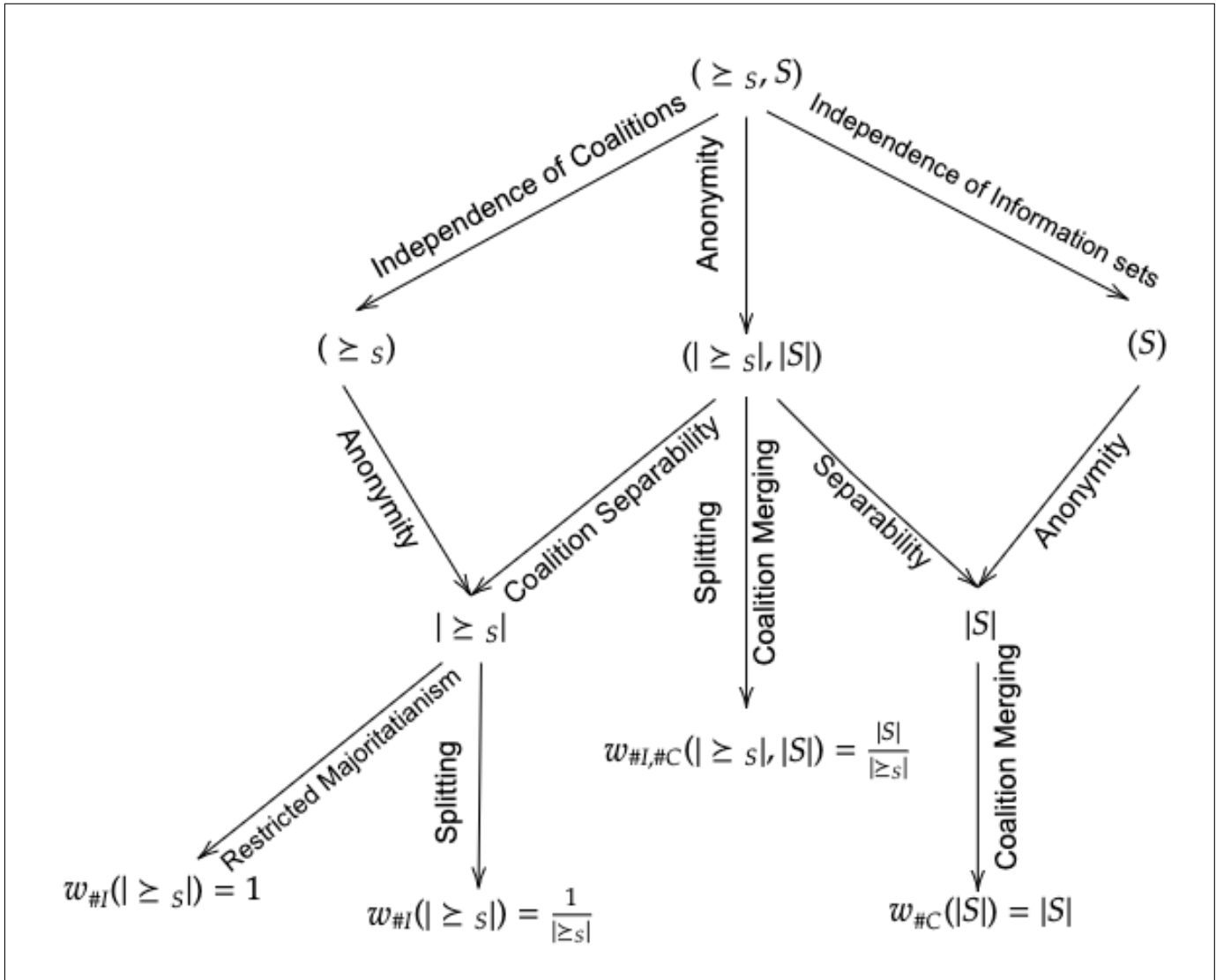
Figure 6.1: Being sub-family relation between different families.
