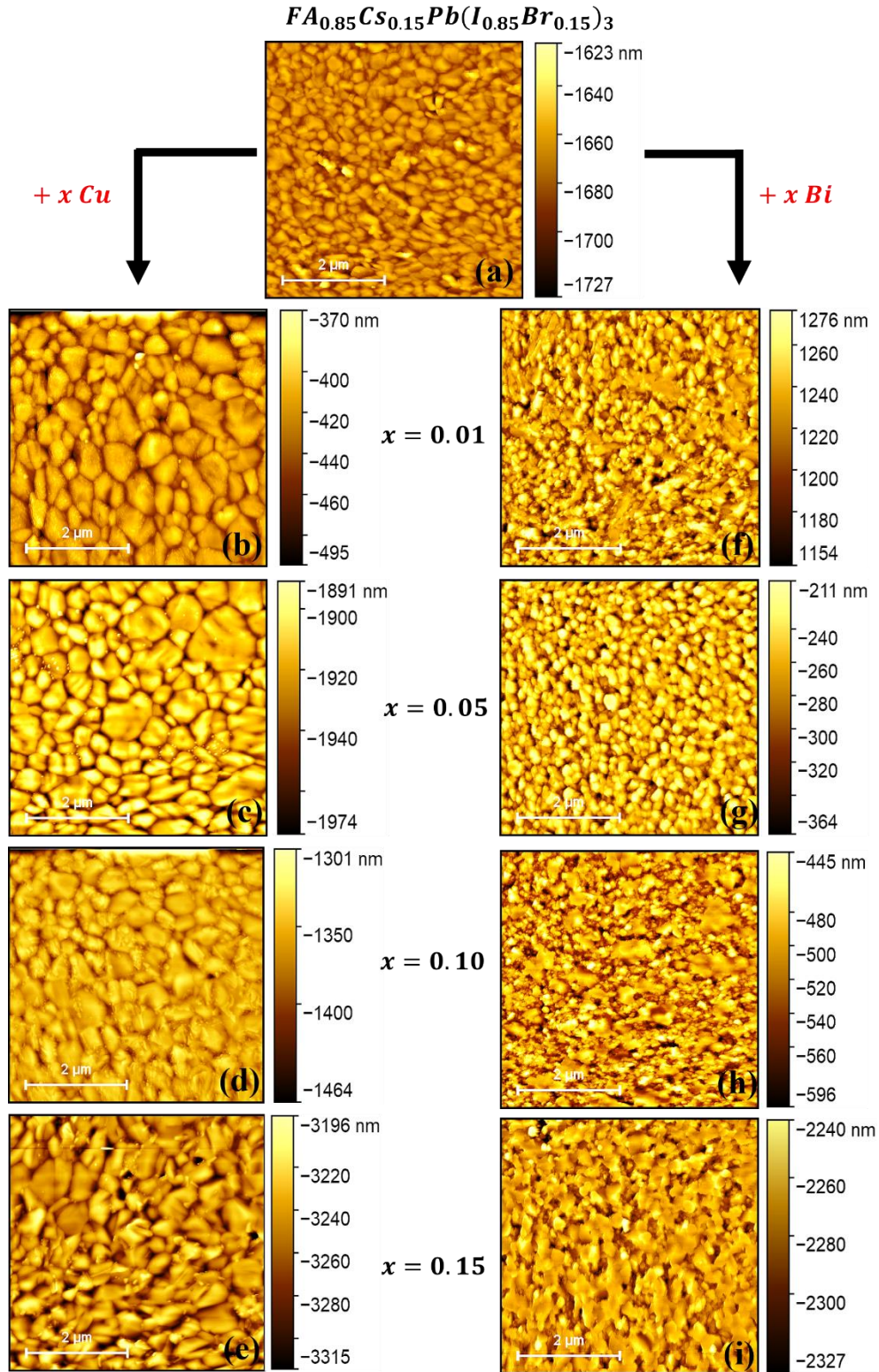
Fig. 8.2. AFM topographical images of undoped FA_{0.85}Cs_{0.15}Pb(I_{0.85}Br_{0.15})_3 , as well as both Cu- and Bi-doped perovskite films. Horizontal scale bar: 2 \mu m.
