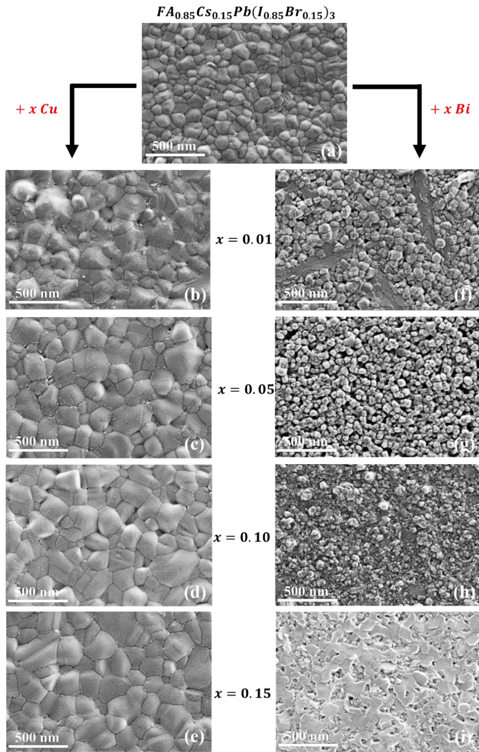
Fig. 8.1. SEM photographs of undoped FA_{0.85}Cs_{0.15}Pb(I_{0.85}Br_{0.15})_3 as well as both Cu and Bi - doped perovskite films. Scale bar: 500 nano-meter.
