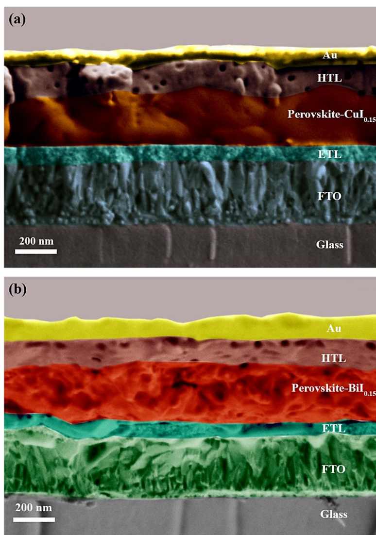
Fig. 8.10. Cross-sectional SEM images of Cu ( x = 0.15 ) (a) and Bi ( x = 0.15 ) (b) doped devices based on the planar FTO/ \text{SnO}_2 /perovskites/Spiro/Au device configuration.
