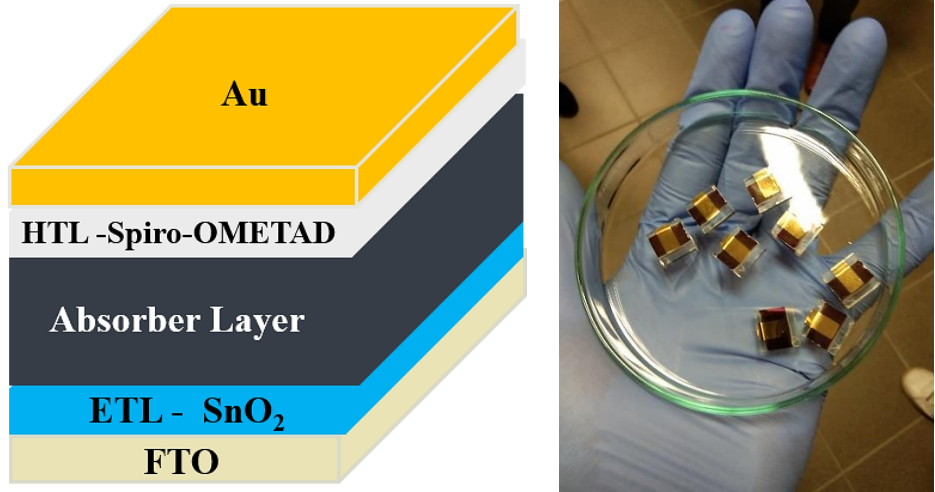
Fig. 4.5. Schematic of the complete perovskite device.
