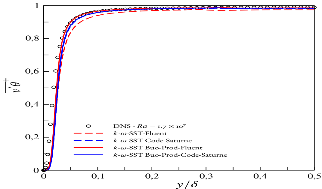
Figure A.9 – Comparison of wall normal heat flux ( \overline{vT^+} ) profiles for buoyancy sensitised k-\omega -SST model in Fluent (red color) and in Code Saturne (blue color) with DNS data Kiß and Herwig [2014] at Ra = 1.7 \times 10^7 and Pr = 0.71
