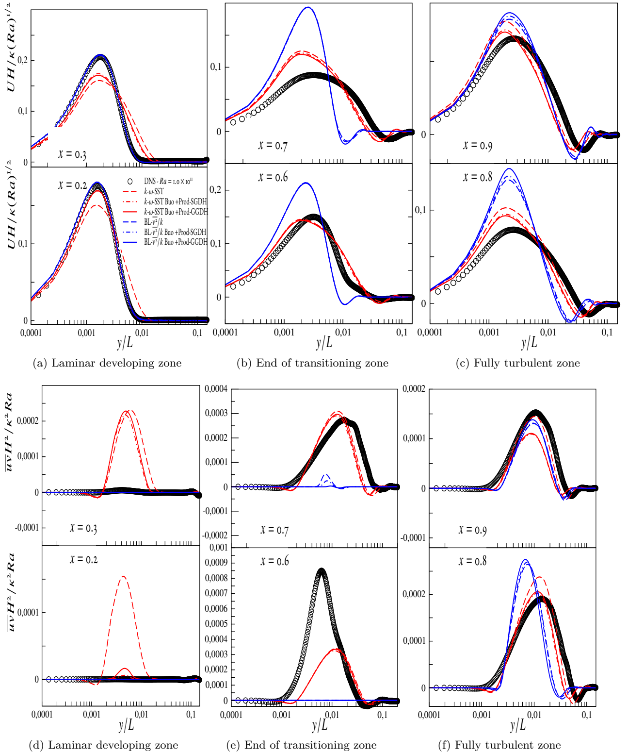
Figure 5.9 – Comparison of mean velocity [\overline{UH}/\kappa(Ra)^{1/2}] (first line) and turbulence shear stress [\overline{uv}H^2/\kappa^2 Ra] (second line) predictions of buoyancy sensitised k-\omega -SST and BL-\overline{v^2}/k models with DNS data [Trias et al., 2010] at Ra = 1 \times 10^{11} and Pr = 0.71
