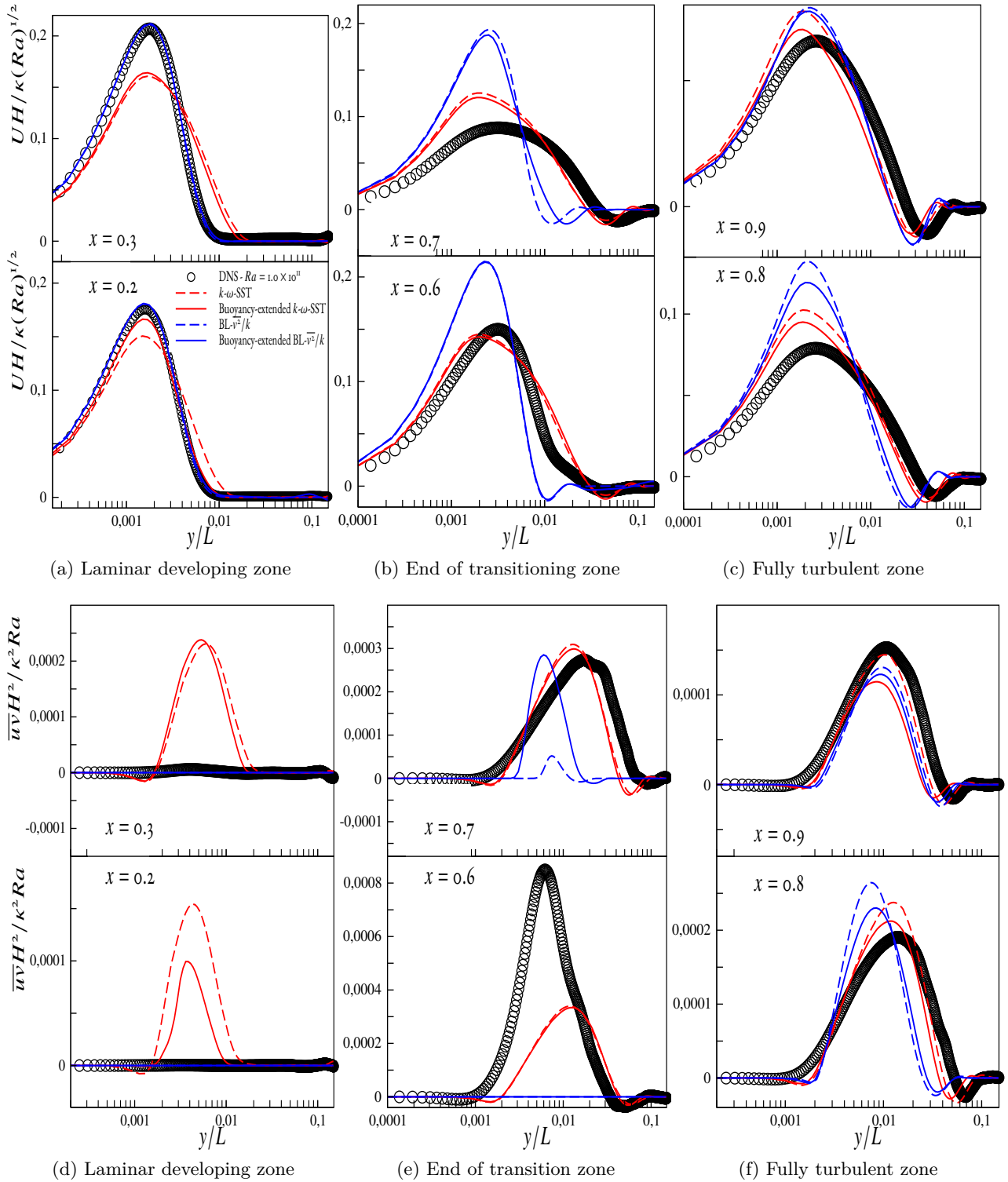
Figure 5.5 – Comparison of the mean velocity [UH/\kappa(Ra)^{1/2}] (first line) and turbulence shear stress [\overline{uv}H^2/\kappa^2 Ra] (second line) predictions of the buoyancy-extended k-\omega -SST (red color) and buoyancy extended BL-\overline{v^2}/k (blue color) models with DNS data [Trias et al., 2010] at Ra = 1.0 \times 10^{11} and Pr = 0.71
