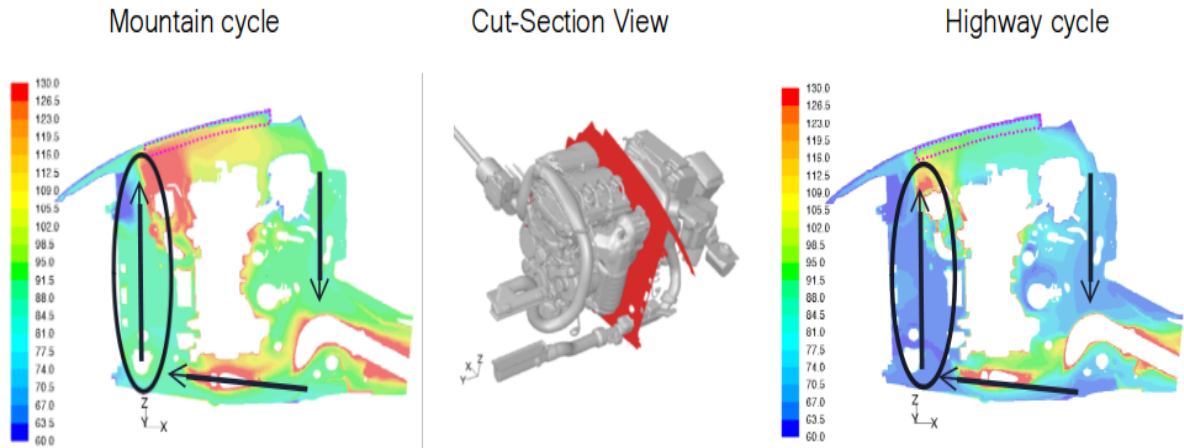
Figure 1.2 – Cut section view of the simulation after stabilising of forced convection phase [Plots are taken from simulation performed at PSA Group, Courtesy (V. Herbert)]
