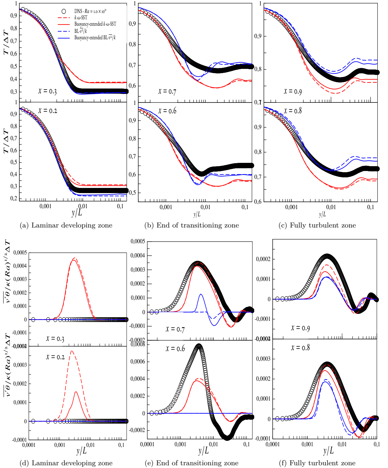
Figure 5.6 – Comparison of mean temperature [T/\Delta T] (first line) and wall normal heat flux [\overline{v'\theta}H/\kappa(Ra)^{1/2}\Delta T] (second line) predictions of buoyancy-extended k\text{-}\omega\text{-SST} (red color) and buoyancy extended BL\text{-}v^2/k (blue color) models with DNS data [Trias et al., 2010] at Ra = 1.0 \times 10^{11} and Pr = 0.71
