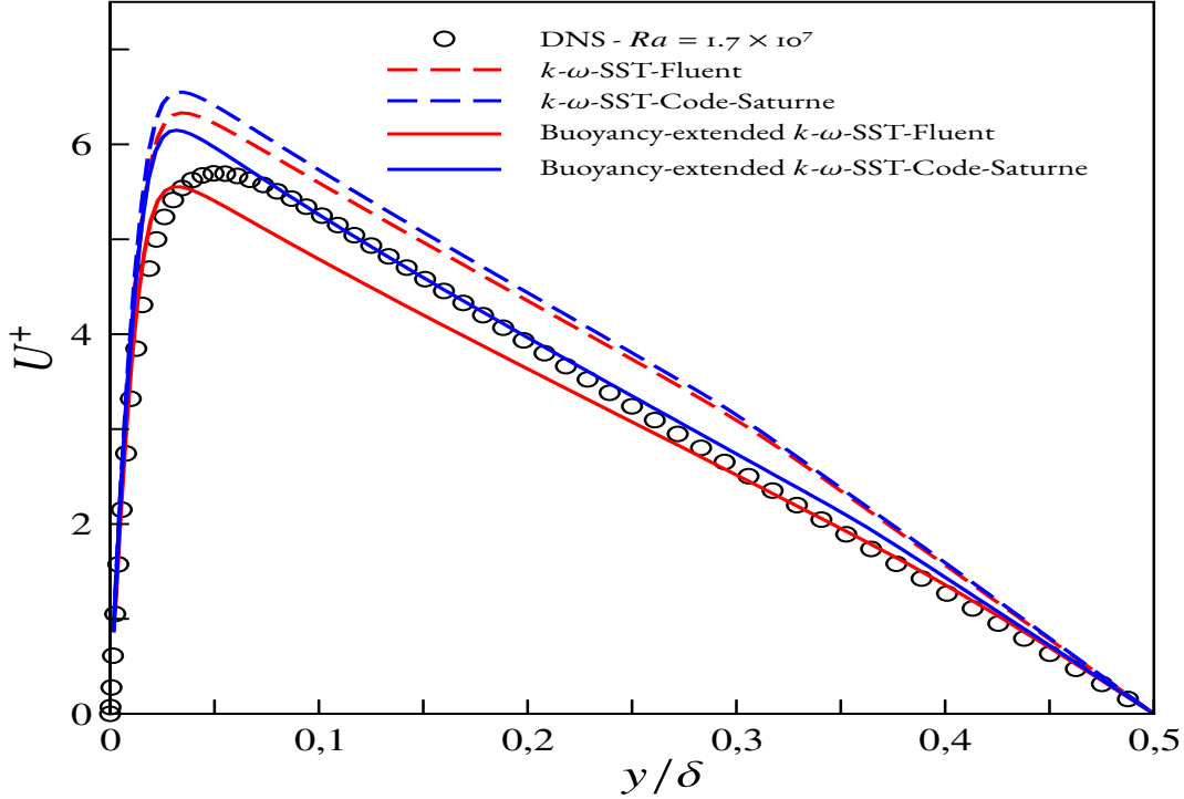
Figure A.2 – Comparison of mean velocity ( U^+ ) profiles for buoyancy extended k- \omega -SST model in Fluent (red color) and in Code Saturne (blue color) with the DNS data Kiš and Herwig [2014] at Ra = 1.7 \times 10^7 and Pr = 0.71
