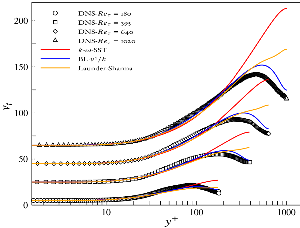
Figure 3.7 – Turbulent viscosity at Re_\tau = 180, 395, 640, 1020 [Plots are shifted for clarity]
