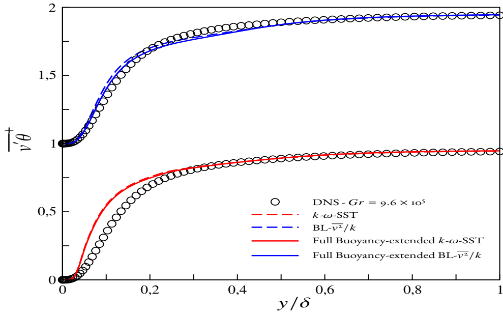
Figure 4.16 – Wall normal heat flux for the aiding side at Gr = 9.6 \times 10^5 [Kasagi and Nishimura, 1997] [Plots are shifted for clarity]
