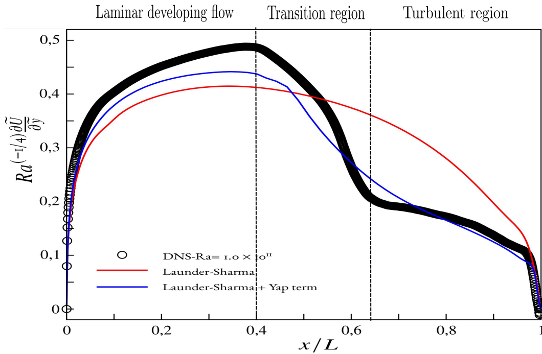
Figure 5.11 – Comparison of vertical wall shear stress scaled by Ra^{-1/4} with DNS data [Trias et al., 2010] at Ra = 1.0 \times 10^{11} and Pr = 0.71
