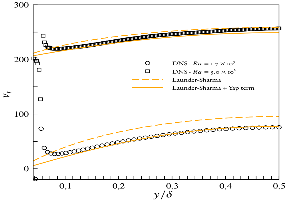
Figure 3.25 – Turbulent viscosity at Ra = 5 \times 10^6 [Versteegh and Nieuwstadt, 1996](denoted by \square ) and Ra = 1.7 \times 10^7 [Kiš and Herwig, 2014](denoted by \circ ) [Plots are shifted for clarity]
