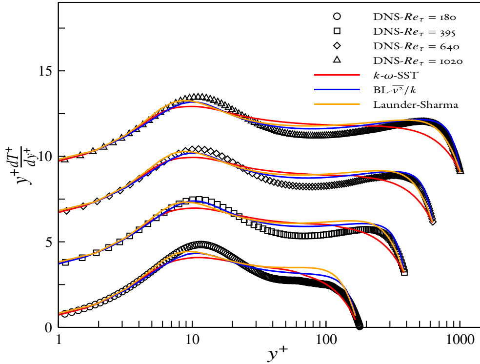
Figure 3.9 – Premultiplied temperature gradient at Re_\tau = 180, 395, 640, 1020 [Plots are shifted for clarity]
