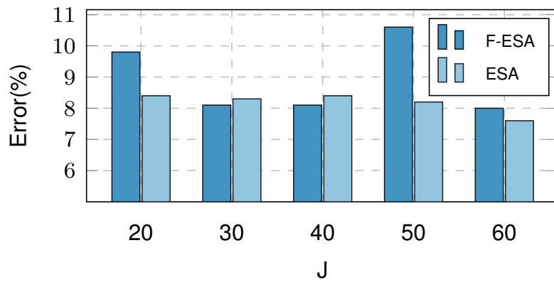
Figure 3.19 – Comparing the percentage error for F-ESA and ESA with topology C for different values of J
