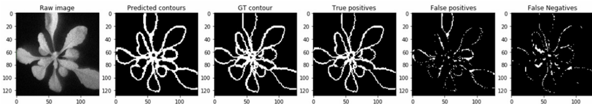
Figure 3.18 – Leaf segmentation results for different training strategies.
