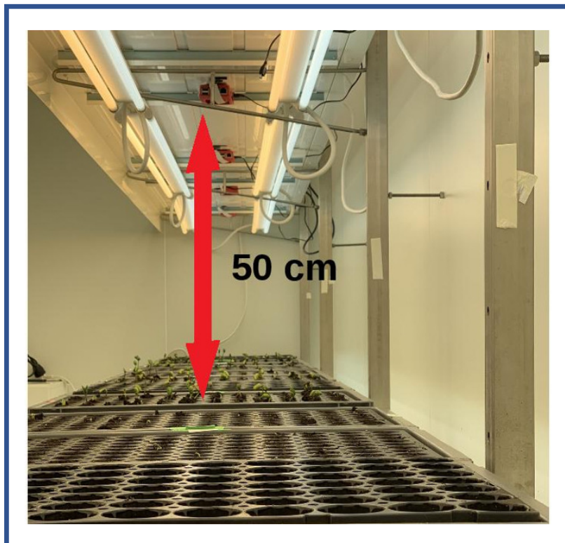
Figure 2.14 – Imaging system installed in a growth chamber.
