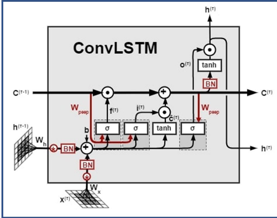
Figure 2.20 – ConvLSTM block with one cell [71]
