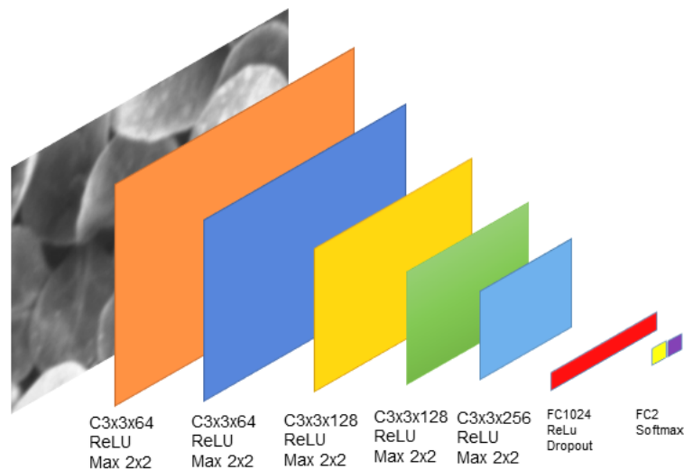
Figure 3.24 – Architecture of the deep network optimized for the task on classification.
