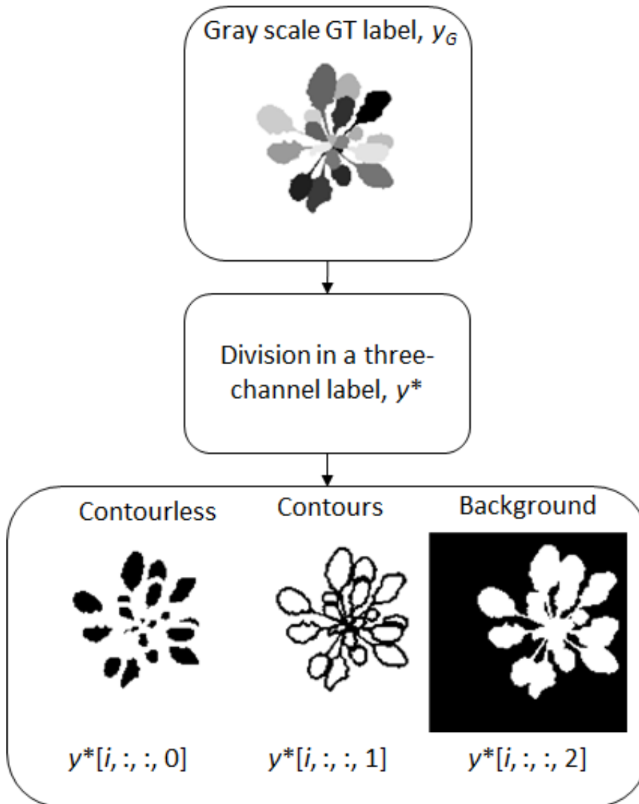
Figure 3.16 – Production of the three-channel binary labels from ground-truth (GT) label: the first channel contains mask without leaf contours, the second - leaf contours, and the third one - background.
