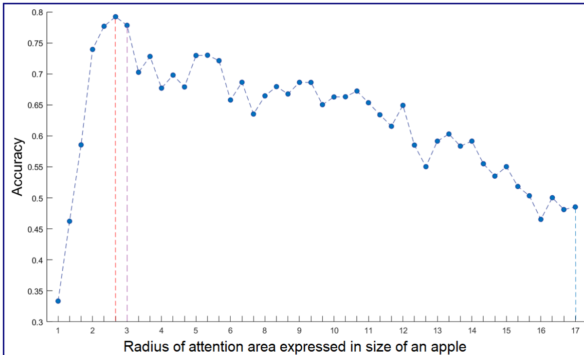
Figure 3.12 – Apple segmentation accuracy as a function of the radius of attention area expressed in the size of apples taken as 30 pixels. Maximum accuracy achieved when the radius size of the attention map is equal to 80 ( 160 \times 160 pixels) corresponding to the red dotted line. The purple dotted line corresponds to the maximum gaze shift error of (169 pixels) between eye-tracker and ground-truth when computed on the whole dataset.
