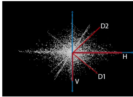
Figure 4. Elements computed in the anisotropy ratio of Eq. (1) applied on the modulus of the Fourier transform.
