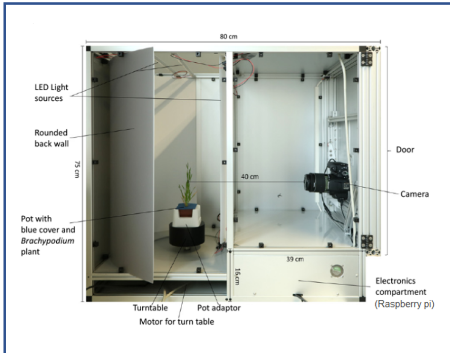
Figure 2.12 – Side-view of the PhenoBox. The camera and turntable are controlled by a Raspberry Pi 3 mini-computer. Reproduced from [13].
