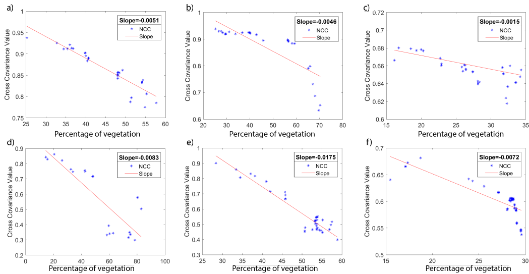
Figure 14. Normalized cross-covariance as a function of the percentage of vegetation. a) Same tree-Same size-Same orientation-Two side, b) Different orientation-Two side, c) Different orientation-One side, d) Forest, e) Different tree-Different size-Different orientation-Two side, f) Same tree-Same size-Same orientation-One side
