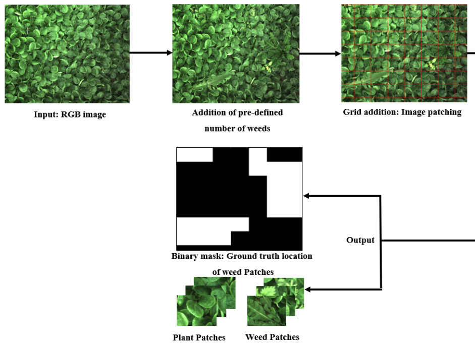
Figure 3.5 – Simulation pipeline for the creation of images of plant with weed of Fig. 3.4 similar to the one presented in Fig. 3.3.
