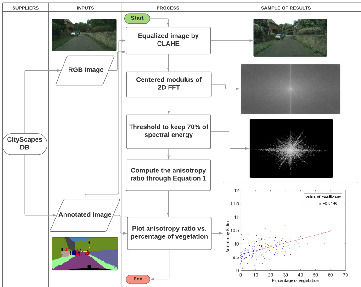
Figure 3. Image processing pipeline for the study of the impact of vegetation in the Fourier domain. CityScapes DB [30] corresponds to an available dataset as illustrated in Fig. 1.
