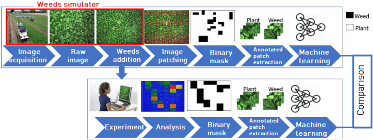
Figure 3.6 – General pipeline of comparison of eye-tracked annotated data with ground-truth.
