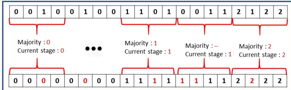
Figure 2.21 – An example of the post-processing step on predicted classes where the sliding window size is four images.
