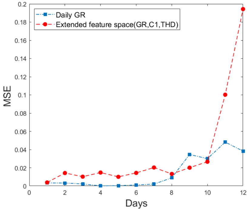
Figure 2.28 – Contrast between control and salt stress for the sole growth rate (Daily GR) and for the extended feature space of Eq. (2.12) computed by the MSE of Eq. (2.13).
