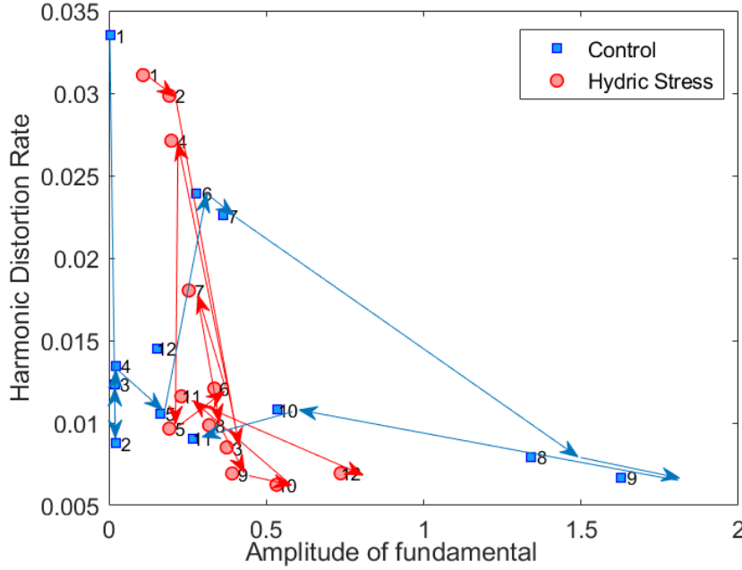
Figure 2.26 – Temporal trajectories of growth represented in a HDR, c_1 graph for control in blue and hydric stress in red. The arrows indicate the flow of time.
