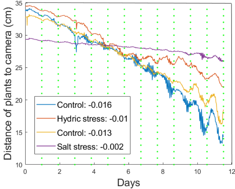
Figure 2.25 – Spatial average of the distance map x(t) to the camera in cm as a function of time in various conditions. The values indicated in the inset correspond to average growth rates in centimeter per minute.
