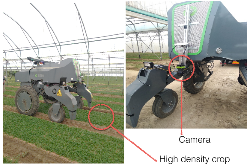
Figure 3.2 – Global view of the imaging system fixed on a robot moving above mache salads of high density. RGB images are captured by a JAI manufactured camera of 20Mpixels with a spatial resolution of 5120x3840 pixels, mounted with a 35 mm objective. The typical distance of plants to camera is of 1 meter.
