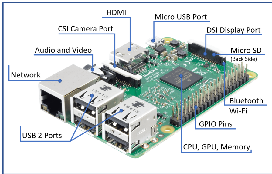
Figure 2.1 – Raspberry Pi version 3B - mini-computer used in seedling growth monitoring in our work on individual observation scale.
