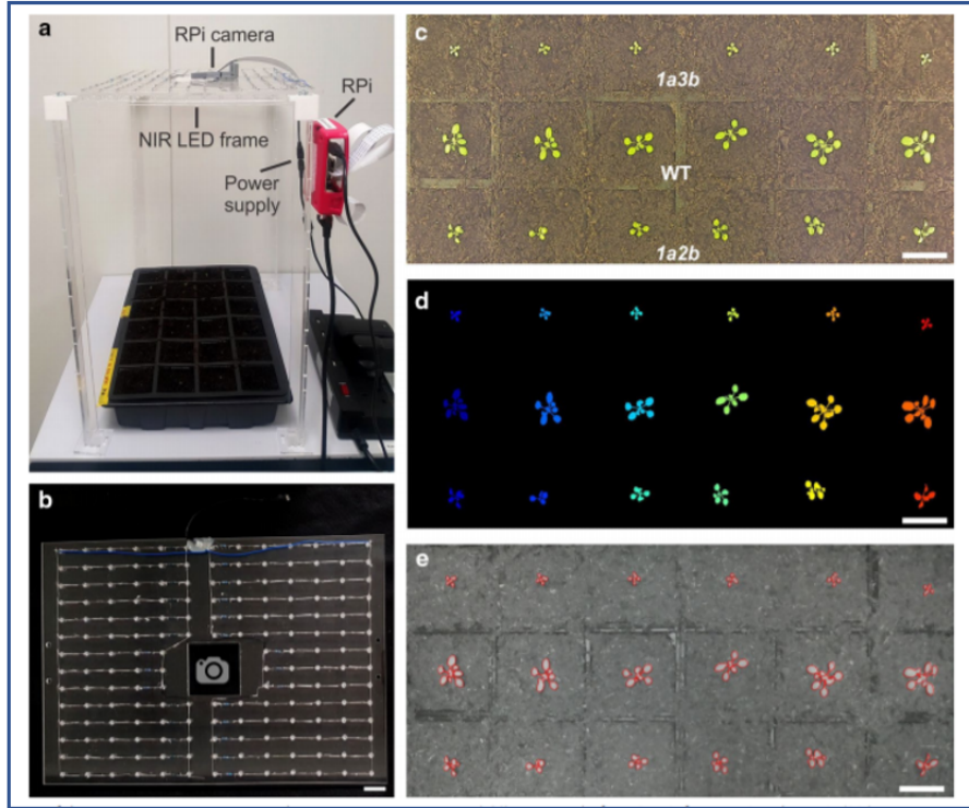
Figure 2.13 – (a) Image capturing system includes a NIR LED frame, and a NoIR RPi camera mounted to a Raspberry Pi mini-computer. (b) The NIR LED frame consists of 173 NIR LEDs arranged in parallel circuits. (c) plants under visible light (VIS) conditions. (d) Automated segmentation of plants. (e) Near-infrared (NIR) image of plants shown in (c) taken in the dark illuminated by NIR LEDs. Reproduced from [14].
