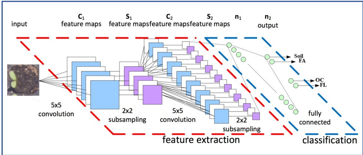
Figure 2.18 – CNN architecture designed to serve as baseline method for the independent classification of each frame of the time-lapses into one of the three stages of plant growth plus soil (Soil, FA, OC, and FL) without any prior temporal order information.
