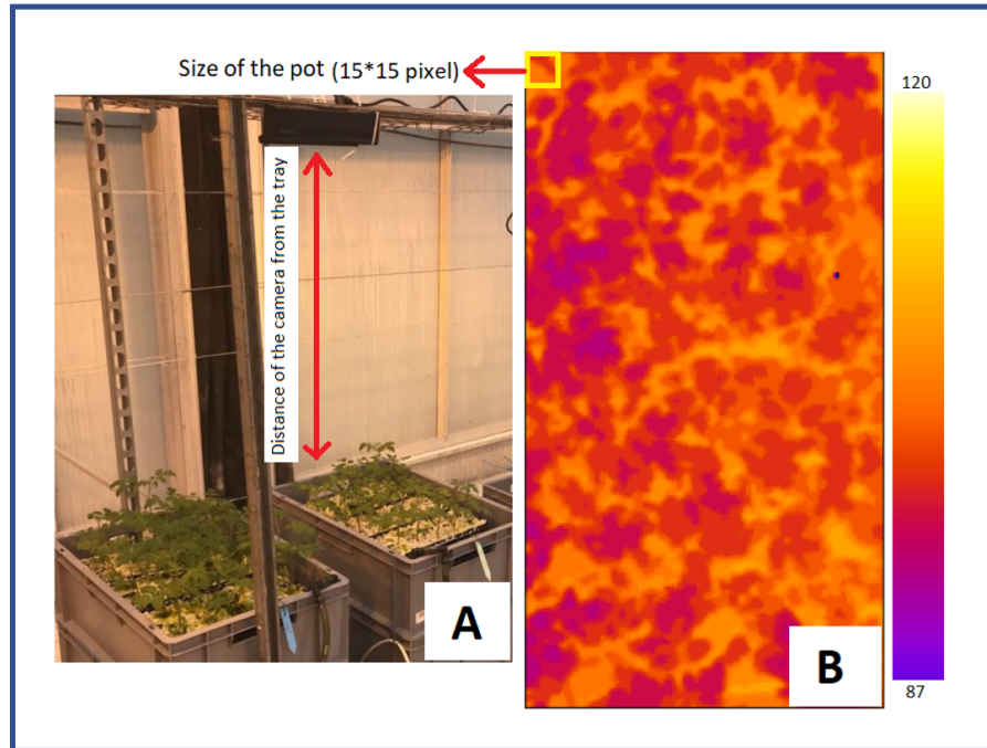
Figure 2.24 – Panel A, view of the image acquisition system. Panel B, colored depth map with look-up Table « fire ». The levels are indicated in cm.
