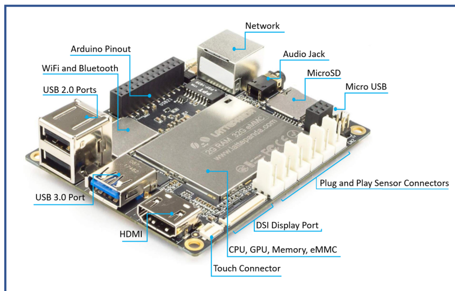
Figure 2.2 – LattePanda - mini-computer used in seedling growth monitoring in our work on canopy observation scale.
