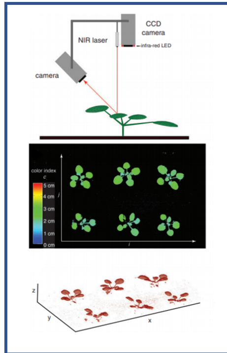
Figure 2.11 – Laser scanner and charged coupled device (CCD) camera mounted on the imaging unit in the Scanalyzer HTS phenotyping device and 2.5D height-scaled image in addition to the 3D point cloud computed from the recorded 2.5D image. Reproduced from [40].
