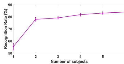
Figure 2. Dependency on the number of training subjects for cross-subject training (LBP features + SVM classifier).
