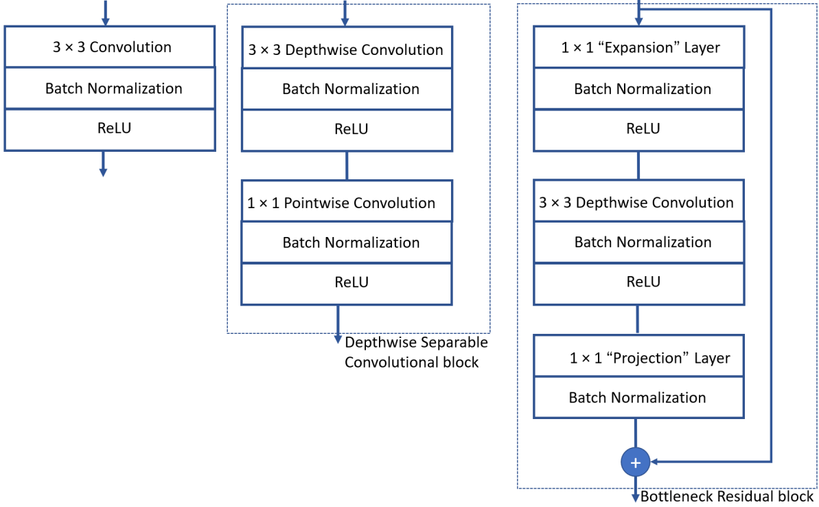
Figure 3.25 – Left: Standard convolutional network architecture with batch normalization and non-linearity. Middle: Depthwise Separable convolutions with Depthwise and Pointwise layers followed by batch normalization and non-linearity. Right: Expansion block consists of expansion layer with batch normalization and non-linearity followed by the depthwise block and the pointwise block including the projection layer and normalization and the residual connection.
