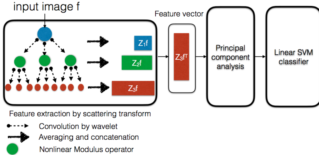
Figure 3.21 – Schematic layout of the weed/plant classifier based on the scattering transform with three layers. The feature vector transmitted to the principal component analysis (PCA) step consists in the scatter vector Z_m f of the last layer of Eq. (3.17) after transposition.
