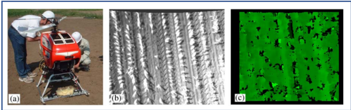
Figure 2.5 – (a) Helicopter-mounted stereo-vision system; (b) acquired crop image; (c) resulting disparity image. Reproduced from [23].
