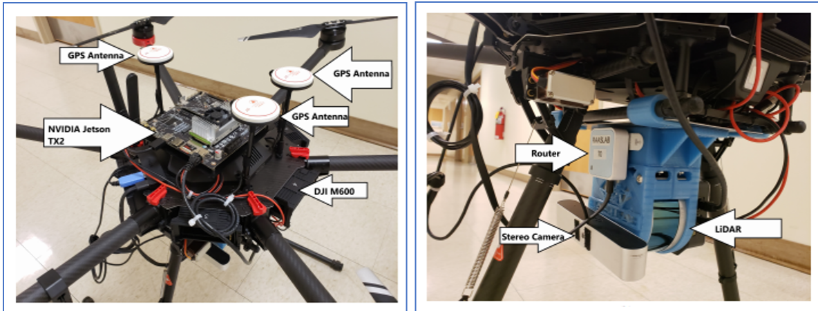
Figure 2.6 – UAV platform with selected sensors connected to the NVIDIA Jetson TX2 SBC on-top and beneath. Reproduced from [24].
