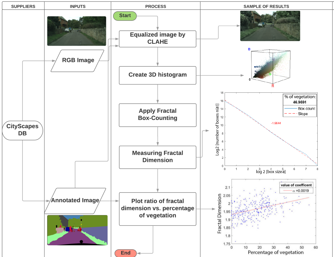
Figure 7. Image processing pipeline for the impact of vegetation in the color domain. CityScapes DB [30] corresponds to available dataset shows in Fig. 1. All images of CityScapes dataset are processed and batched city by city.
