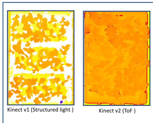
Figure 2.4 – Comparison of the depth map generated by the structured light sensor (Kinect v.1) and the ToF sensor (Kinect v.2).
