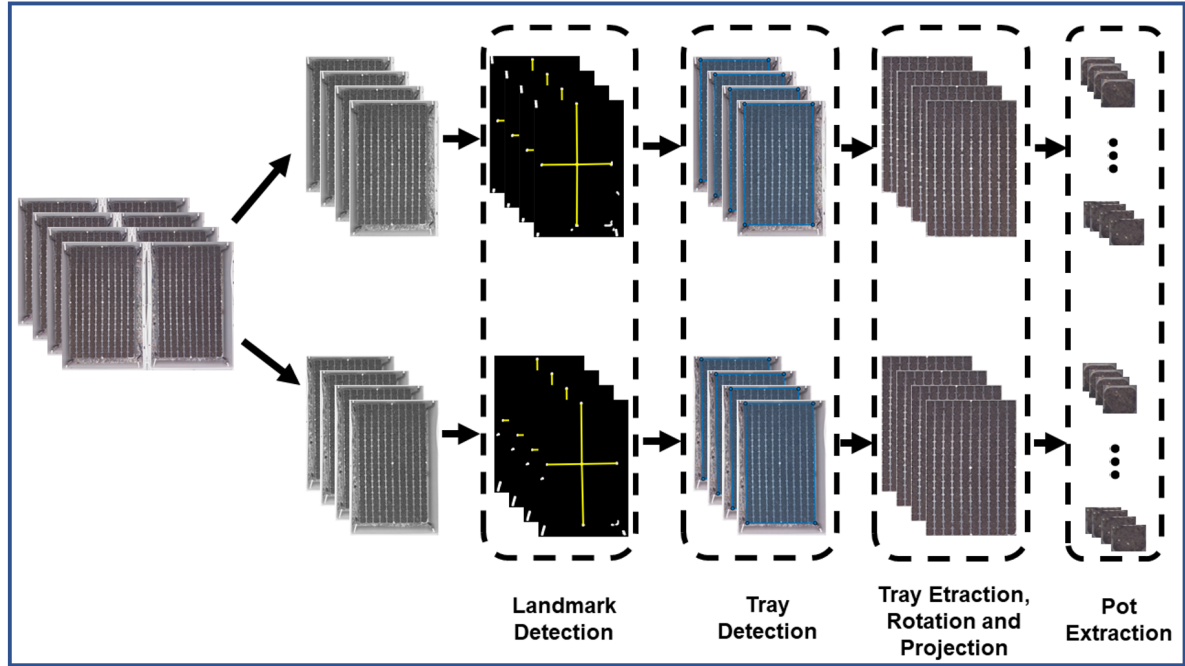
Figure 2.17 – Pot extraction workflow.
