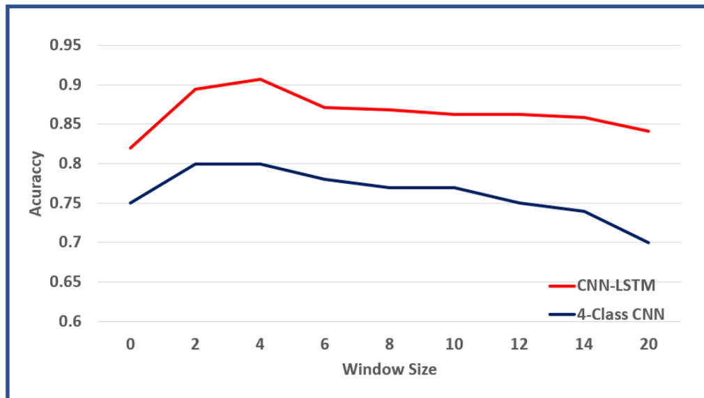
Figure 2.22 – Classification accuracy as a function of denoising windows size.
