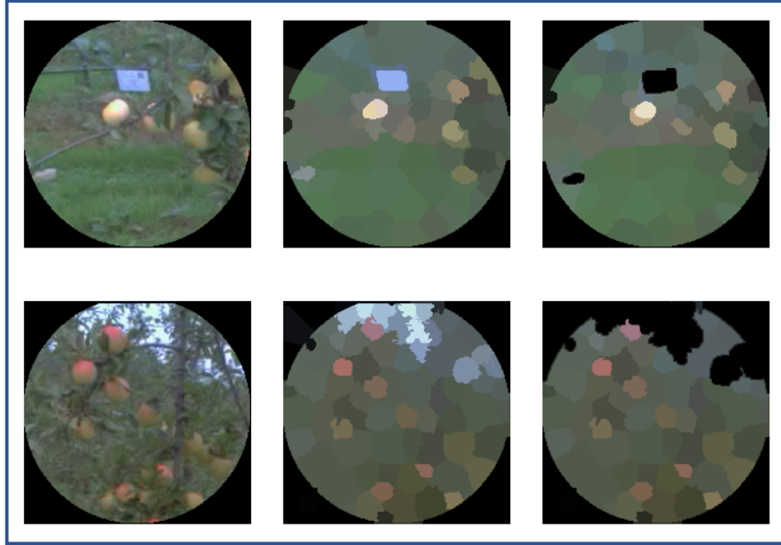
Figure 3.10 – Color thresholding to remove blueish color belonging to the sky or blue tree-labels on superpixel segmented attention areas. Each row represents from left to right: the attention area, superpixel segmented attention area, and the thresholded one, respectively.
