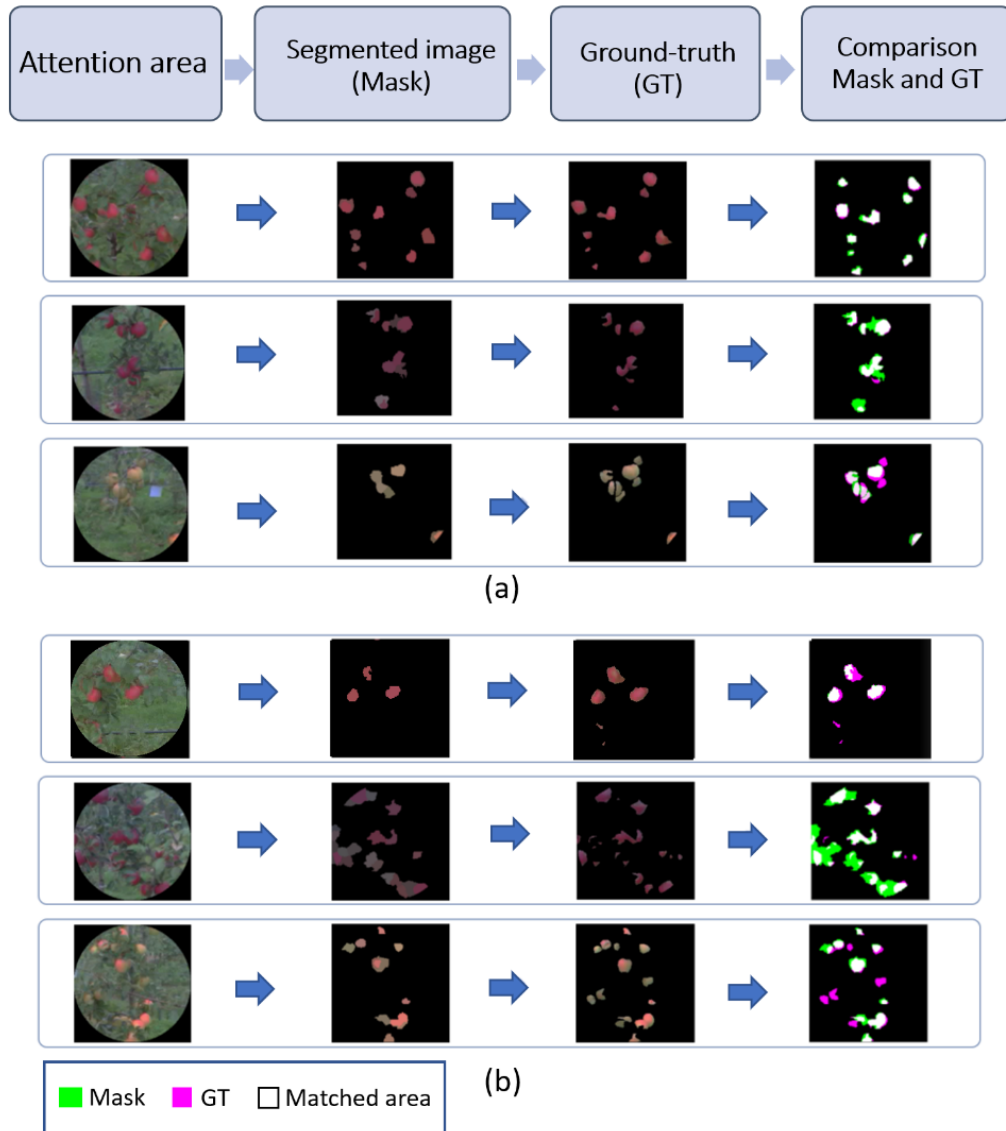
Figure 3.14 – Qualitative assessment of results. From left to right, an example of the attention area captured by eye-tracking, automatic annotation obtained from the proposed image processing pipeline of Fig. 3.9, ground-truth manually recorded, and comparison of manual ground-truth and automatic segmentation. (a) provides examples of good performance; (b) shows some challenging conditions where more errors are found (missed detection, false detection).
