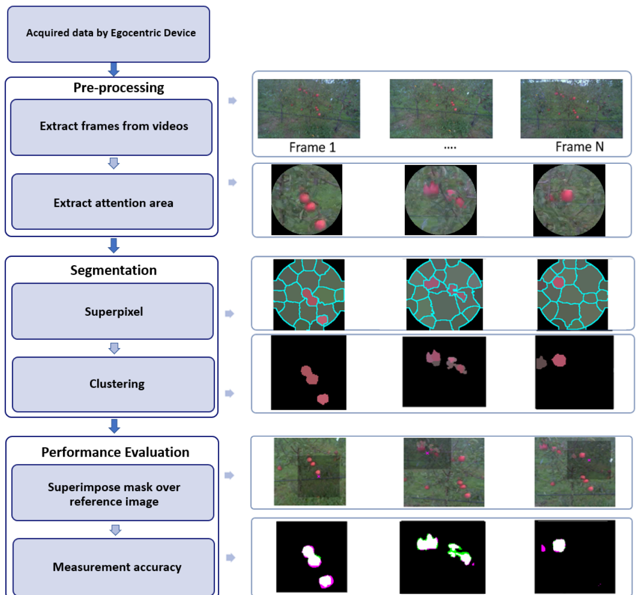
Figure 3.9 – Three steps image processing pipeline proposed to automatically segment apples from attention area captured with egocentric devices.
