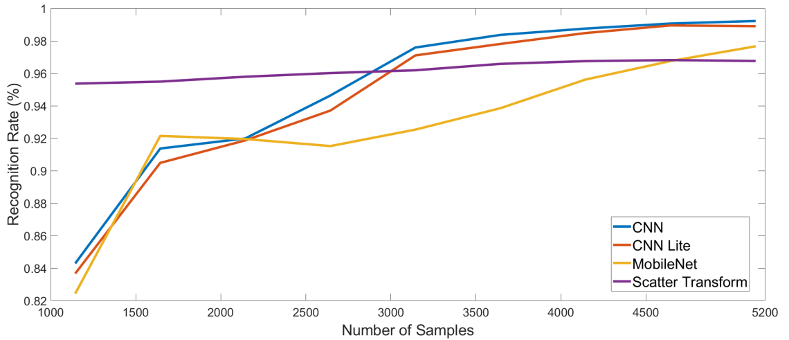
Figure 3.26 – Comparison of the recognition accuracy between scatter transform and baseline CNN plus CNNLite and MobileNet architecture when the number of samples increases.
