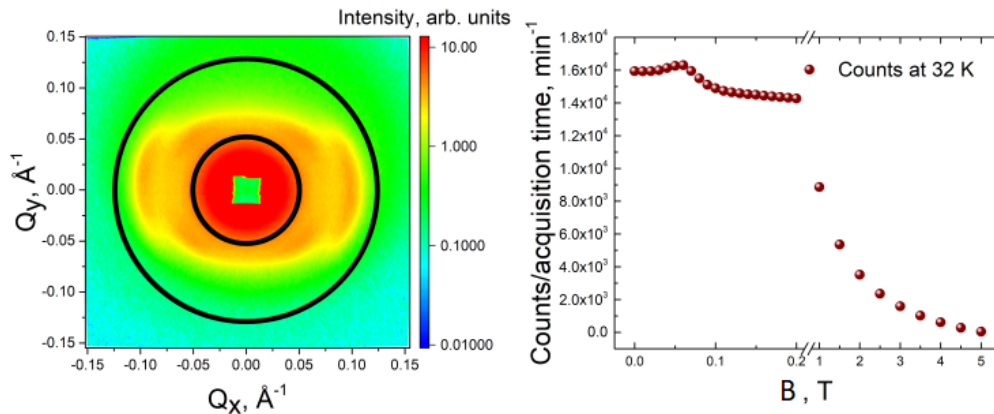
Figure 3.31: Left: SANS pattern for the ordered \text{Co}_5\text{TeO}_8 polymorph collected at 32 K and B = 0.08 \text{ T} . Small and large rings represent R_{min} and R_{max} respectively. Right: the evolution of detector counts in the area of interest ( R_{min} > R > R_{max} ) as the function of the applied magnetic field ( \mathbf{B} \parallel q_x ) at 32 K.
