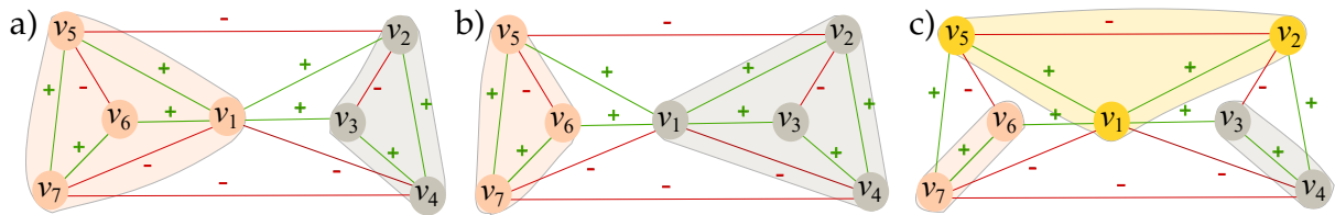
Figure 7.8: Three (out of 22) different optimal CC solutions obtained for the same 7-vertices signed graph: a) \mathcal{P}_a = \{\{v_1, v_5, v_6, v_7\}, \{v_2, v_3, v_4\}\} ; b) \mathcal{P}_b = \{\{v_5, v_6, v_7\}, \{v_1, v_2, v_3, v_4\}\} ; and c) \mathcal{P}_c = \{\{v_1, v_2, v_5\}, \{v_6, v_7\}, \{v_3, v_4\}\} . Red and green lines represent negative and positive edges, respectively. The graph is complete, but for clarity, some negative edges between communities are intentionally omitted.
