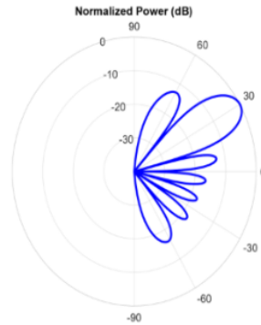
Figure 2.9: Phased array beam pattern.
