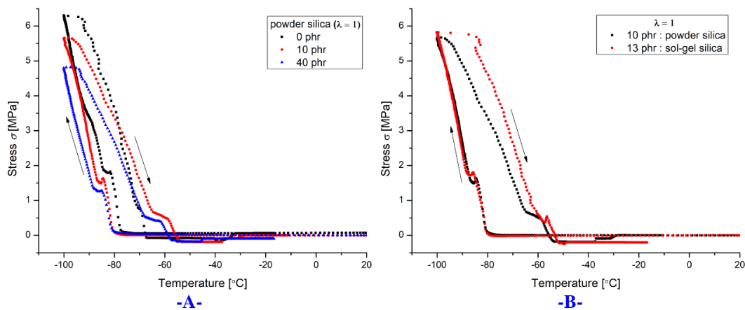
Figure 5.10 The thermoelastic properties of unstretched dog bone shape during cooling and heating: -A- different powder silica content; -B- different mixing method of silica.
