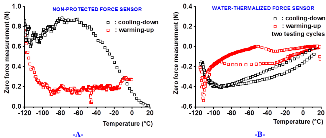
Figure 5.3 Drift of the sensor in absence of any loading during a cooling cycle.
