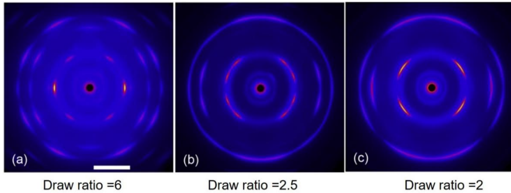
Figure 1.11 WAXD patterns [30] of cross-linked PDMS samples crystallized at -90\text{ }^{\circ}\text{C} (scale bar = 10\text{ nm}^{-1} ). Stretching direction is vertical. \text{Cu K}\alpha radiation was used as the X-ray source.
