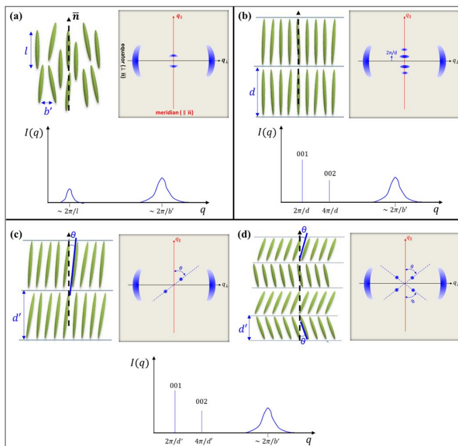
Figure 7.4 Schematic representation of molecular arrangements and their corresponding X-ray scattering patterns, diffraction profiles from aligned samples of different LC phases: (a) Nematic, (b) Smectic A, and (c, d) Smectic C phase in different alignment. \bar{n} refers to the director of molecules and \theta is the tilted angle between the director and the layer normal, b' is the average lateral distance between two neighbor liquid crystal molecules.
