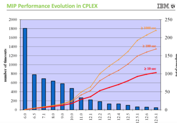
FIGURE 2.7 – Mixed Integer Programming Evolution in Cplex [Lin17].
