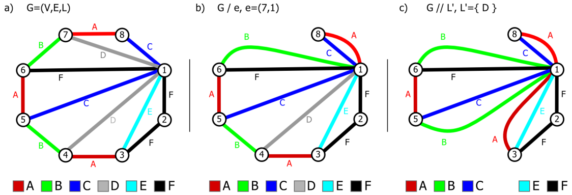
Figure 3.1: Illustration of the concepts of edge and label contraction. (a) the ELG G = (V, E, L) . (b) the graph G after the contraction of the edge e = (7, 1) , and (c) the graph G after the contraction of the label D
