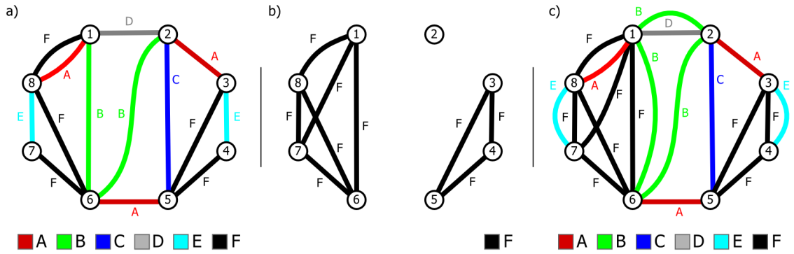
Figure 3.6: Example of transitive and chromatic closures. (a) The edge-labeled graph G = (V, E, L) . (b) The transitive closure of the label F . (c) the chromatic closure of the graph G .
