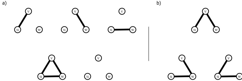
Figure 9.2: Allowed and forbidden configurations according to the P_3 elimination inequalities. (a) The allowed and (b) the forbidden configurations
