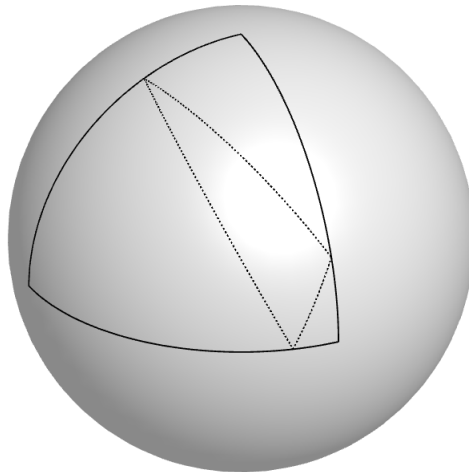
Figure 6: An example of 3-reflective billiard on the sphere presented by Barychnikov. The outer triangle is boundary of the billiard, the interior triangle in dotted lines is an orbit. Two vertices of the orbit can be moved arbitrarily without changing its periodicity.
