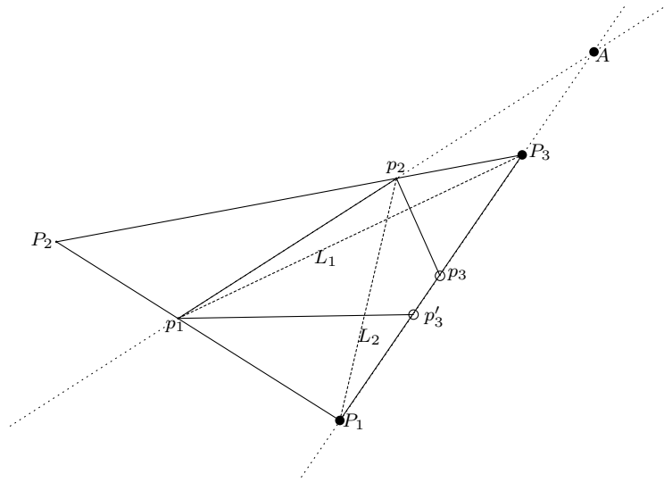
Figure 3.5: As in the proof of Proposition 3.10, both quadruples of points (p_2, A, P_1, P_3) and (p_1, A, P_2, P_3) are harmonic, hence necessarily p_2 = p_1 .
