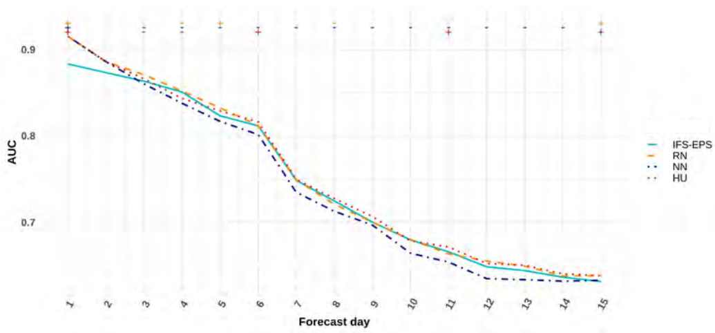
703 FIG. 8. AUC of 2-meter temperature forecasts above 15°C, computed for the 11 sites over the period 01/06/2018- 704 31/05/2019, as a function of forecast day. Results for the random 12-member IFS-EPS and the three seamless 705 ensembles are overlaid. Top + (resp. -) signs indicate that the performance of a seamless ensemble is statistically 706 better (resp. worse) than the IFS-EPS performance, according to the Wilcoxon test.
