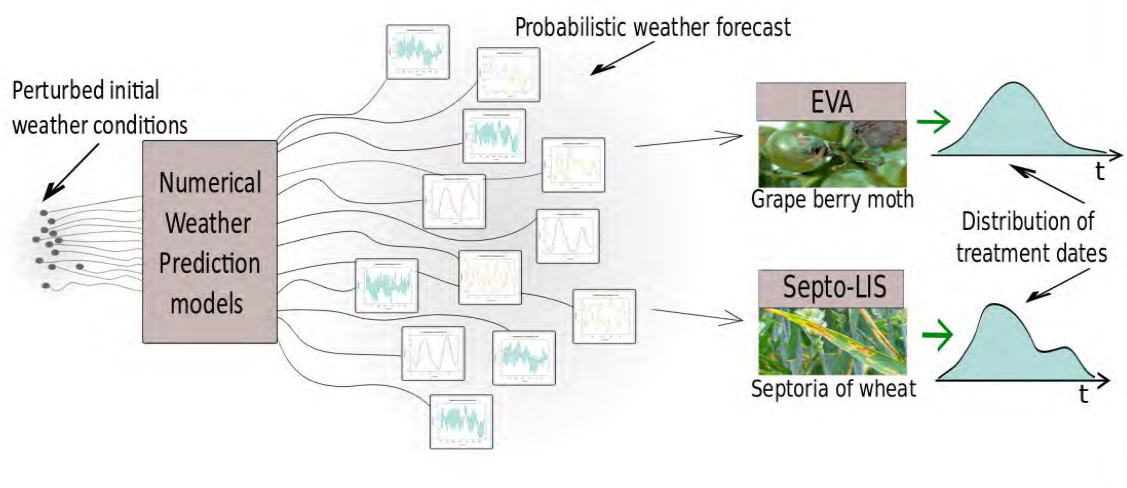
Figure 3: Ensemble prediction and propagation of weather forecast uncertainties through the both cases wheat septoria and grape berry moth.
