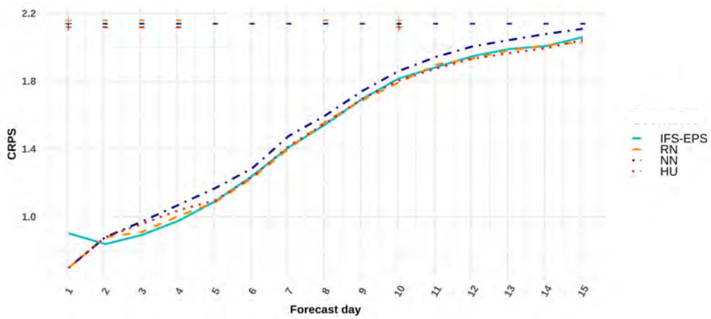
699 FIG. 7. CRPS of 2-meter temperature forecasts computed for the 11 sites over the period 01/06/2018- 700 31/05/2019, as a function of forecast day. Results for the random 12-member IFS-EPS and the three seamless 701 ensembles are overlaid. Top + (resp. -) signs indicate that the performance of a seamless ensemble is statistically 702 better (resp. worse) than the IFS-EPS performance, according to the Wilcoxon test.
