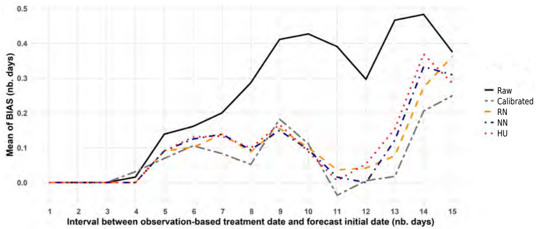
715 FIG. 11. Bias of the ensemble mean treatment date forecast, as a function of the time interval (in day) between 716 the observation-based date and the forecast starting date. Scores are averaged over the 8 vineyard sites and the 717 period of interest 01/04-19/09 for the years 2018 and 2019. Results from using raw IFS-EPS, calibrated IFS-EPS 718 and the three seamless ensemble forecasts are overlaid.
