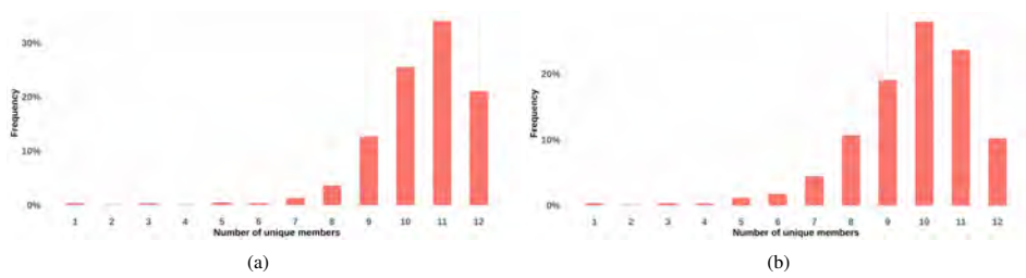
692 FIG. 5. Frequency histograms of the number of independent members in the NN ensembles, computed for the 693 11 sites over the period 01/06/2018-31/05/2019, (a) after the 48h-merging step and (b) after the 96h-merging 694 step.
