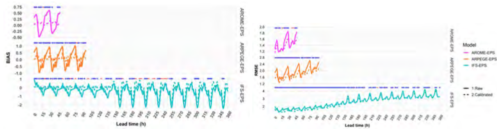
683 FIG. 3. Bias (left) and RMSE (right) of ensemble mean forecast for 2-meter temperature, as a function of 684 forecast lead time. Scores are computed for the 11 sites over the period 01/06/2018-31/05/2019 with raw (solid 685 line) and calibrated (dashed line) ensembles. Top: AROME-EPS, middle: ARPEGE-EPS and bottom: IFS-EPS. 686 Top + (resp. -) signs indicate that the performance of the calibrated ensemble is statistically better (resp. worse) 687 than the raw ensemble performance, according to the Wilcoxon test.
