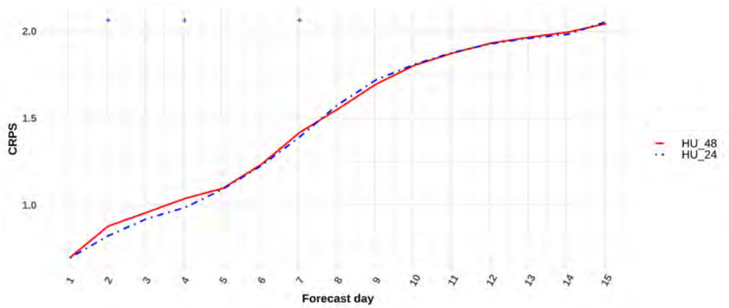
710 FIG. 10. CRPS of 2-meter temperature forecasts computed for the 11 sites over the period 01/06/2018- 711 31/05/2019, as a function of forecast day. Results are given for seamless HU ensembles with a first merging 712 at 24h (dashed-dotted line) and 48h (solid line). Top + (resp. -) signs indicate that the performance of the 713 24h-merging is statistically better (resp. worse) than the performance of the 48h-merging, according to the 714 Wilcoxon test.
