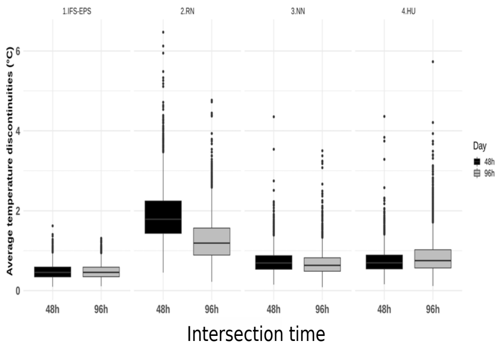
695 FIG. 6. Boxplots of absolute temperature forecast differences, averaged over ensemble members, between lead 696 times 48 and 49h (in black) and lead times 96 and 97h (in gray), computed for the 11 sites over the period 697 01/06/2018-31/05/2019. These forecast differences are presented, from left to right, for IFS-EPS members and 698 for the seamless RN, NN and HU ensemble members.
