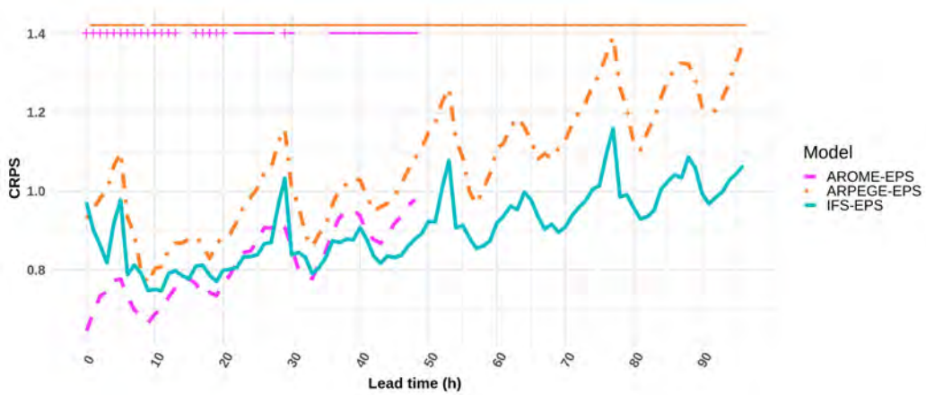
688 FIG. 4. CRPS of 2-meter temperature forecasts as a function of forecast lead time. Scores are computed for 689 the 11 sites over the period 01/06/2018-31/05/2019 for the three calibrated EPS. Top + (resp. -) signs indicate 690 that the performance of the AROME-EPS and the ARPEGE-EPS is statistically better (resp. worse) than the 691 IFS-EPS performance, according to the Wilcoxon test.
