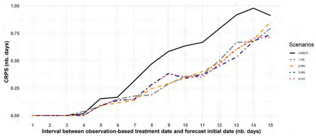
719 FIG. 12. CRPS for the forecast treatment date, as a function of the time interval (in day) between the 720 observation-based date and the forecast starting date. Scores are averaged over the 8 vineyard sites and the period 721 of interest 01/04-19/09 for the years 2018 and 2019. Results from using raw IFS-EPS, calibrated IFS-EPS and 722 the three seamless forecasts are overlaid.
