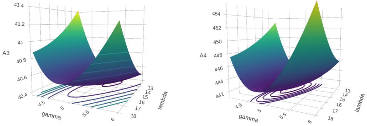
Figure 3.2: Shapes of the surfaces defined by the functions A_3(\cdot, \cdot) and A_4(\cdot, \cdot) , see Lemma 14.
