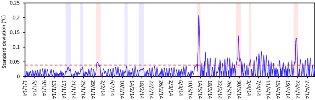
Figure 5- 4: Standard deviation of temperature at 0.5 meter, the dashed red line represents the threshold parameter.
