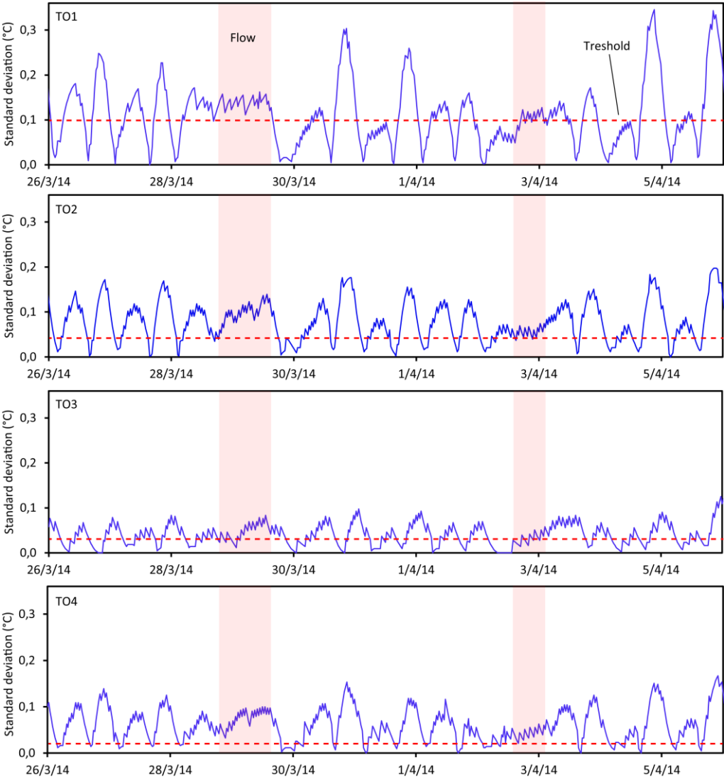
Figure 5- 3: MSD of temperature measured at the four probes installed across the wadi during the period between 26/03/2014 and 06/04/2014.
