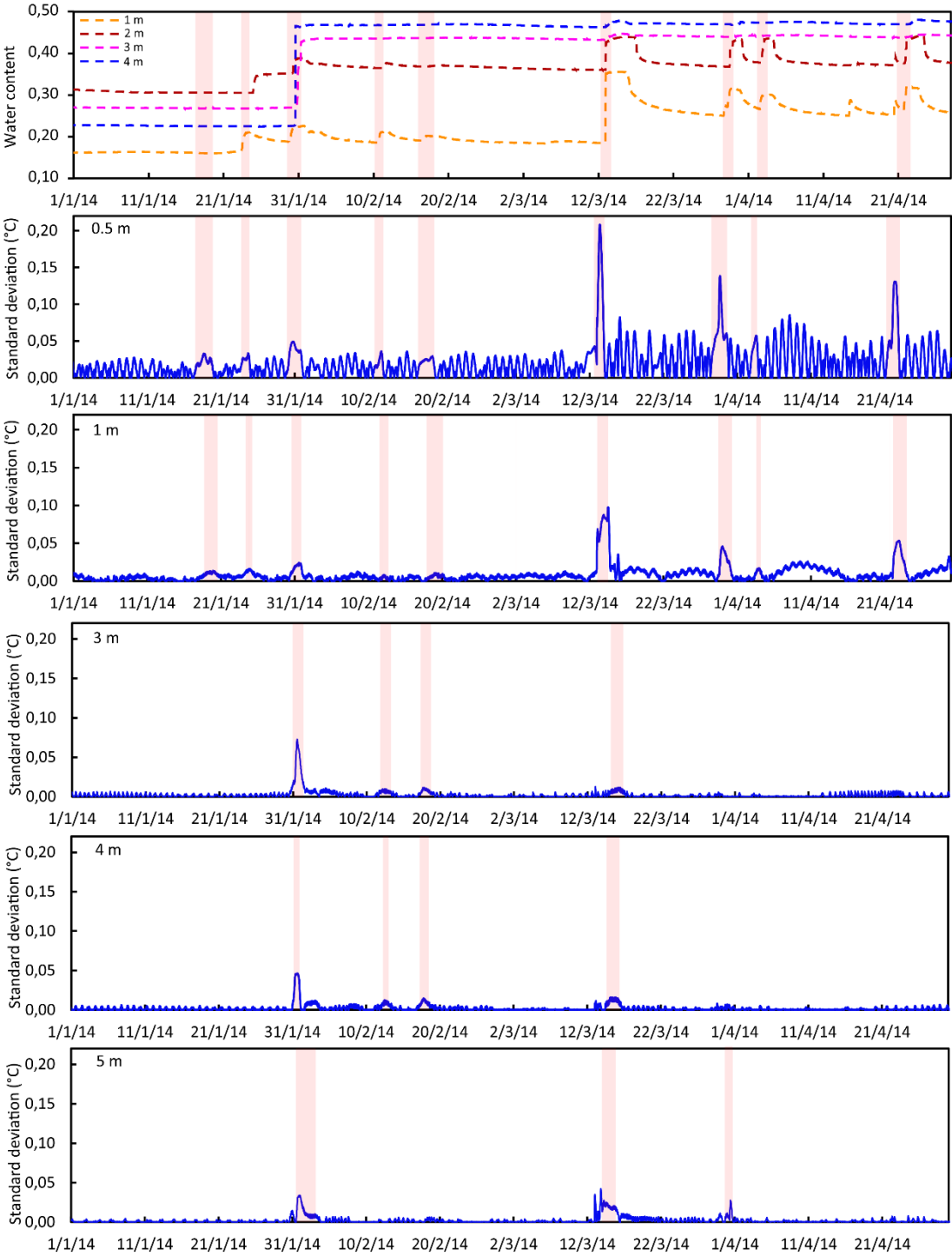
Figure 5- 8: Standard deviation of temperature data at multiple depths (0.5, 1, 3, 4 and 5 meters) coupled with water content data at multiple depths (1, 2, 3 and 4 meters).
