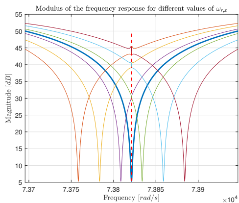
(a) |F_{\omega_{r,x}}(e^{j\omega T_s})|
