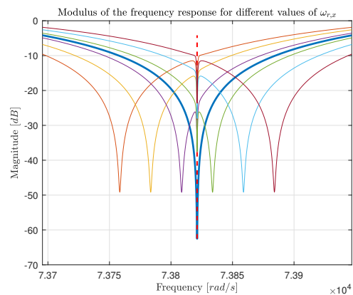
(b) |S_{\omega_{r,x}}(e^{j\omega T_s})|
