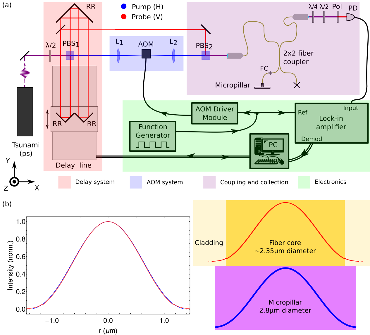
Figure 5.9: (a) Optical setup for TDBS measurements of fiber-integrated micropillars. Picosecond pulses pass by a half waveplate ( \lambda/2 ) and a polarizing beam splitter ( \text{PBS}_1 ) where two beams of pulses are generated for a pump and probe detection scheme. Then, the probe enters an optical delay system. The pump is focused through an optoacoustic modulator system where an 800 kHz modulation is imprinted on it. Both pump and probe beam are coupled to the same single-mode fiber where their spatial modes are cleaned. By controlling the delay between pump and probe and demodulating the effects of the pump on the sample at the instant the probe is reflected from it, we are able to resolve the Brillouin scattered signal in time. A quarter, a half waveplate and a polarizer are used at the probe collection to extinguish the pump pulses in a cross polarization scheme. (b) Left: Intensity profile of single-mode fiber and 2.8 \mu\text{m} diameter micropillar plotted in red and blue, respectively. The core refractive index and radius were found by fitting these two curves while maintaining the cladding refractive index fixed at 1.450. Right: Schematic showing the micropillar against the single-mode fiber. The intensity profile of fiber and pillar are plotted in red and blue, respectively.
