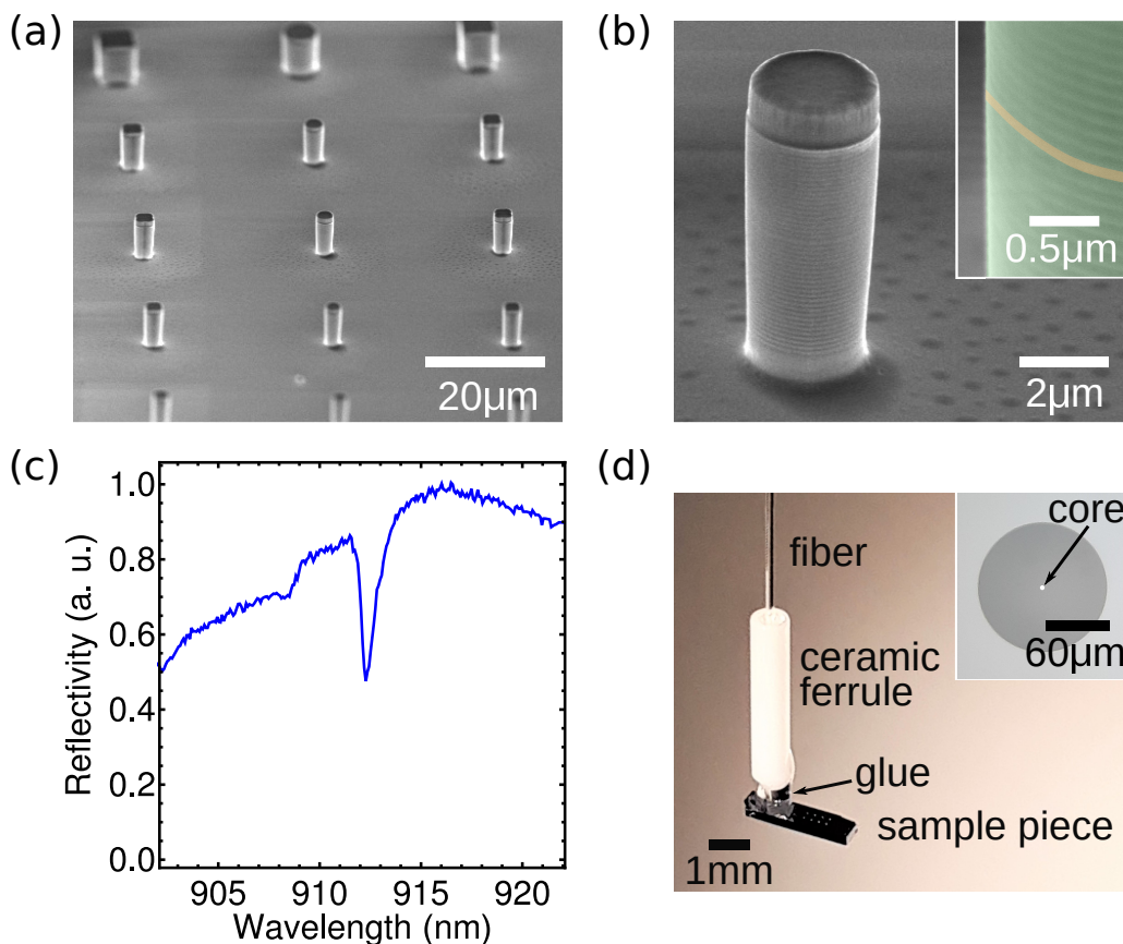
Figure 5.8: (a) SEM image of an array of pillars present in the sample piece used for fiber integration. (b) SEM image of a 2.8 \mu\text{m} diameter micropillar. Inset shows a zoom near the center of the multilayer structure. Transparency and false colors are used to enhance the contrast between layers. (c) Reflectivity spectrum of the fiber-integrated micropillar. The micropillar optical's mode appears as a reflectivity dip around 912.1 nm. (d) Image of the final device. Inset presents a microscopy image of the single-mode fiber where the core can be distinguished.
