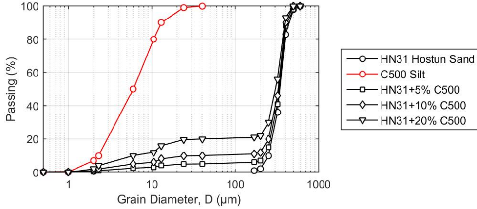
Figure 3.2: Grain size distribution of HN31 Hostun-RF sand, Silica C500 silt and various mixtures (5, 10 and 20%)
