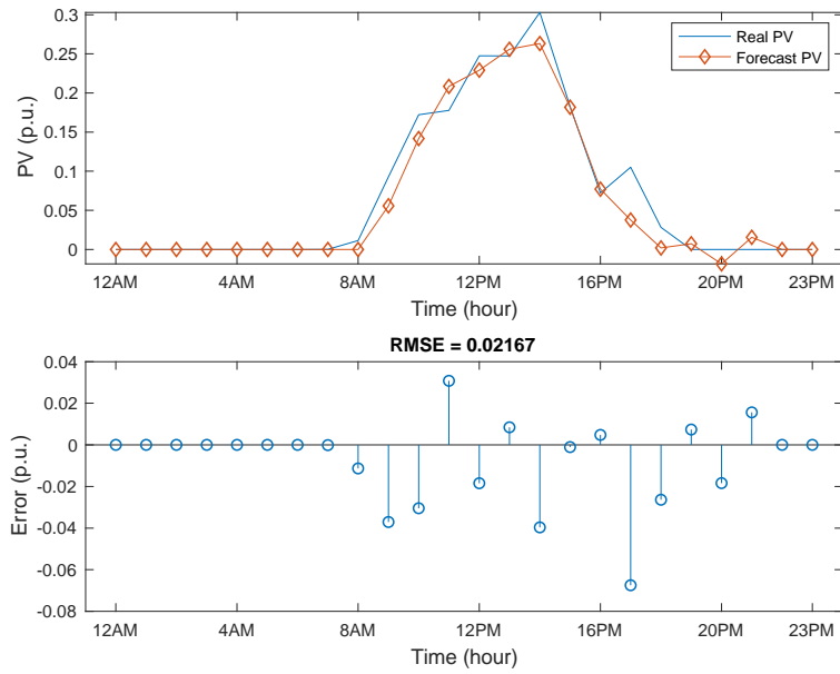
(b) Hourly PV power forecast and forecast errors
