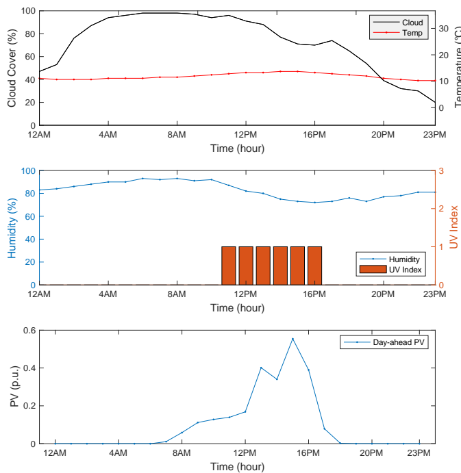
(a) Inputs: Day-ahead forecasted cloud cover and temperature, day-ahead sensed PV power
