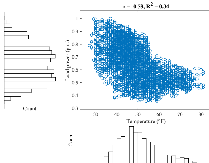
Fig. 2-6 The correlation between temperature and load power
