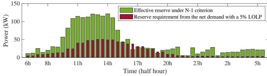
(b) Comparison of effective reserve and reserve requirement
