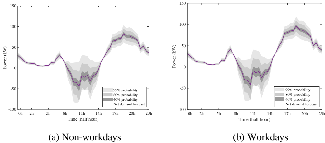
Fig. 5-38 pdf -based expected net demand in spring
