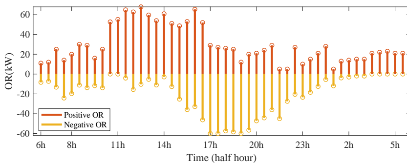
Fig. 3-27 Effective OR corresponding to the expected worst case of PV generation.
