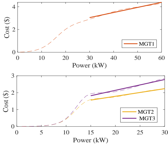
Fig. 3-31 Linearization of the nonconvex cost function of studied three MGTs
