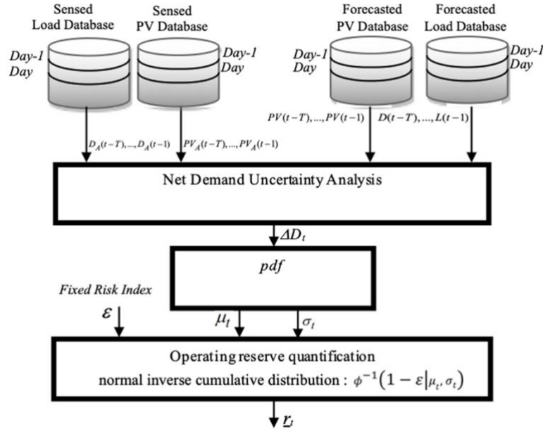
Fig. 5-7 Deterministic operational planning with combination of storage strategy regarding reserve allocation
