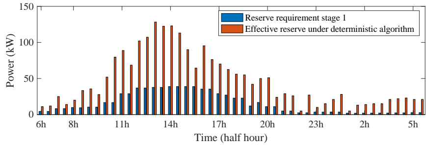
(b) Obtained effective reserve with a LOLP \leq 5\% in strategy 2
