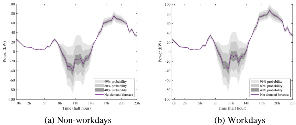
Fig. 5-39 pdf -based expected net demand in summer
