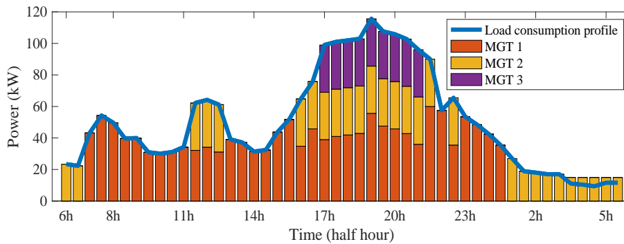
Fig. 3-14 Generation planning without PV
