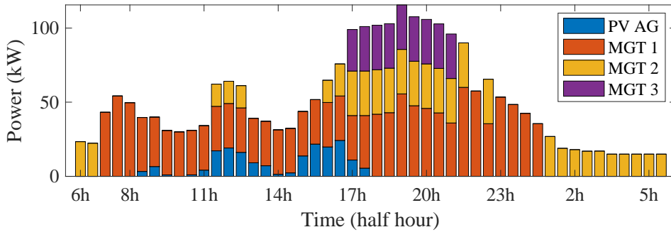
Fig. 3-17 Generation planning under N-1 criterion
