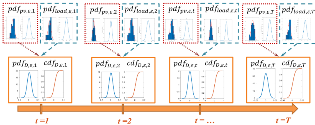
Fig. 3-3 pdf of net demand forecast errors from historic database of PV and load demand forecasting errors.
