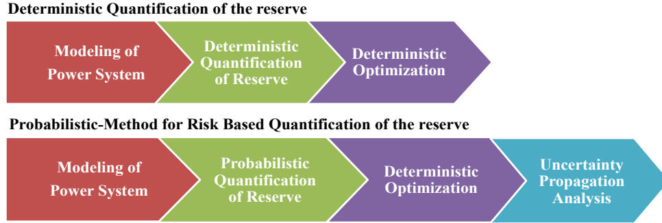
Fig. 1-14 DUC schemes of deterministic optimization without and with probabilistic reserve quantification
