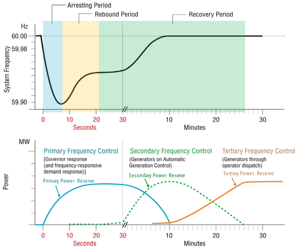
Fig. 3-2 Sequential actions of primary, secondary, and tertiary frequency controls following the sudden loss of generation [179].
