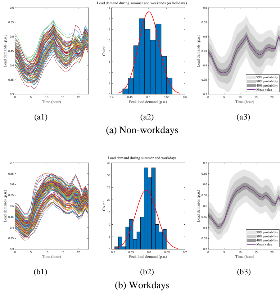
Fig. 5-31 Probabilistic analysis and pdf of load demand in summer
