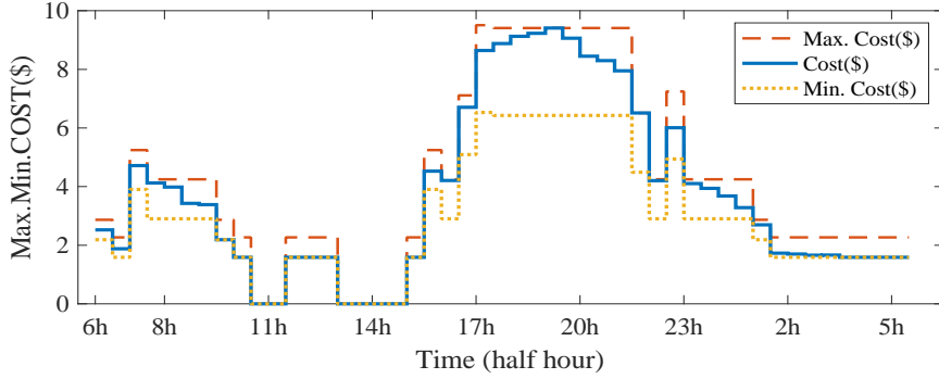
Fig. 3-23 Expected, maximum and minimum operational costs
