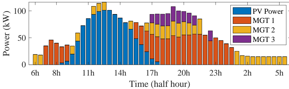
Fig. 3-20 Optimal day-ahead generation scheduling with risk-based deterministic optimization.
