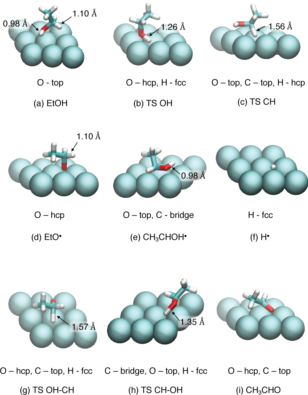
Figure 4.7. Structures of reaction species for EtOH dehydrogenation on Co(0001) facet: (a) EtOH, (b) TS OH, (c) TS CH, (d) EtO • , (e) CH 3 CHOH • , (f) H • , (g) TS OH-CH, (h) TS CH-OH, (i) CH 3 CHO. Element coding on picture is as follow: light blue (cyan) balls – Co, light blue (cyan) sticks – C, red sticks – O and white sticks – H. The OH and CH bond lengths are given on the pictures (in Å).
