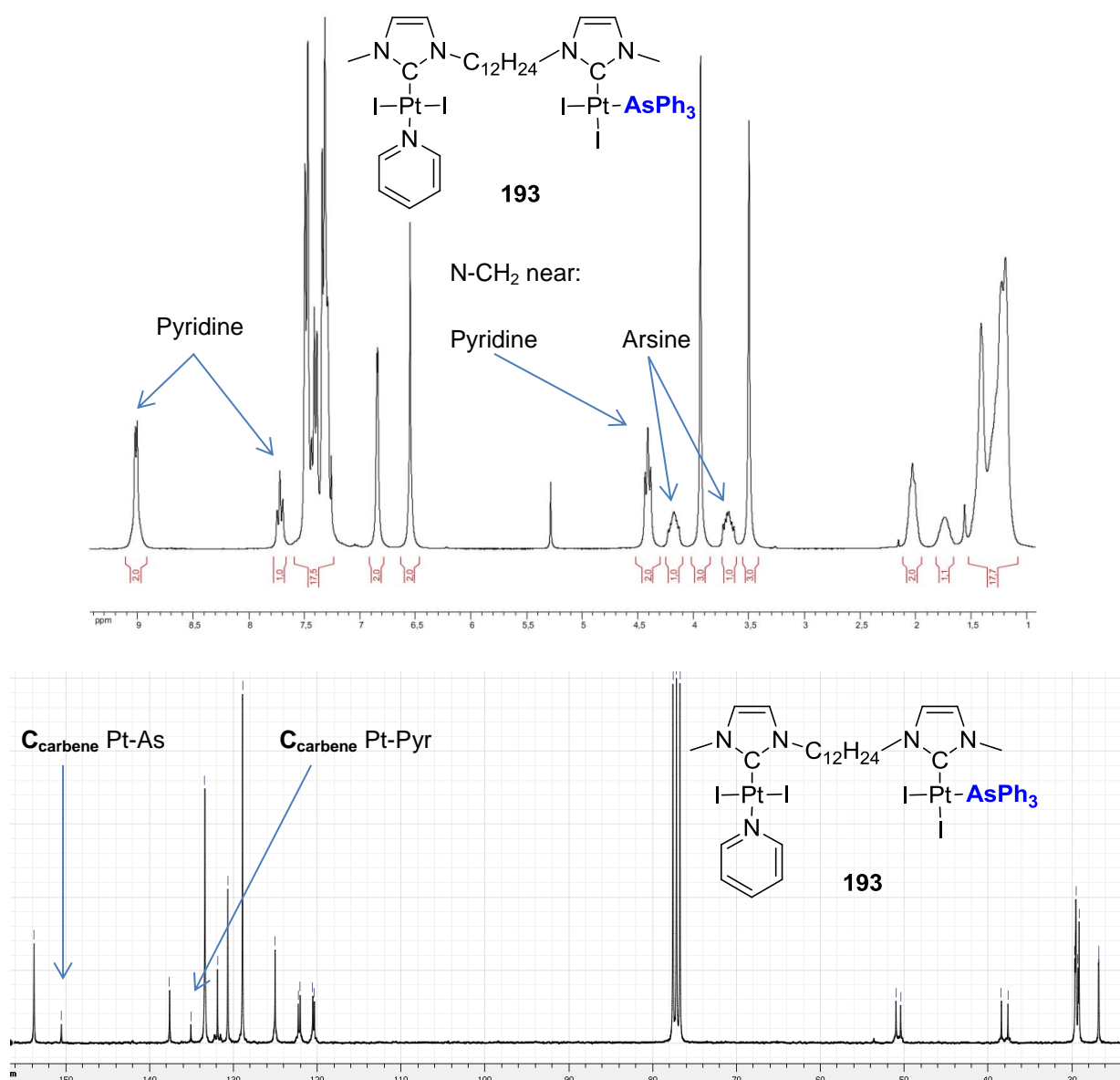
Figure 150: ^1\text{H} and ^{13}\text{C} -NMR spectra of a binuclear NHC complex 193 with pyridine and arsine ligands
