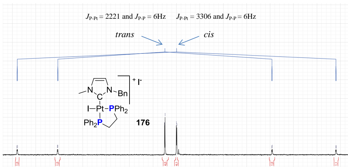
Figure 137: NMR ^{31}\text{P} spectrum of [(\text{NHC})\text{Pt}(\text{dppe})]\text{I} complex 176 : evidence of cis and trans P
