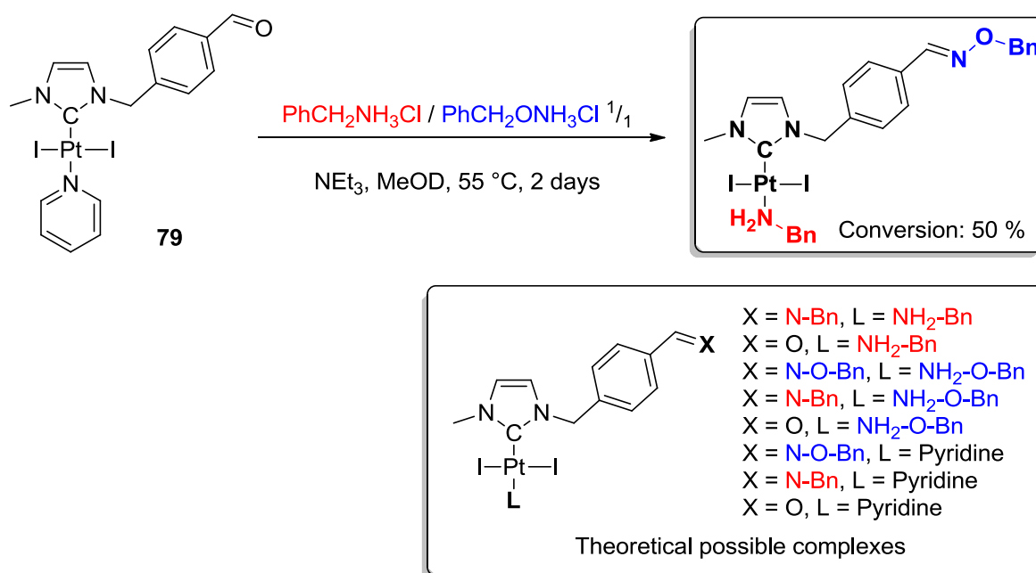
Figure 177: Competition experiment between amine and oxime on a [(pyridine)Pt 2 (NHC-benzaldehyde)] complex: relative selectivity of oxime formation and ligand exchange
