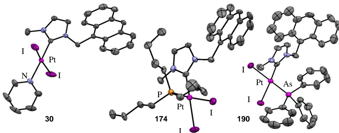
Figure 145: (Anthracene-NHC)Pt(II)-ligand complexes: 30 (pyr), 174 \text{P}(n\text{Bu})_3 and 190 ( \text{AsPh}_3 )
