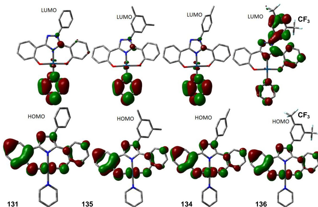
Figure 100: Locations of LUMOs and HOMOs on the (O ^ N ^ O) platinum complexes: influence of the CF 3 group on the LUMO
