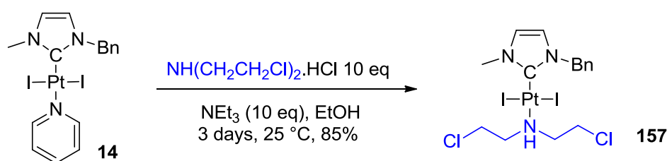
Figure 104: Synthesis of nitrogen mustard platinum derivative 157
