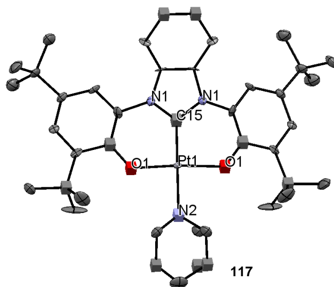
Figure 82: Preliminary molecular structure of [(O^{\wedge}C^{\wedge}O)Pt(\text{pyridine})] 117 obtained by X-ray diffraction
