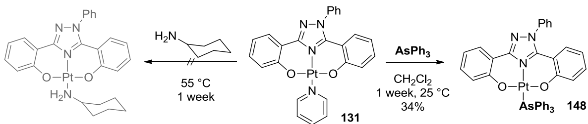
Figure 90: Ligand exchange reactivity of [(O^*N^*O)Pt(pyridine)]
