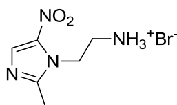
2-(2-methyl-5-nitro-1H-imidazol-1-yl)ethanaminium bromide
