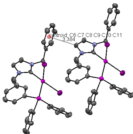
Figure 141: Solid-state \pi\text{-}\pi interaction established between a phenyl ring and imidazole ring two stibine complexes 179
