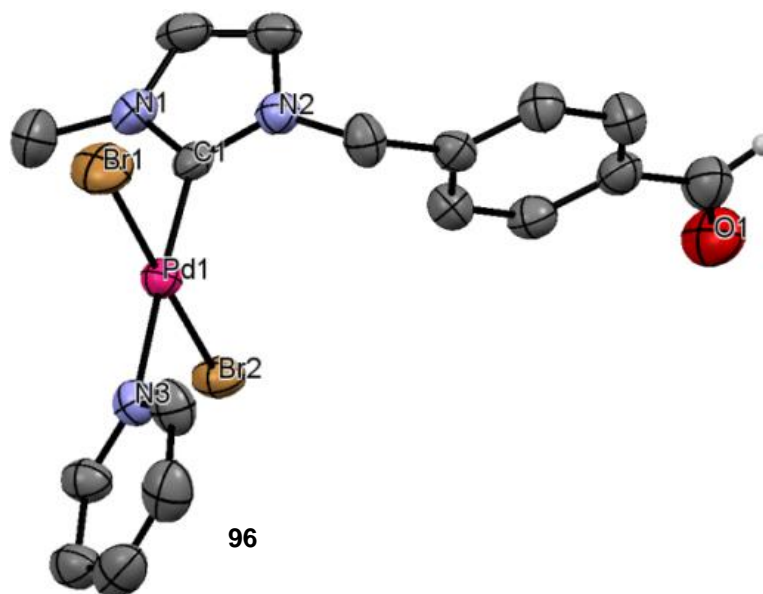
Figure 72: X-ray structure of [(Benzaldehyde-NHC)PdBr 2 (pyr)] complex 96 . Selected bond lengths (Å) and angles (°): C-Pd:1.961; Pd-Br: 2.443, 2.423; Pd-N: 2.100; C-Pd-N: 177.04; N-C-Pd-I: 87.87, 90.00.
