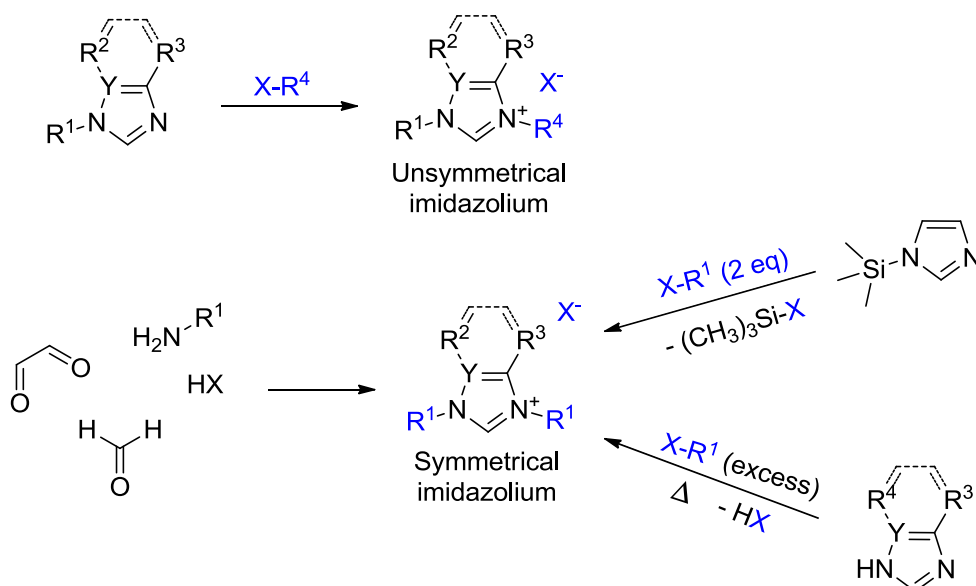
Figure 200: Imidazolium synthesis
