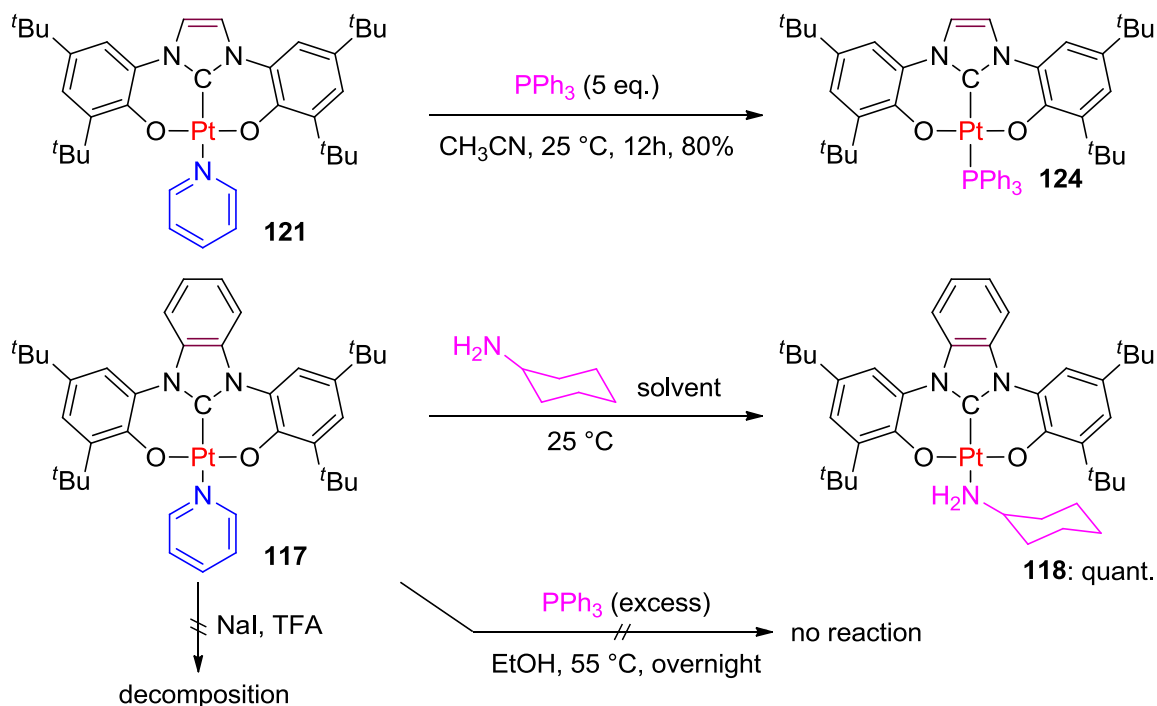
Figure 83: Reactivity of the (O ^ C ^ O) complexes towards neutral ligands or acids 326
