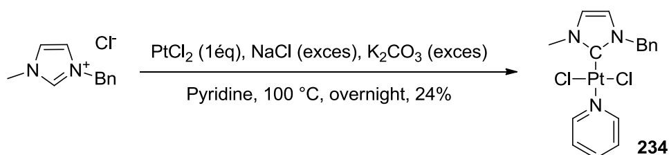
Figure 190: Synthesis of [(NHC)PtCl 2 (pyridine)] from the imidazolium chloride
