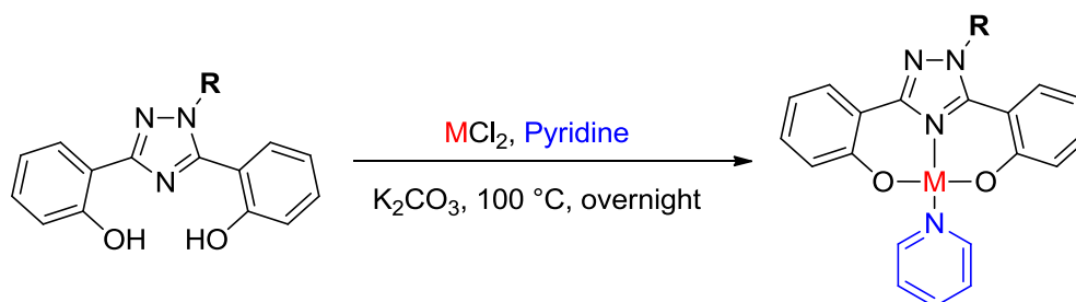
Figure 86: Synthesis of [(O^{\wedge}N^{\wedge}O)M(\text{pyr})] complexes (M = Pt or Pd)
