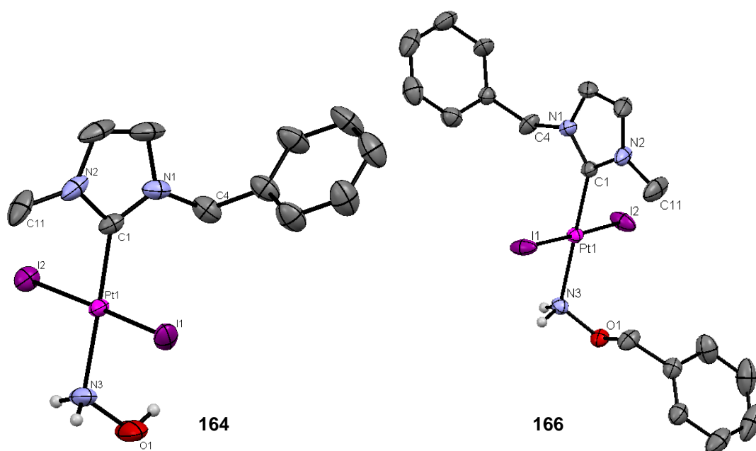
Figure 112: X-ray diffraction structures of [(NHC)PtI 2 (NH 2 OH)] 164 and [(NHC)PtI 2 (benzylhydroxylamine)] 166
