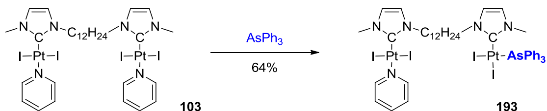
Figure 149: Binuclear NHC complex 198 with pyridine and arsine ligands
