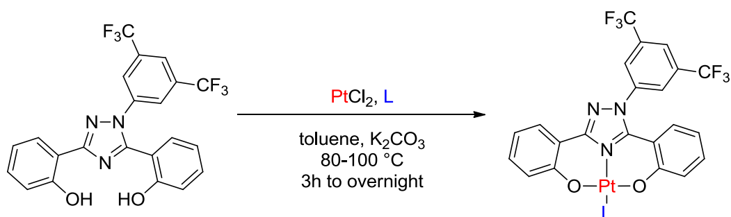
Figure 88: Synthesis of [(O^{\wedge}N^{\wedge}O)Pt(L)] complexes: variation of the monodentate L ligand
