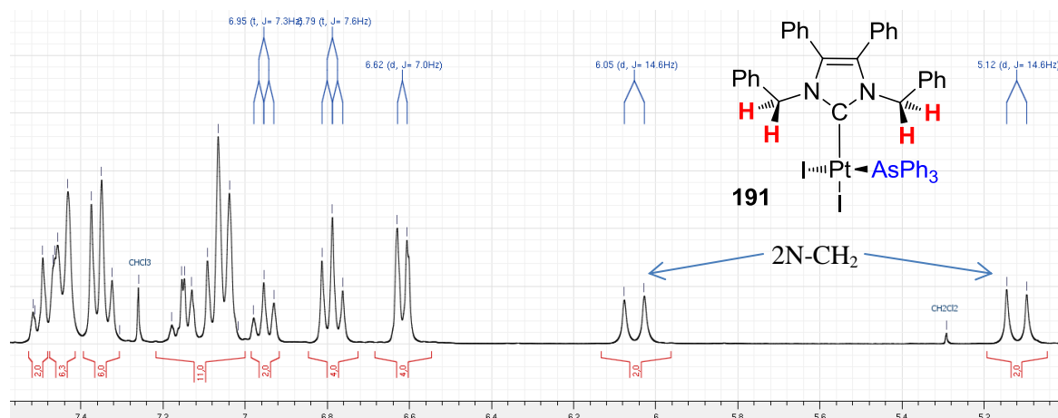
Figure 144: ^1\text{H-NMR} spectrum of a 1,3-dibenzyl-4,5-diphenyl-imidazol-2-ylidene-Pt (II)-arsine complex 191 : N- \text{CH}_2 disymmetrisation
