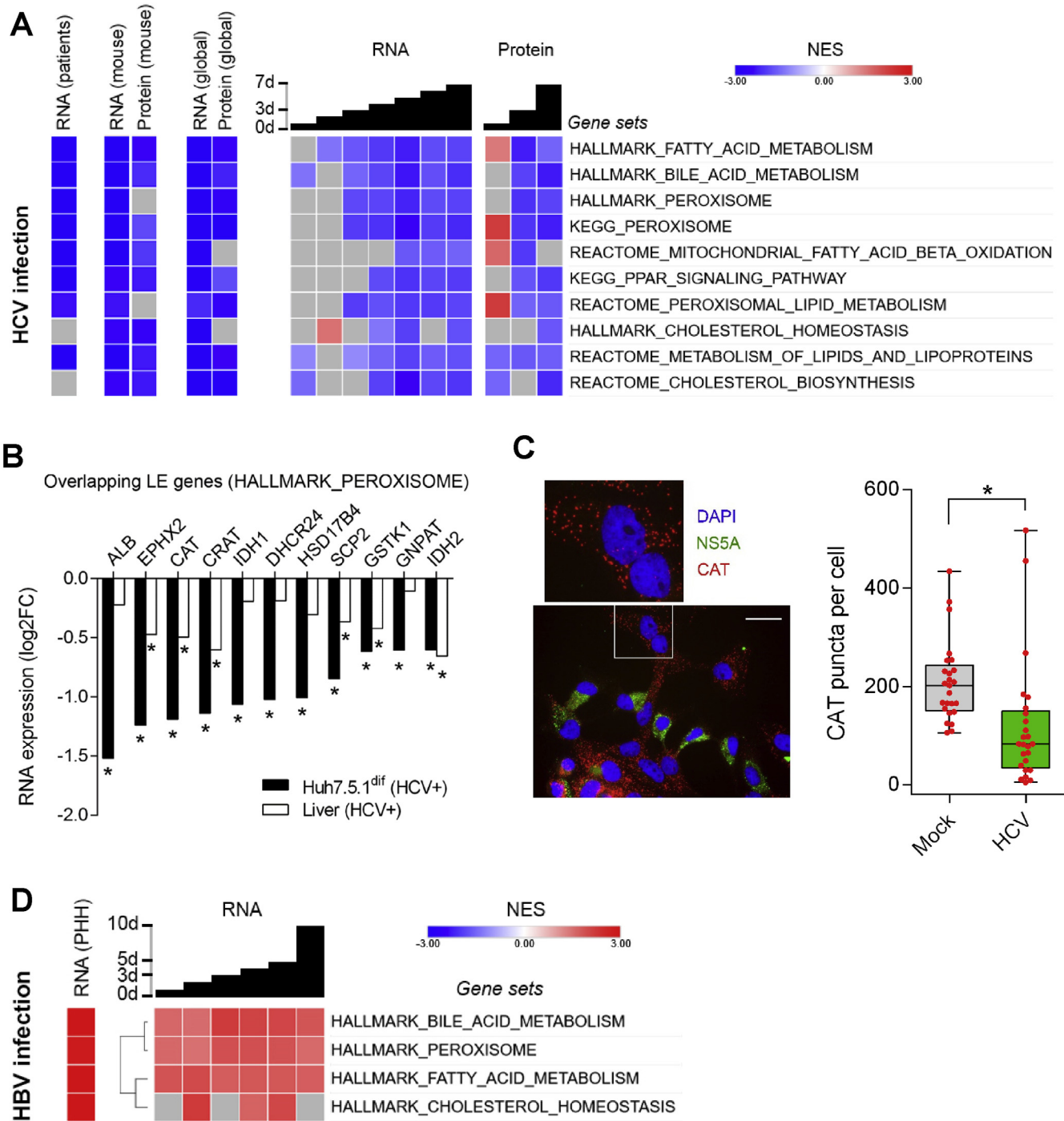
Figure 3. HCV, but not HBV, infection impairs expression of peroxisomal genes in Huh7.5.1 dif cells and liver tissue of patients. (A) HCV infection impairs metabolic pathways associated with peroxisomal function and lipid homeostasis. GSEA of RNA-seq data from liver tissue of 25 chronic HCV-infected patients to 6 noninfected individuals 26 and transcriptomics and proteomics of HCV-infection time course of Huh7.5.1 dif relative to mock-infected cells (n = 2). (B) Expression of 11 peroxisomal genes is significantly (P < .05, Wald test) suppressed by HCV in Huh7.5.1 dif and in the liver tissue of patients with chronic HCV infection. 26 Log fold change of leading-edge gene expression of the HALLMARK_PEROXISOME gene set in A. (C) Peroxisome marker expression is significantly (P = .0048, t test) perturbed in HCV-infected hepatocyte-like cells. Immunofluorescence microscopy of Huh7.5.1 dif cells infected for 3 days with HCVcc. The peroxisomal marker catalase (CAT) is stained in red, nuclear DNA (DAPI) in blue, and HCV (NS5A) in green (see also Supplementary Figure 5 ). Quantification of catalase-stained peroxisomes in 25 random HCV-infected cells and 25 mock cells is shown in the boxes/whiskers; scale bar represents 200 μm. (D) HBV infection promotes peroxisome function. GSEA of transcriptomics of HBV-infection of HepG2-NTCP for 10 days (n = 3) and primary human hepatocytes (n = 3) infected for 40 days with HBV (genotype D) (GSE69590). NESs are displayed in red (increased), blue (decreased), and gray (no significant change). Temporal analysis of infected Huh7.5.1 dif are presented as global trend (global) and individual time points. The statistical cutoff for GSEA of liver tissues was a false discovery rate of Q < .05 and for Huh7.5.1 dif was P < .005. FC, fold change; NES, normalized enrichment score; * significant, as stated in the respective panel legends.
