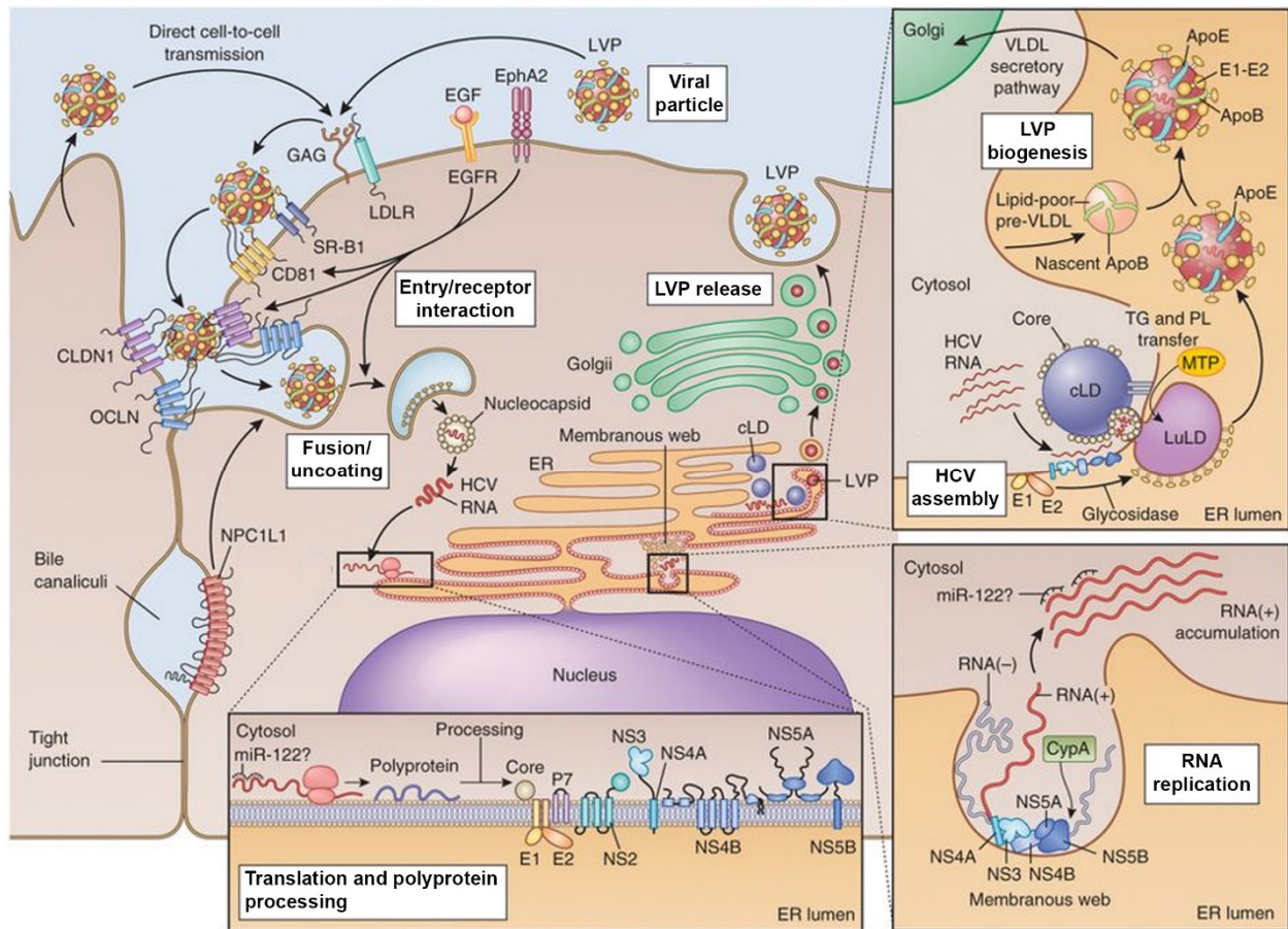
Figure 3: The HCV life cycle. Model of the different stages required for the HCV viral cycle including entry, fusion, translation, genome replication, HCV assembly and LVP release (Image modified from Scheel and Rice 2013).
