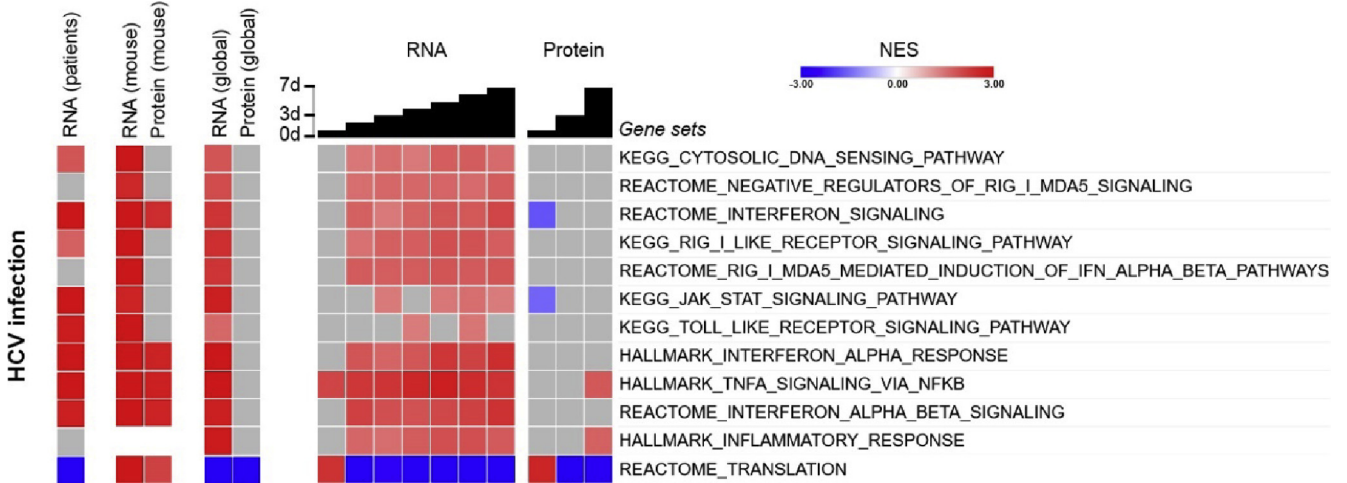
Supplementary Figure 3. Persistent HCV infection triggers an attenuated innate immune response. HCV-infected Huh7.5.1 dif cells relative to mock-infected cells until 7 days after infection. GSEA of proteomics and/or transcriptomics of livers of HCV-infected patients, human liver chimeric uPA/SCID mice, and Huh7.5.1 dif . HCV infection induces RNA expression of genes associated with innate immunity but suppresses their translation into proteins. NESs are displayed in red (increased), blue (decreased), gray (no significant change), and white (below analysis cutoff). Temporal analysis of infected Huh7.5.1 dif are presented as global trend (global) and individual time points. Statistical cutoff for GSEA of liver tissues was a false discovery rate of Q < .05 and for infected Huh7.5.1 dif ( P < .005 ).
