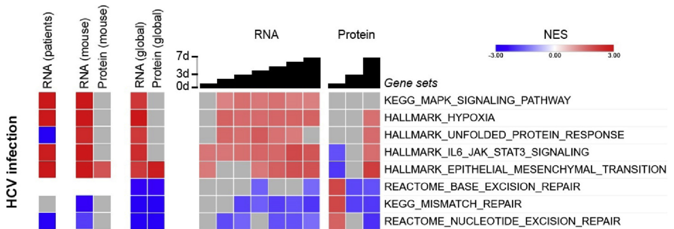
Supplementary Figure 6. Persistent HCV infection perturbs cell circuits driving liver disease and cancer. GSEA of transcriptomics and proteomics of HCV-infected Huh7.5.1 dif cells relative to mock-infected cells until 7 days after infection. HCV infection perturbs pathways that are known hallmarks of cancer development. NESs are displayed in red (increased), blue (decreased), gray (no significant change), and white (below analysis cutoff). Temporal analysis of infected Huh7.5.1 dif are presented as a global trend (global) and individual time points. Statistical cutoff for GSEA of liver tissues was a false discovery rate of Q < .05 and for infected Huh7.5.1 dif was of P < .005 .
