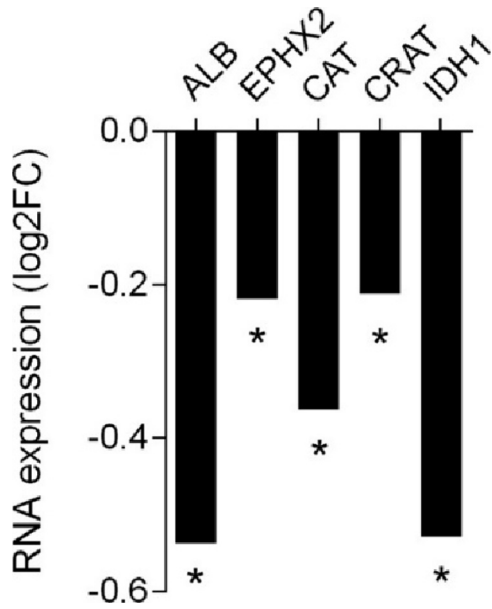
Supplementary Figure 4. Expression of leading-edge genes of the HALLMARK_PEROXISOME gene set are impaired by HCV infection. Validation of the top 5 genes (Huh7.5.1 dif , RNA-seq) shown in Figure 3B using quantitative PCR. Data are displayed as log2FC RNA expression in HCV-infected Huh7.5.1 dif cells. GAPDH expression was used as the housekeeping gene. * P < .05, 1-tailed t test ( n = 3 in duplicate).
