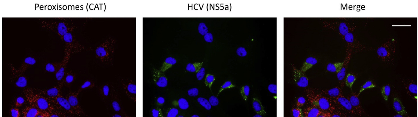
Supplementary Figure 5. Peroxisome marker expression is perturbed in HCV-infected hepatocyte-like cells. Immunofluorescence microscopy of Huh7.5.1 dif cells infected for 3 days with HCVcc. The peroxisomal marker catalase (CAT) is stained in red, nuclear DNA (DAPI) in blue, and HCV (NS5A) in green. Scale bar represents 200 \mu m.
