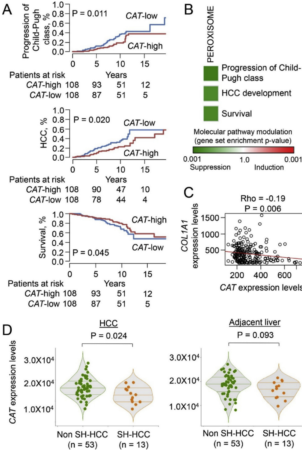
Supplementary Figure 8. Significant association of hepatic catalase expression with clinical outcomes and phenotypes in viral and metabolic liver disease. (A) Early-stage HCV cirrhosis patients (N = 216) 20 are classified into 2 groups, CAT-high and CAT-low groups, based on median expression level. Association of the grouping with overall survival (bottom), HCC development (middle), and progression of Child-Pugh class 21 from A to B or C (top). Patients with lower CAT expression levels show worse clinical outcomes (log-rank test). (B) Association of peroxisome pathway modulation with the clinical outcomes in the 216 HCV cirrhosis patients determined by GSEA. (C) CAT expression levels were negatively correlated (Spearman correlation test) with hepatic COL1A1 expression levels in the 216 HCV cirrhosis patients. (D) Distribution and probability density of CAT expression in HCC tumor (left) and adjacent non-tumor liver tissues (right) in 66 HCC patients 22 according to presence of histologic steatohepatic HCC (SH-HCC) variant 23 (violin plot, Wilcoxon rank-sum test).
