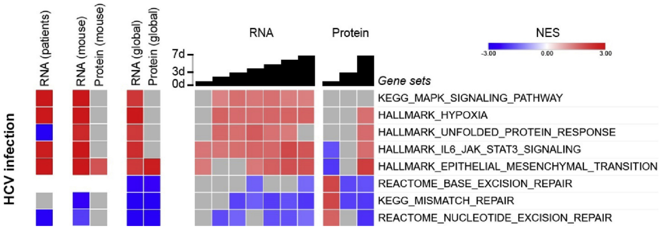
Supplementary Figure 6. Persistent HCV infection perturbs cell circuits driving liver disease and cancer. GSEA of transcriptomics and proteomics of HCV-infected Huh7.5.1 dif cells relative to mock-infected cells until 7 days after infection. HCV infection perturbs pathways that are known hallmarks of cancer development. NESs are displayed in red (increased), blue (decreased), gray (no significant change), and white (below analysis cutoff). Temporal analysis of infected Huh7.5.1 dif are presented as a global trend (global) and individual time points. Statistical cutoff for GSEA of liver tissues was a false discovery rate of Q < .05 and for infected Huh7.5.1 dif was of P < .005 .
